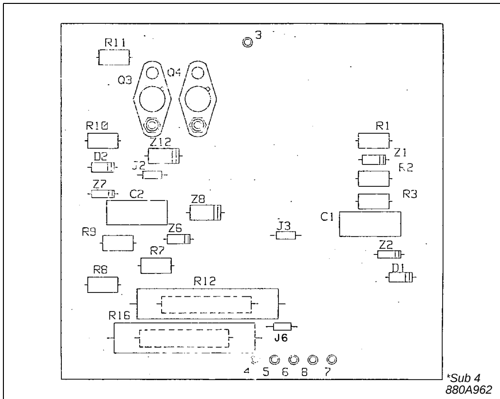
Figure 13. Component Location 2 Buffered Input "OR" in FT-22 Case; 48 Vdc.
