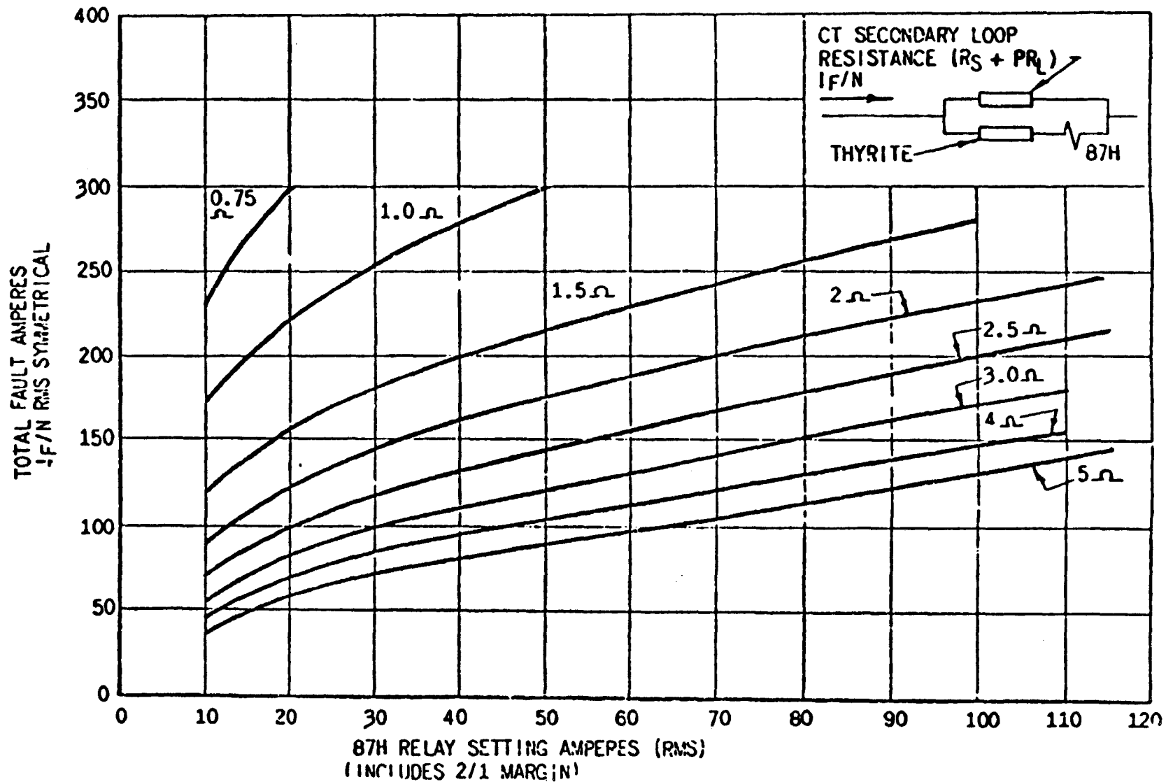
FIG. 10 (0246A3797-0) Curves Used for Obtaining 87H Unit Setting 2(R_s + P R_L) I_f / N Exceeds 350 Volts
