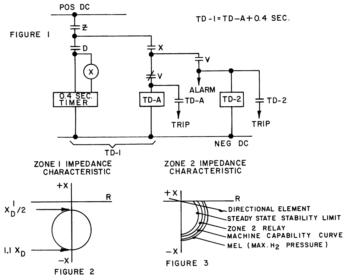
Figure 10. Generalized External Schematic
