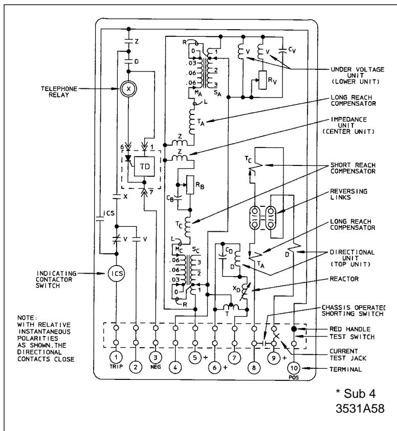
Figure 3. Internal Schematic of Type KLF Relay in FT-41 Case
