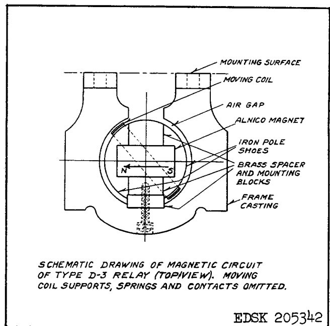
Fig. 3. Magnetic Circuit of d'Arsonval Type dc Contact Making Milliammeter.
