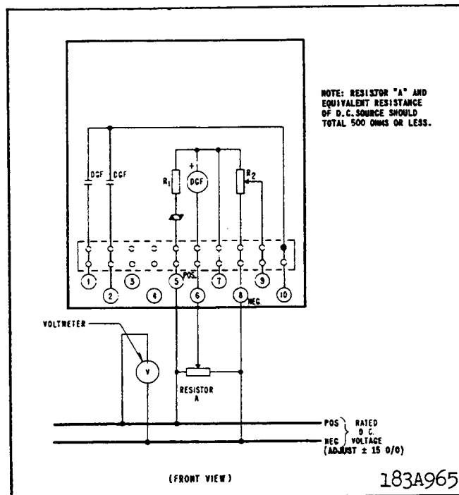
Fig. 8. Test Circuit of the Type DGF Relay.
