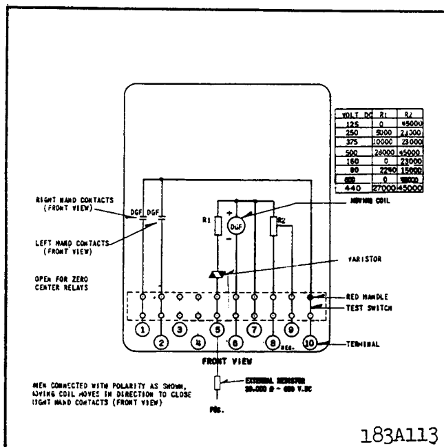
Fig. 2. Internal Schematic of the Type DGF Relay in the FT21 Case.
