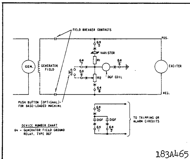
Fig. 4. External Schematic of the Type DGF Relay.
