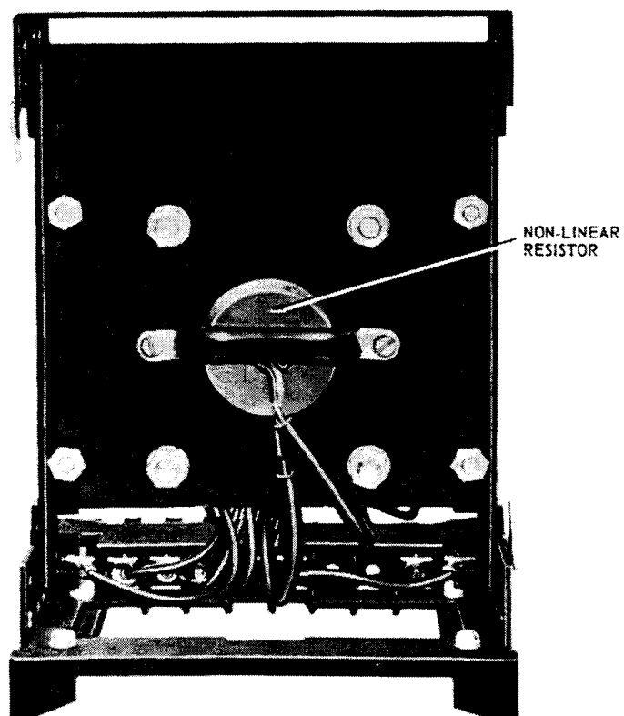
Fig. 1. Type DGF Relay without Case.
