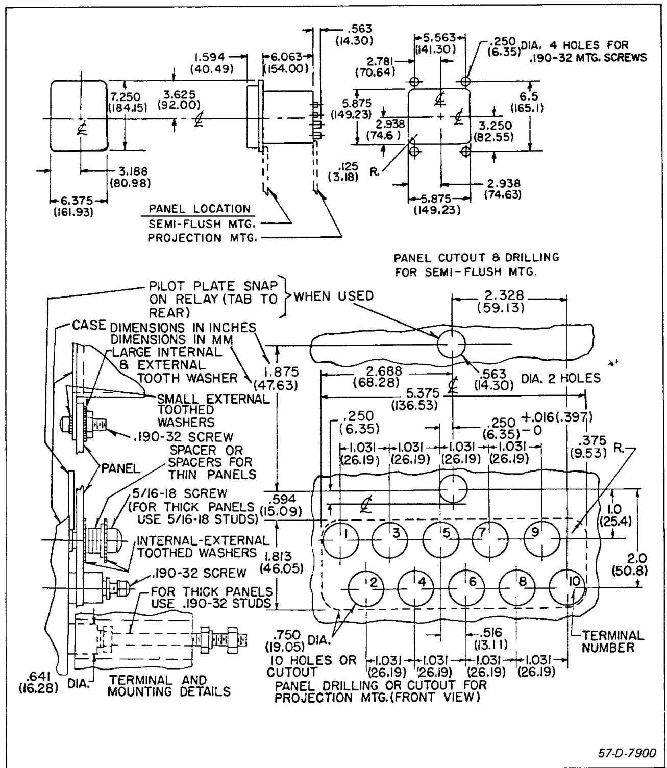
Fig. 12. Outline and Drilling Plan FT-11 Case
