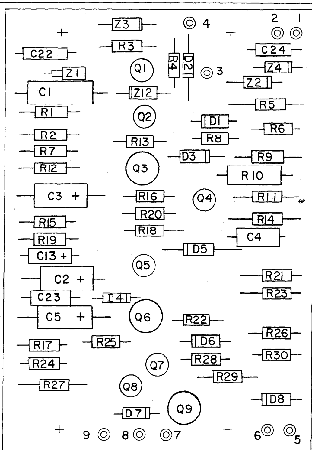
Fig. 9. Component Location of Reset Printed Circuit Board for Type SGR-52 Relay
