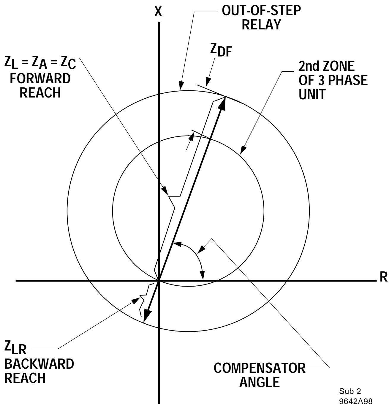
Figure 4. Relay Characteristic on R-X Diagram
