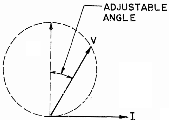
Figure 5. Compensator Construction
