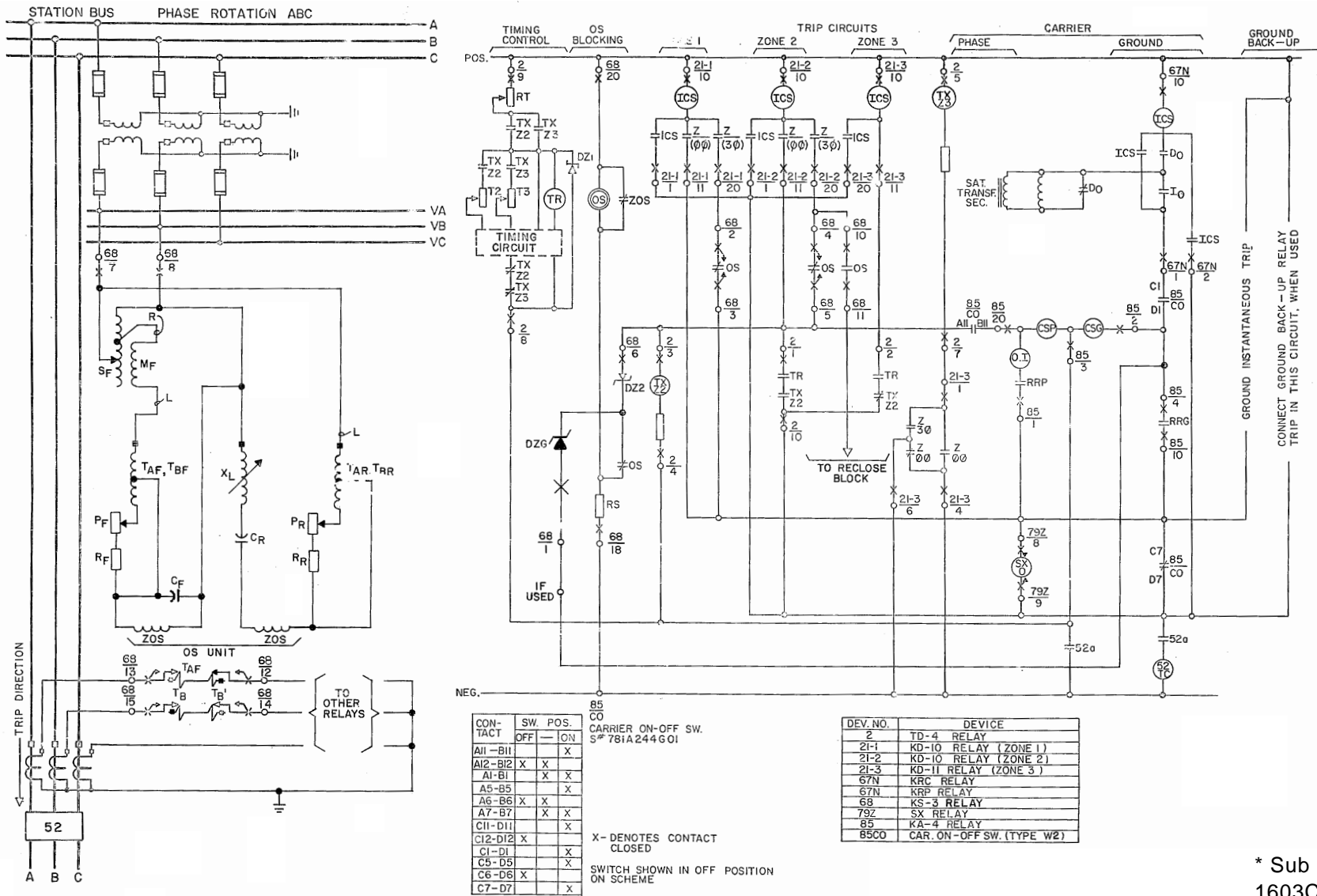
Figure 2. External Connections of KS-3 Relay
