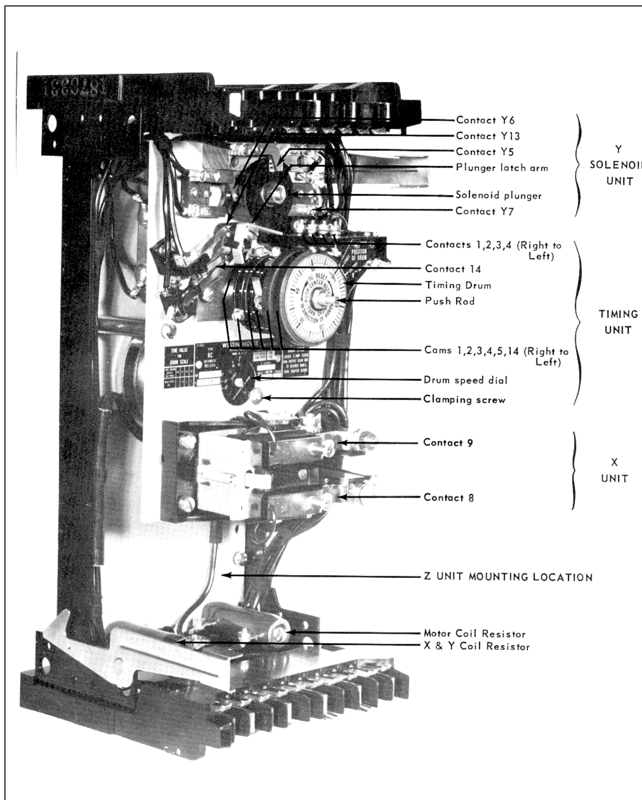
Figure 1. Type RC Relay, without Z Unit, without Case
