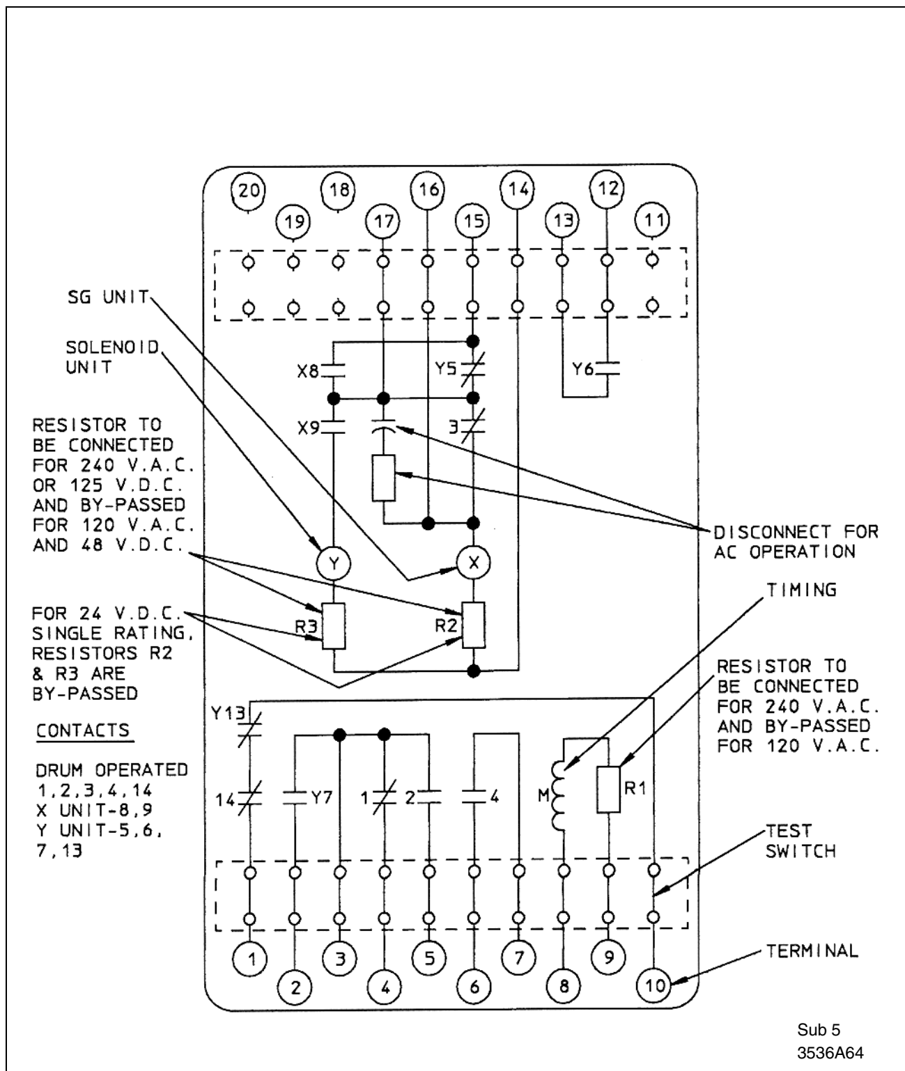
Figure 2. Internal Schematic of the RC Relay, without Z Unit, in Type FT-32 Case
