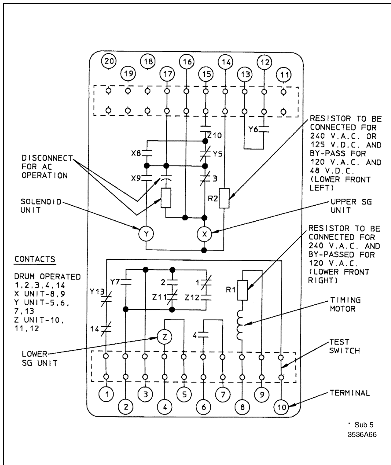
Figure 3. Internal Schematic of the RC Relay, with Z Unit, in Type FT-32 Case
