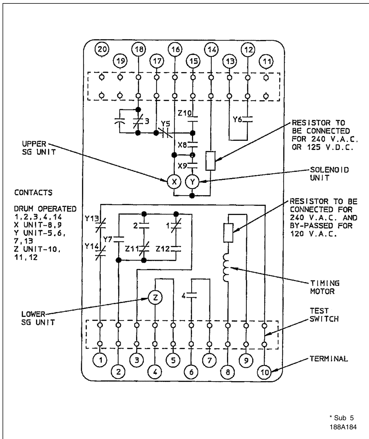
Figure 11. Internal Schematic of the RC Relay, with Z Unit, and #3 Contact Connected in Terminals, in Type FT-32 Case
