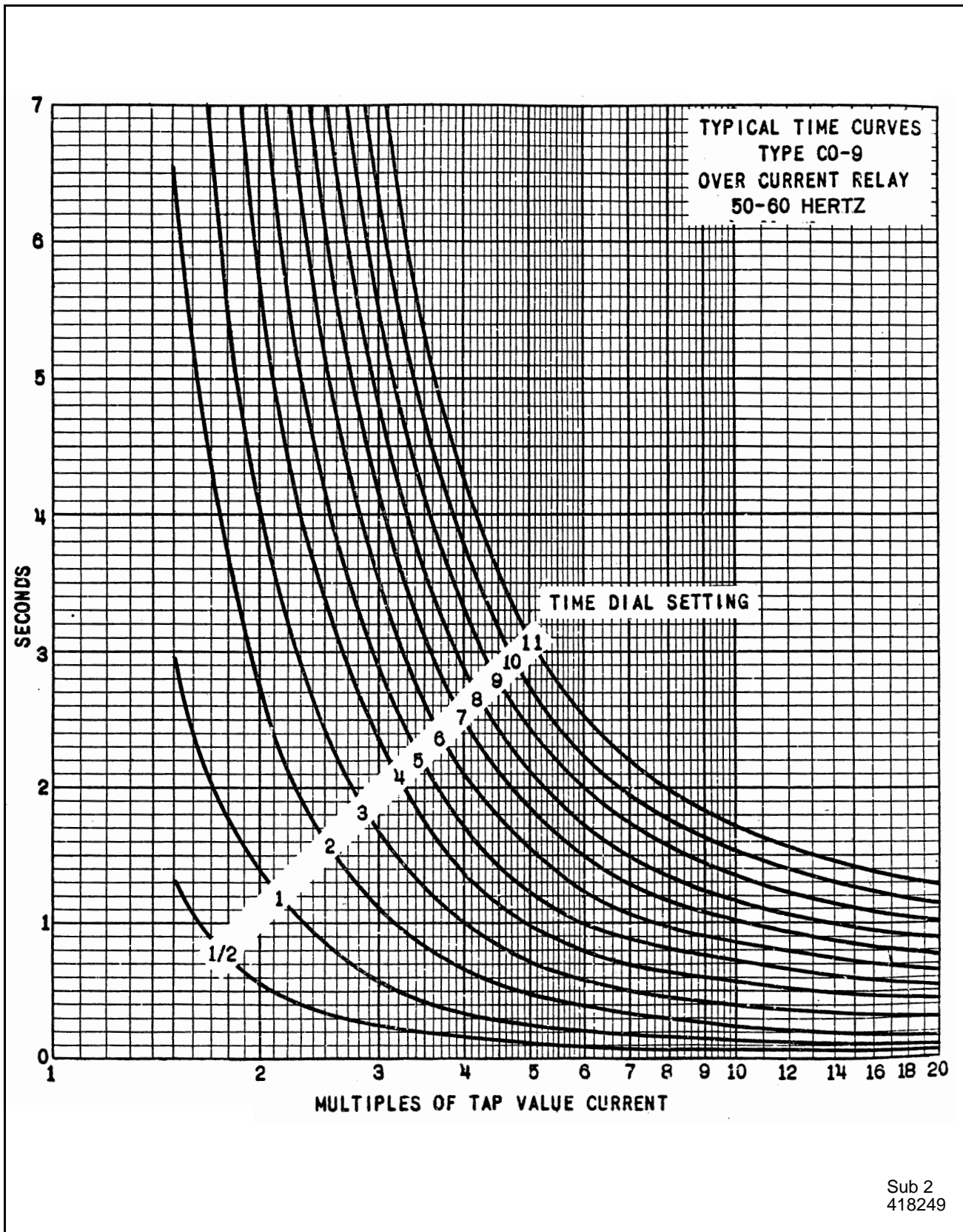
Figure 7: Typical 50 and 60 Hz Time Curves of COV-9 Overcurrent Unit
