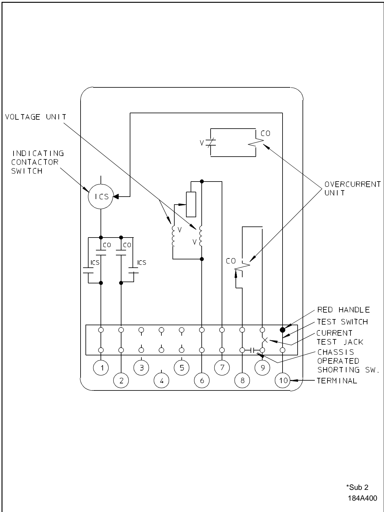
Figure 12: Relay Types COV-6, COV-7, COV-8, COV-9 Voltage Controlled Overcurrent Relay, Double Trip, In TypeFT-21 Case
