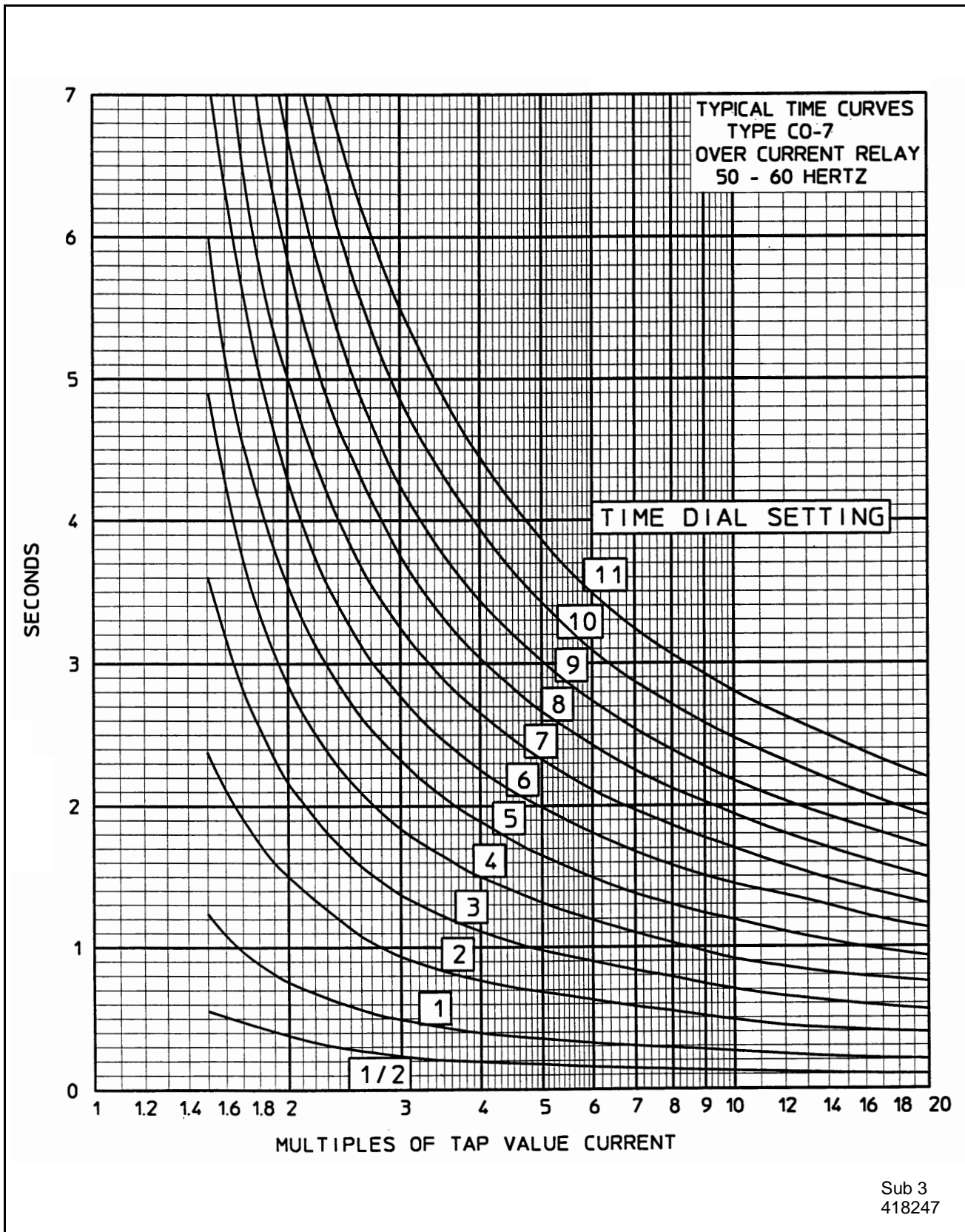
Figure 5: Typical 50 and 60 Hz Time Curves of COV-7 Overcurrent Unit
