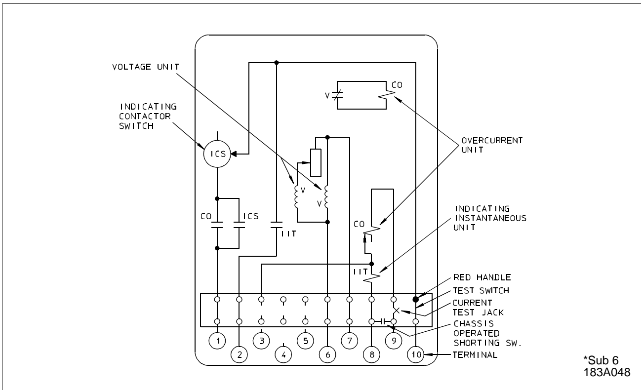
Figure 2: Internal Schematic of the COV Relay with the Indicating Instantaneous Trip Unit in the Type FT-21 Case
