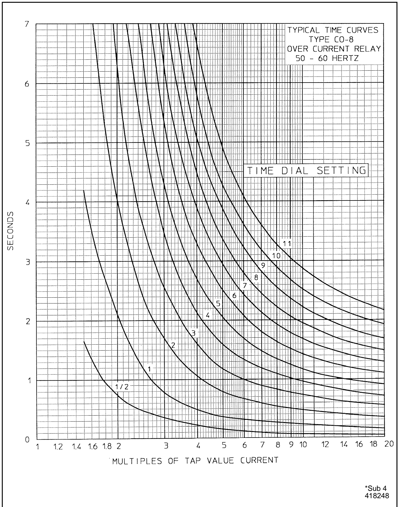
Figure 6: Typical 50 and 60 Hz Time Curves of COV-8 Overcurrent Unit
