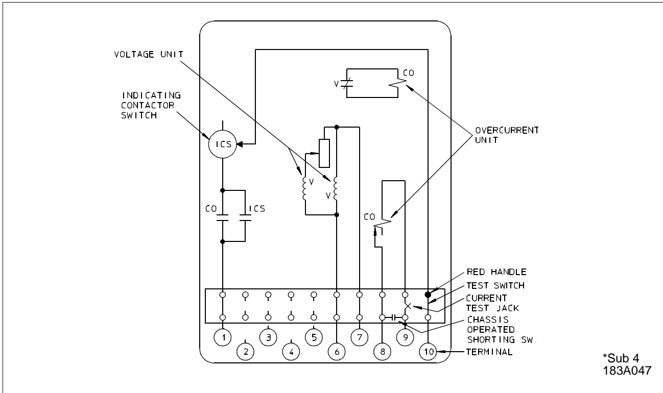
Figure 1: Internal Schematic of the COV Relay in the Type FT-21 Case
