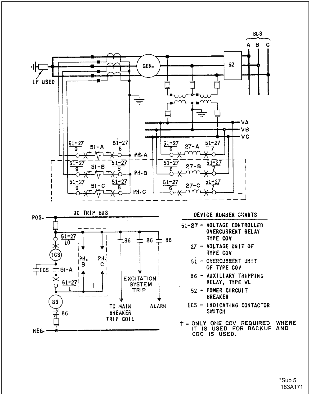
Figure 10: External Schematic of the Type COV Relay on a Generator
