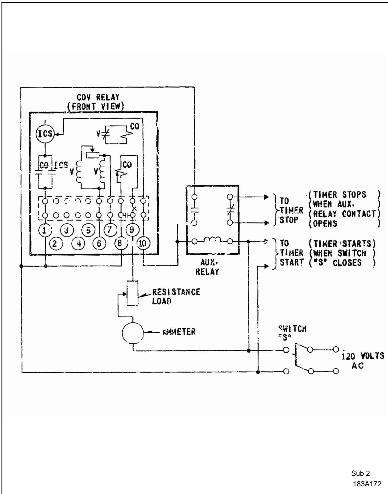
Figure 9: Diagram of Test Connections of the Overcurrent Unit
