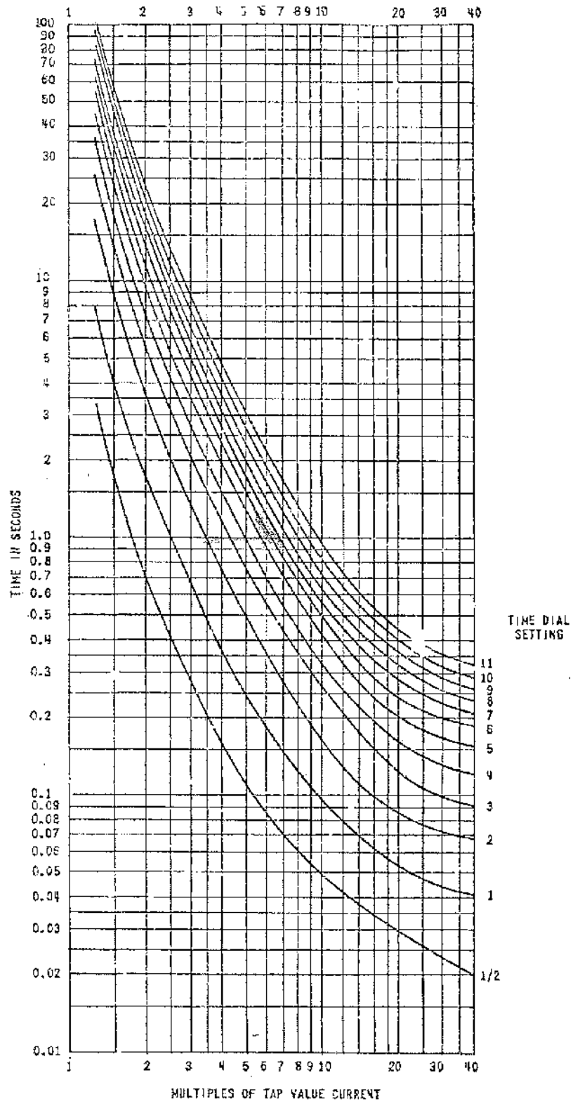
Figure 8: Typical Time Curves of COV-11 Overcurrent Unit, 50-60 Hertz
