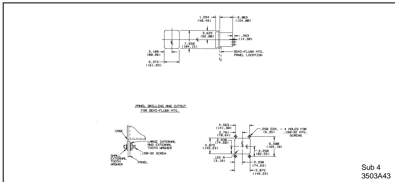
Figure 17: Outline and Drilling for the Type CO Relay in Case Type FT-11 for Class 1E Application
