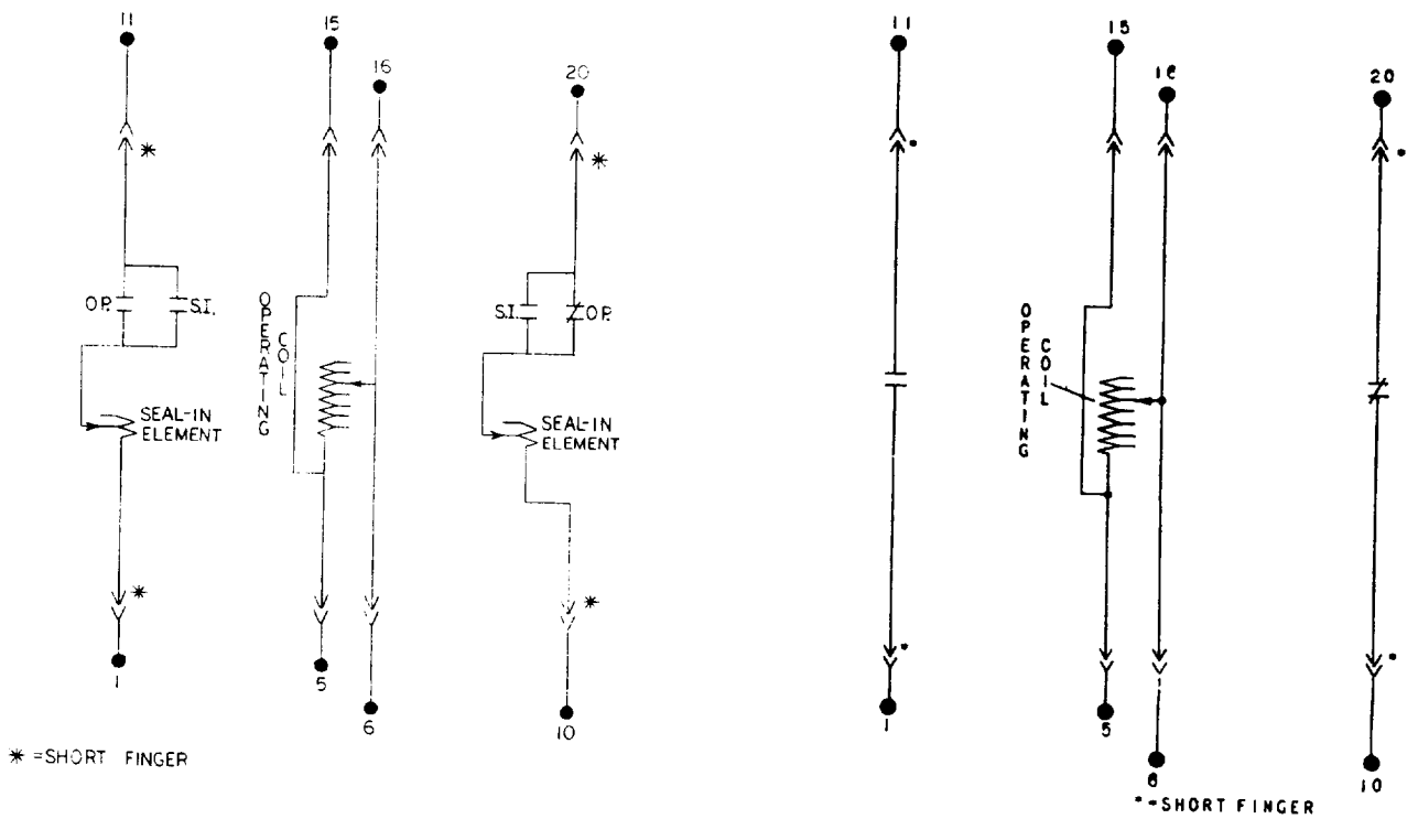
Figure 7 (K-6556475-1) Internal-Connection Diagram for Type-IAV53K Relay
