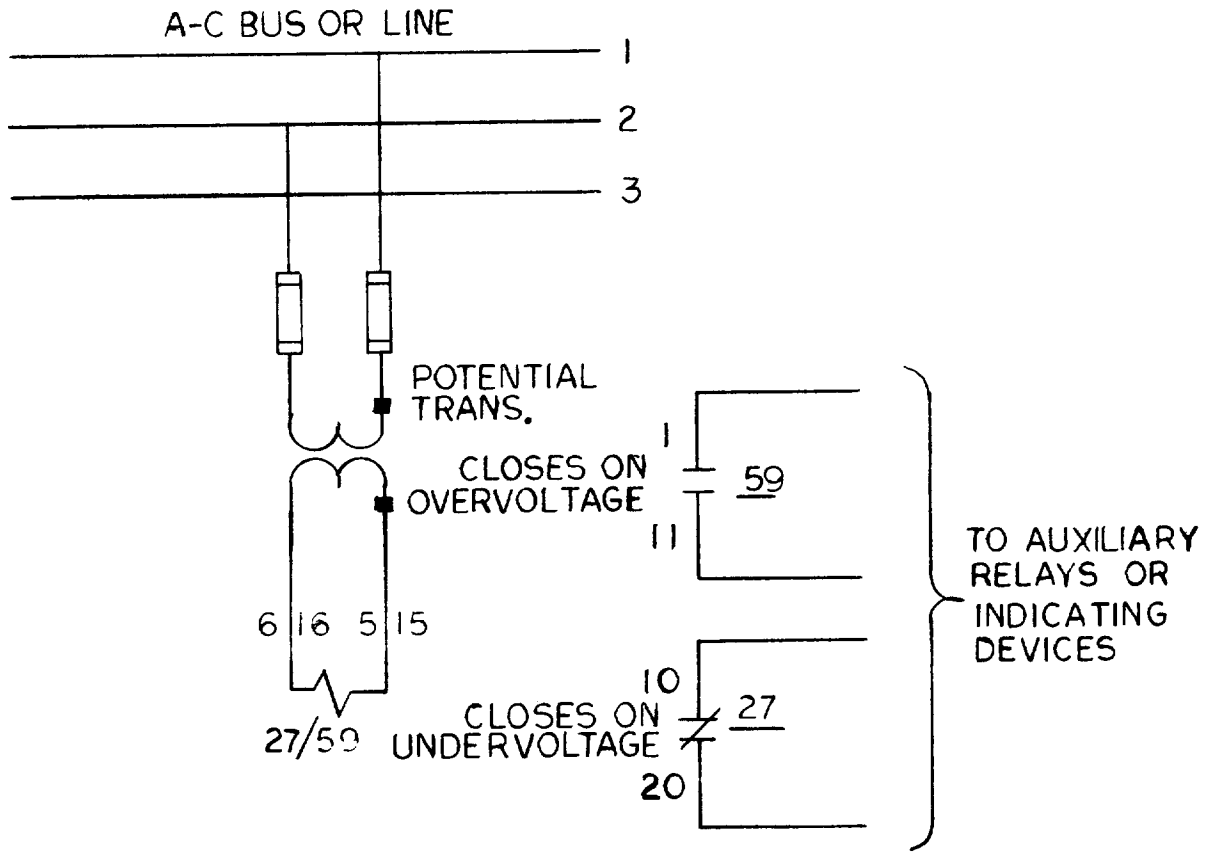
27/59 - UNDER AND OVERVOLTAGE RELAY TYPE IAV53K
