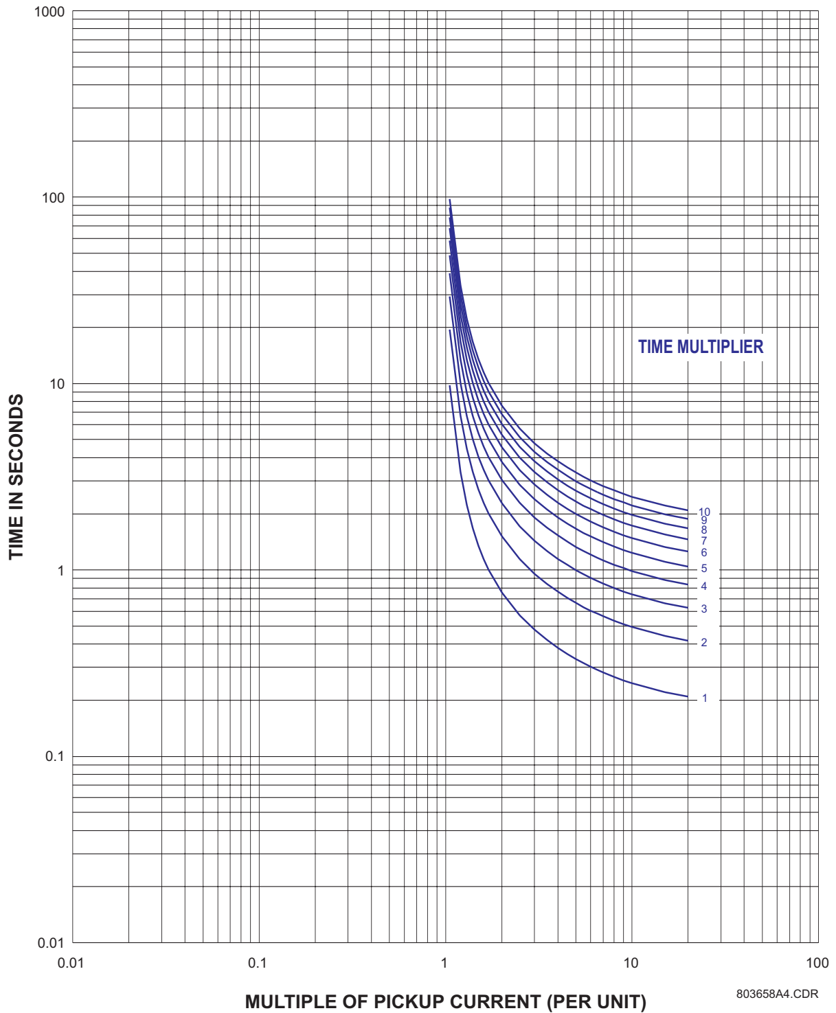
Figure 5–1: ANSI MODERATELY INVERSE CURVES
