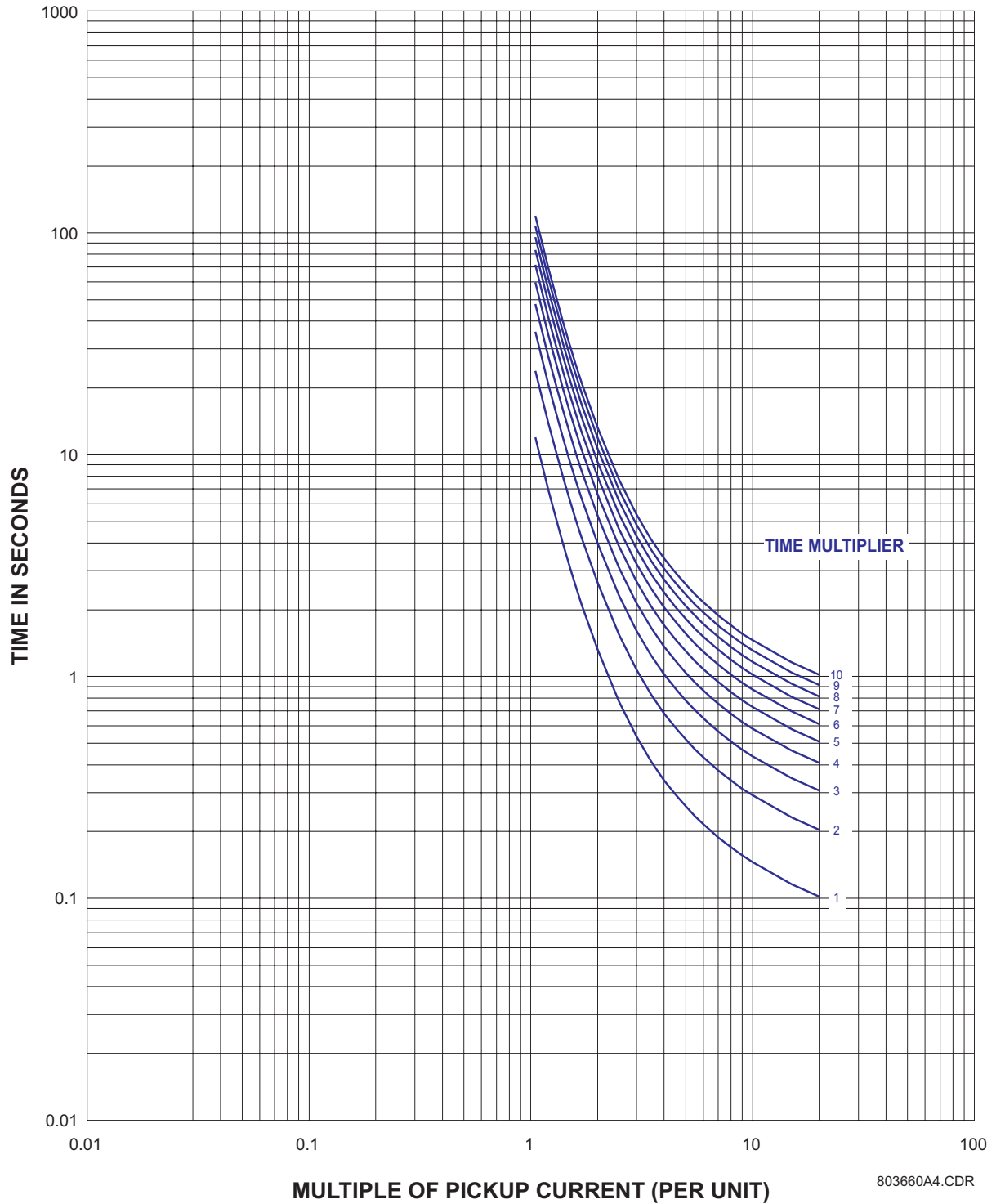
Figure 5-3: ANSI VERY INVERSE CURVES
