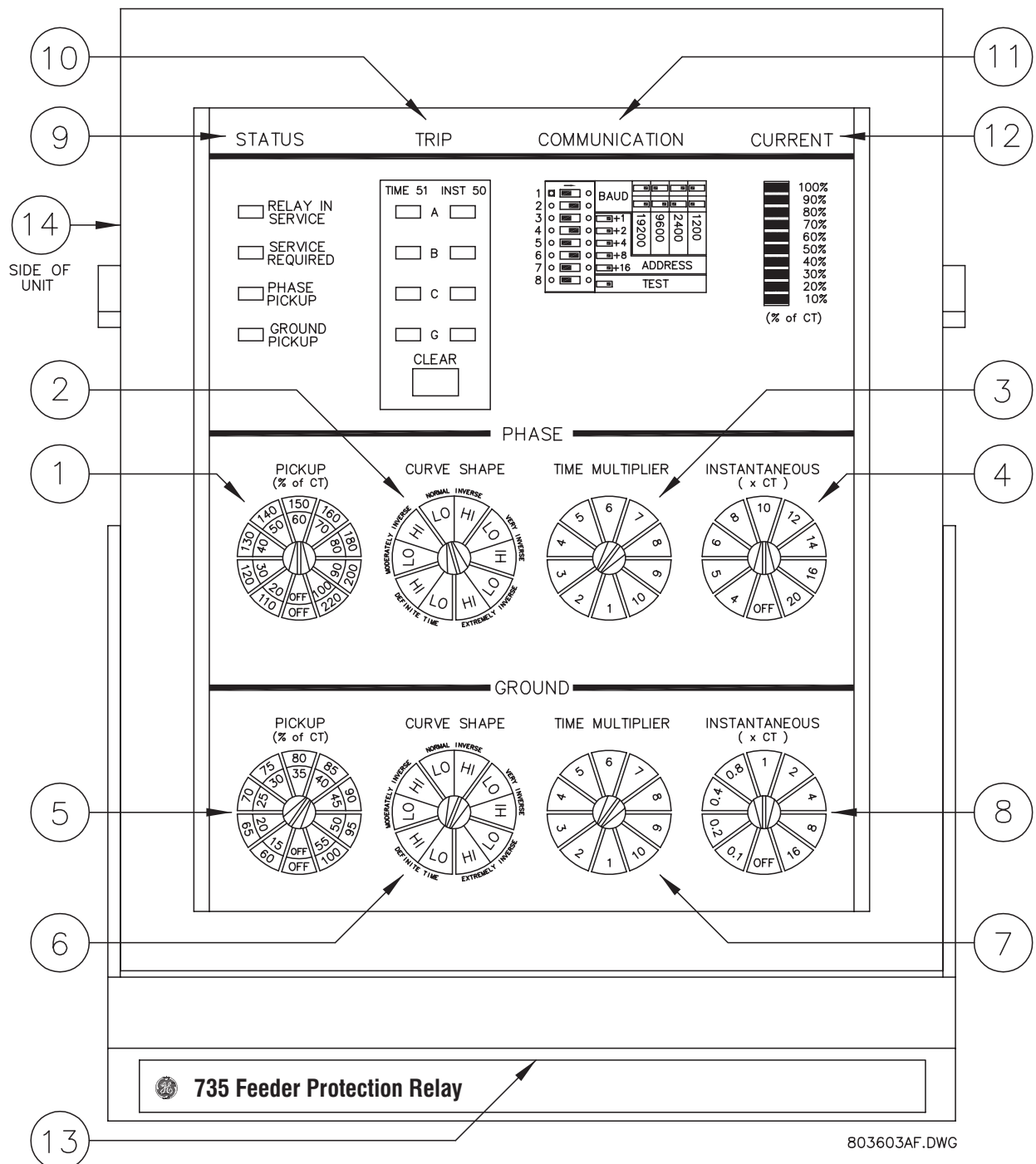
Figure 3-1: FRONT PANEL CONTROLS AND INDICATORS
