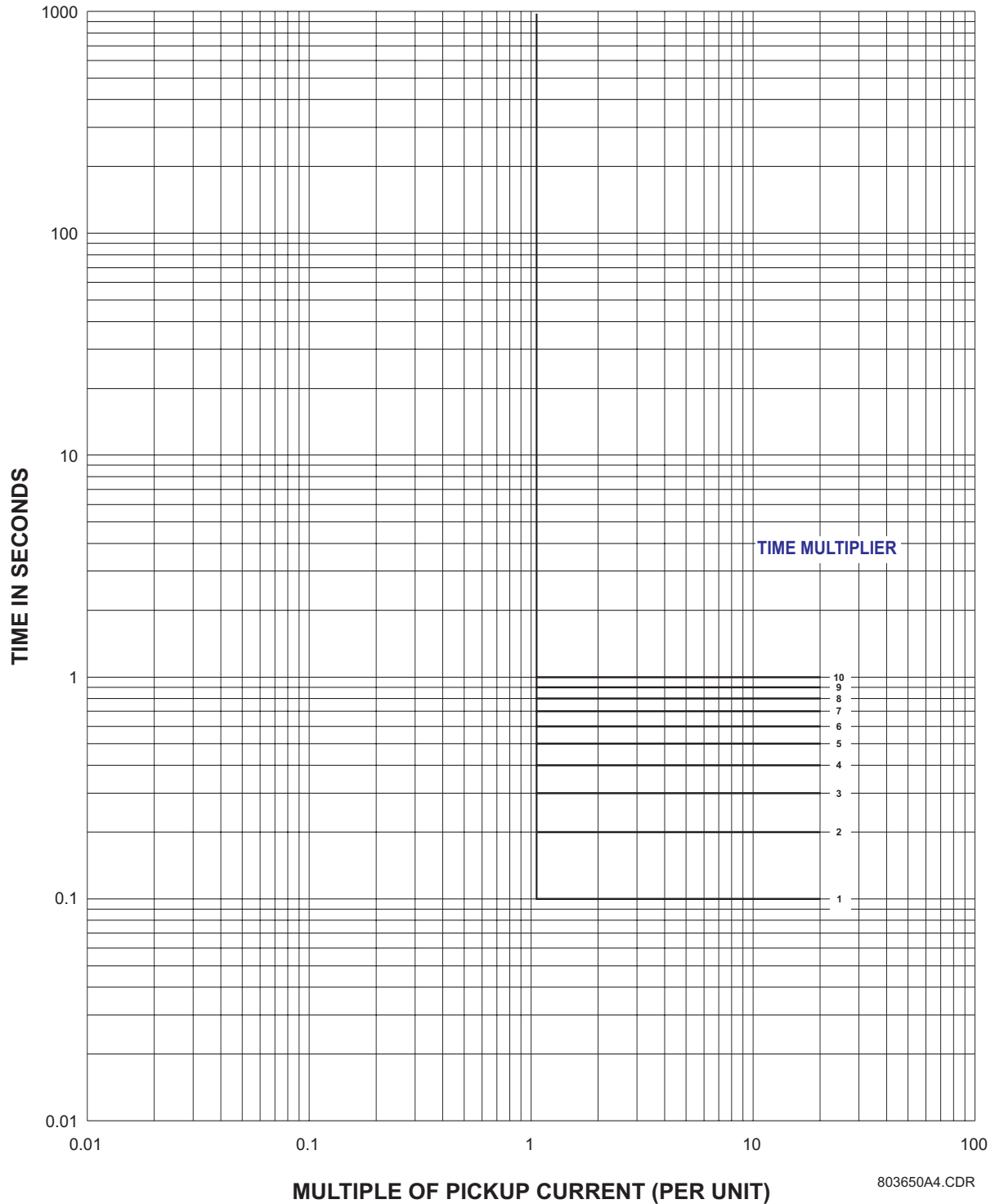
Figure 5–5: DEFINITE TIME CURVES
