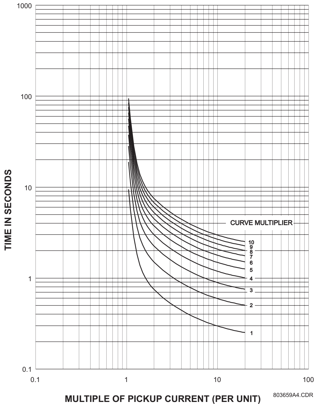
Figure 5-7: IAC INVERSE CURVES
