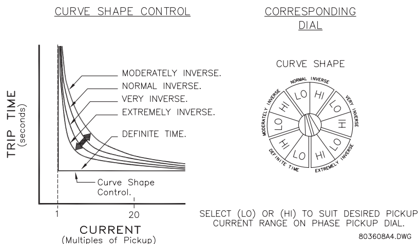
Figure 3-3: PHASE CURVE SHAPE SETTING
