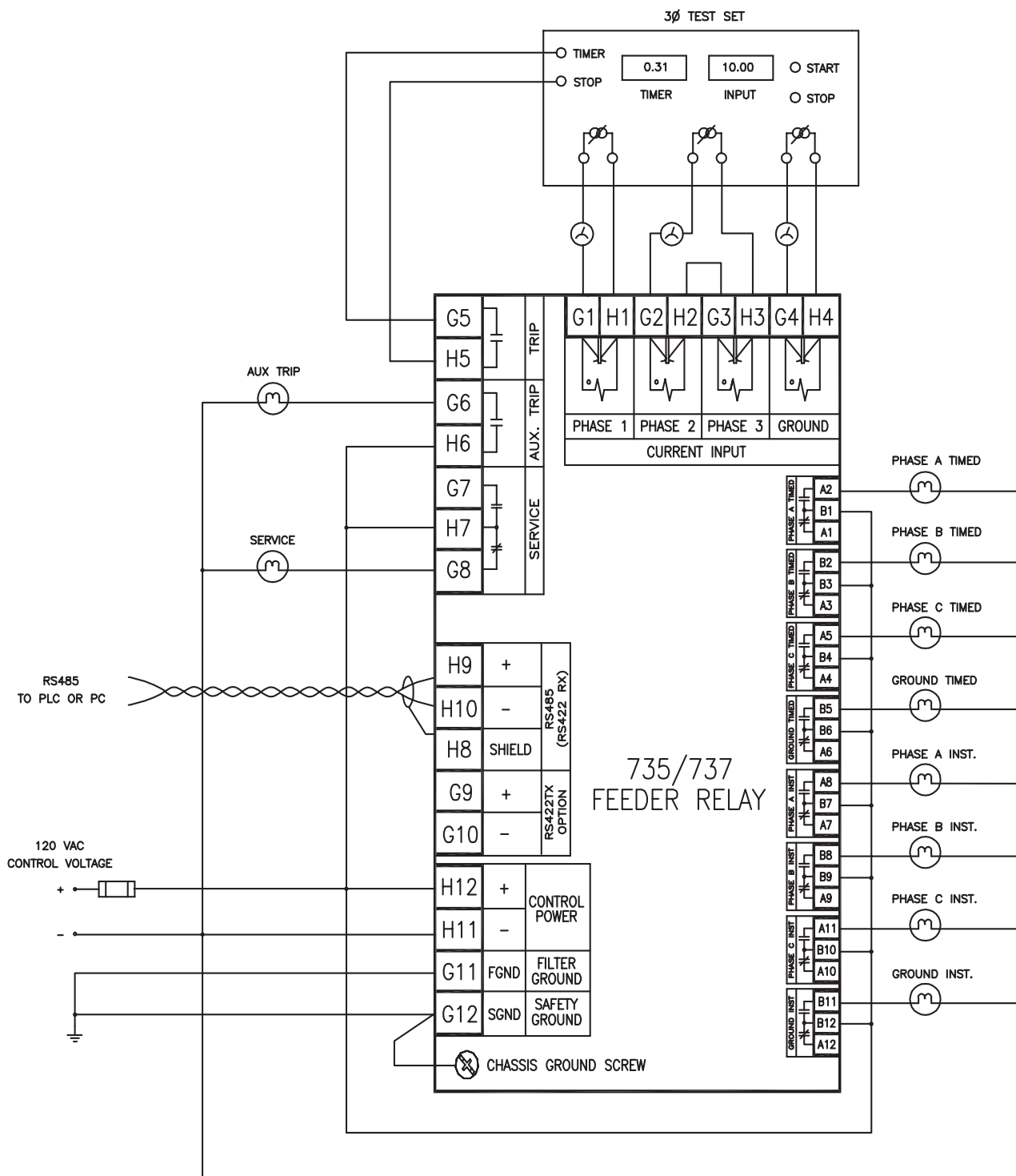
Figure 6-1: TEST SETUP
