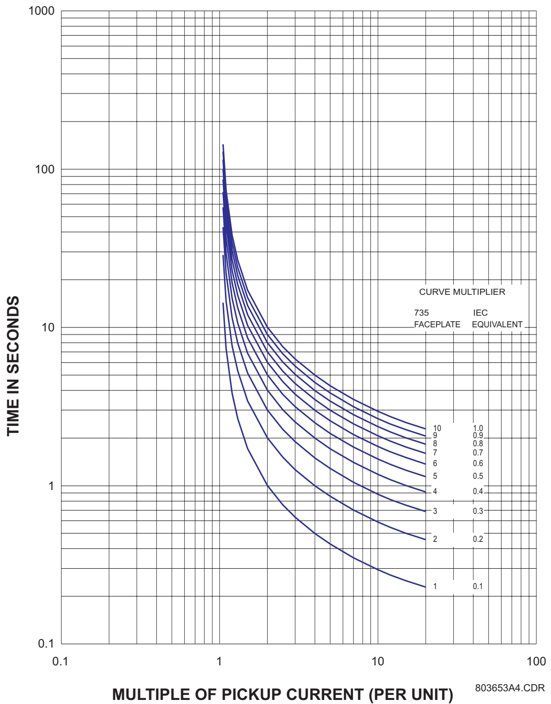
Figure 5-11: IEC A CURVES
