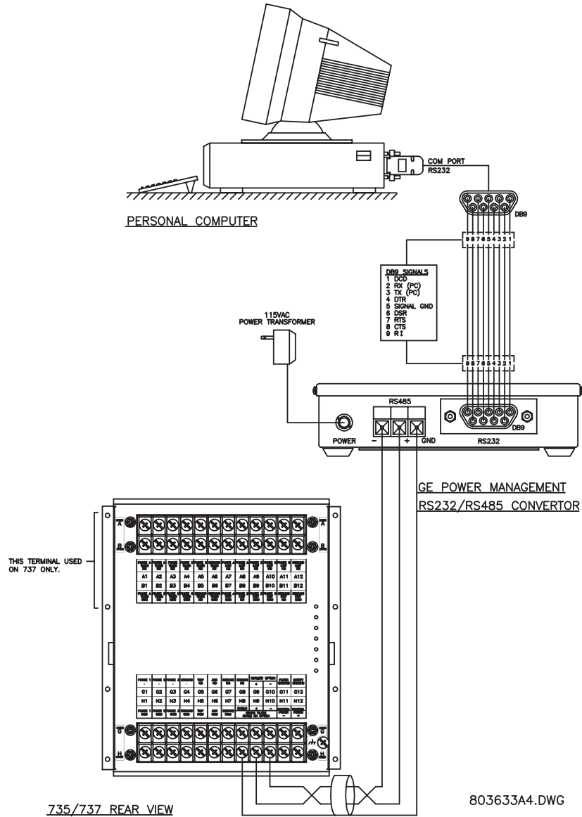
Figure 2-14: RS232/485 CONVERTER
