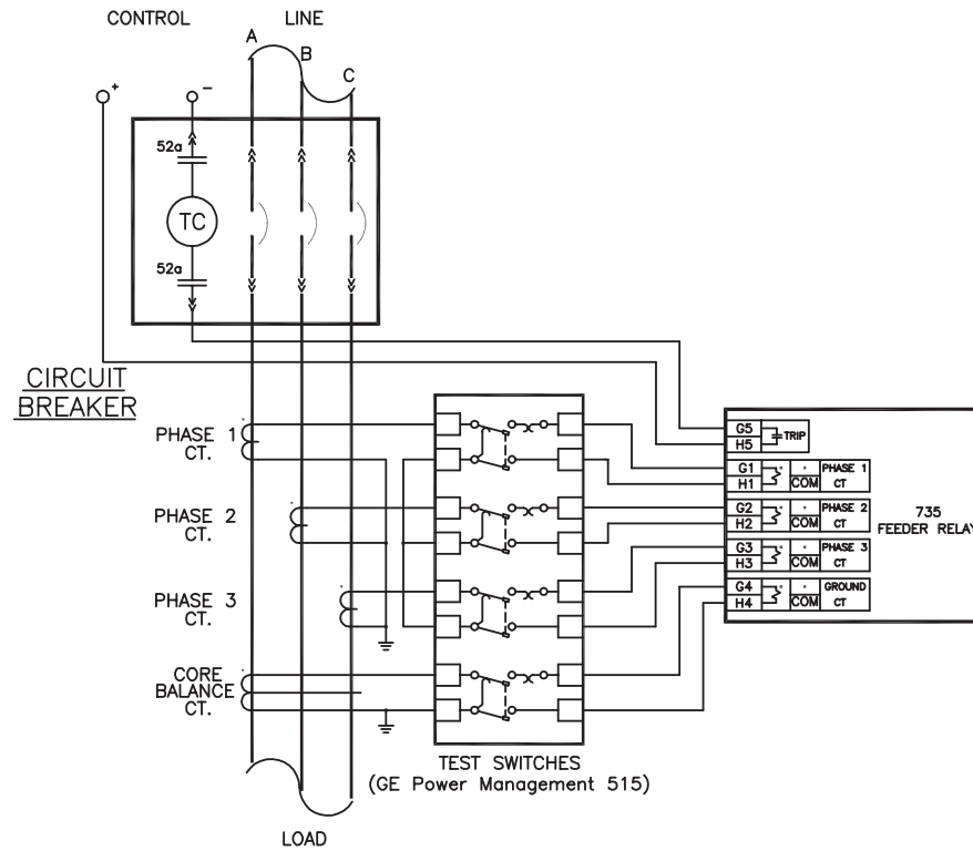
Figure 2-9: BACKUP WIRING – CORE BALANCE
