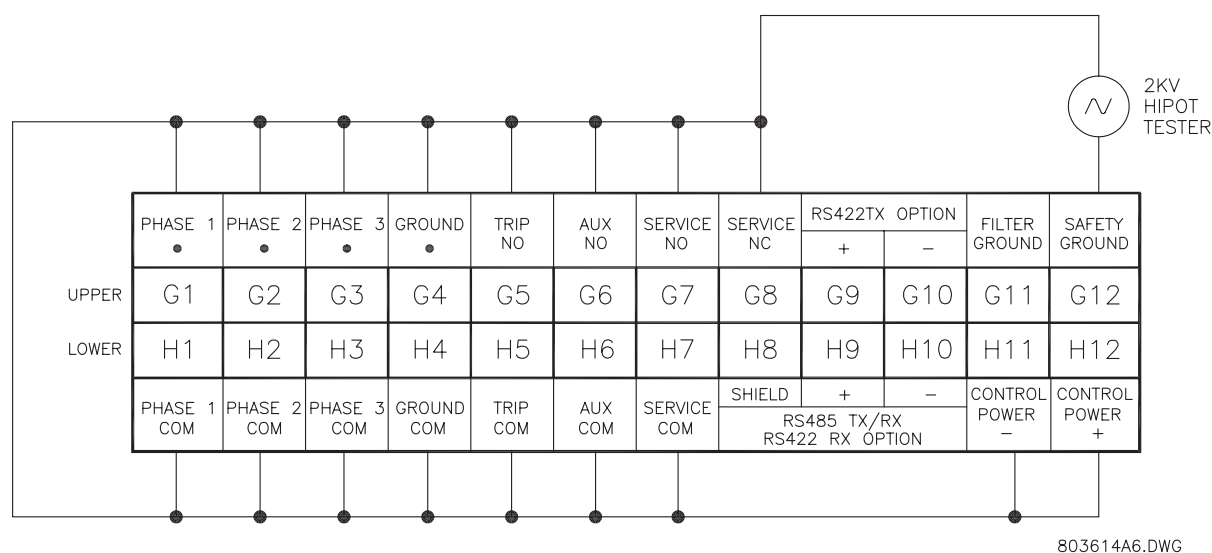
Figure 2–15: HI-POT TESTING CONNECTIONS
