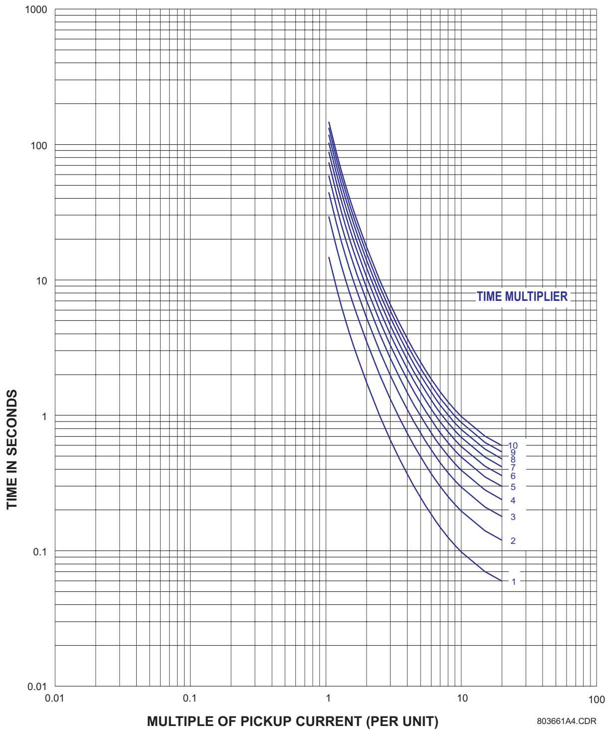
Figure 5-4: ANSI EXTREMELY INVERSE CURVES
