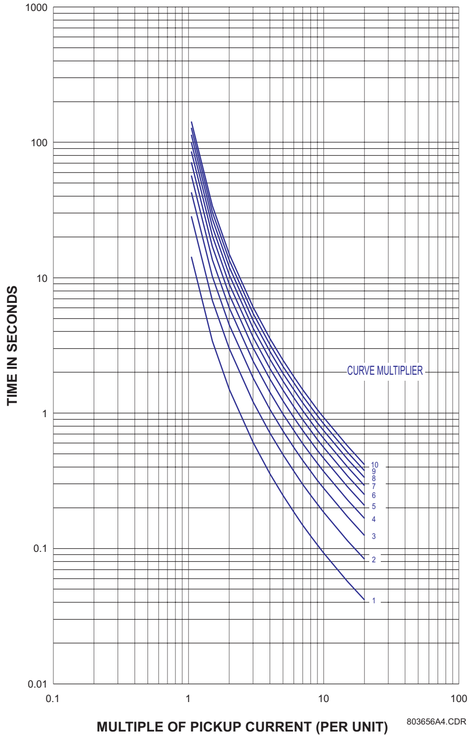
Figure 5–9: IAC EXTREMELY INVERSE CURVES
