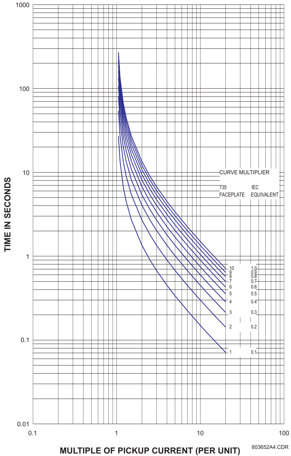
Figure 5-12: IEC B CURVES
