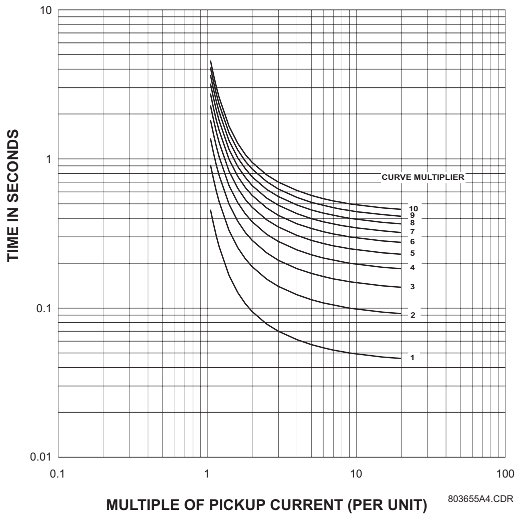
Figure 5–6: IAC SHORT INVERSE CURVES
