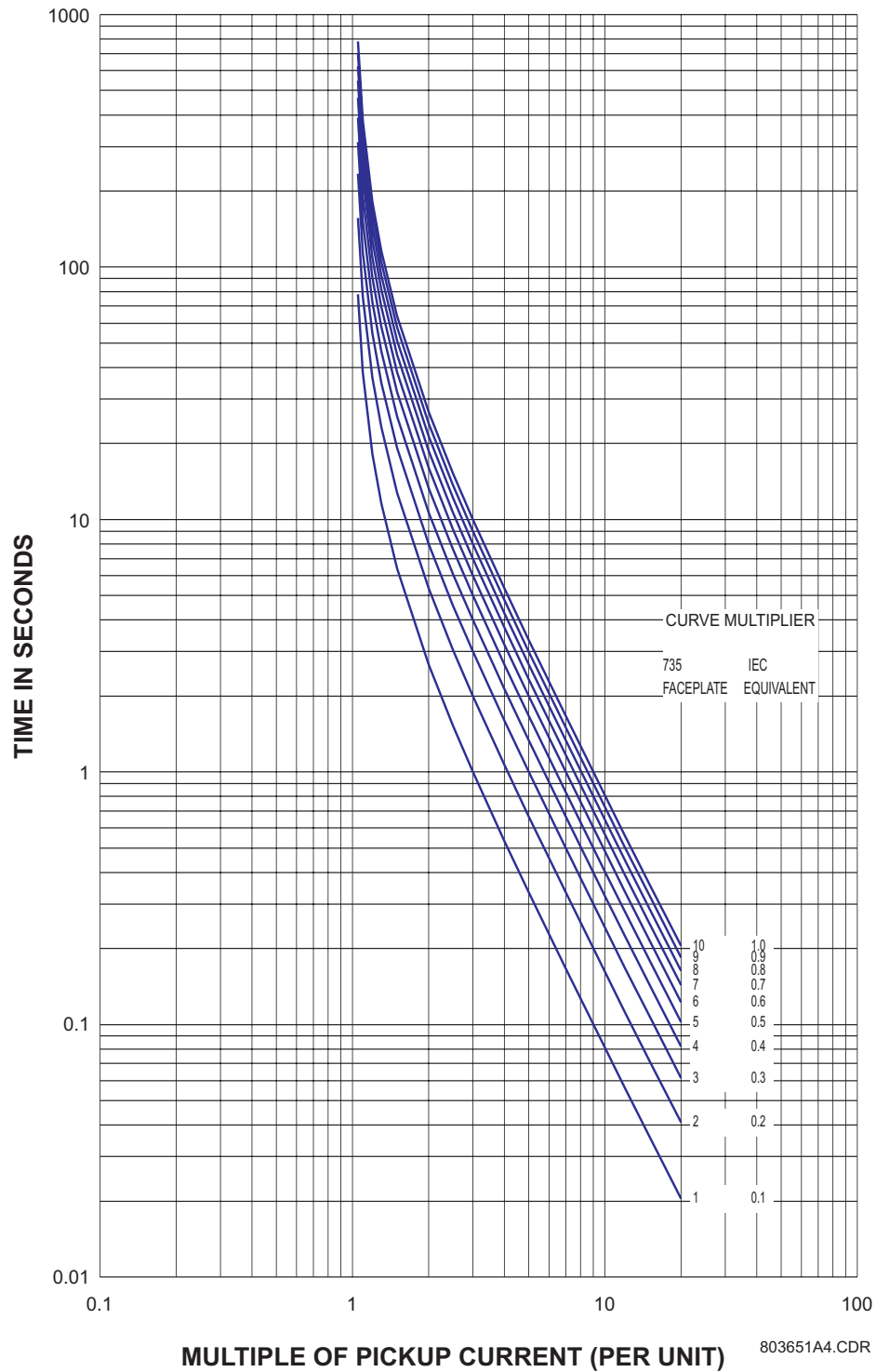
Figure 5-13: IEC C CURVES
