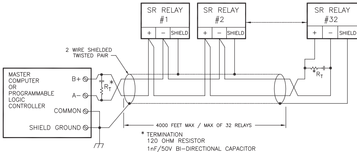
Figure 2-12: RS485 TERMINATION
