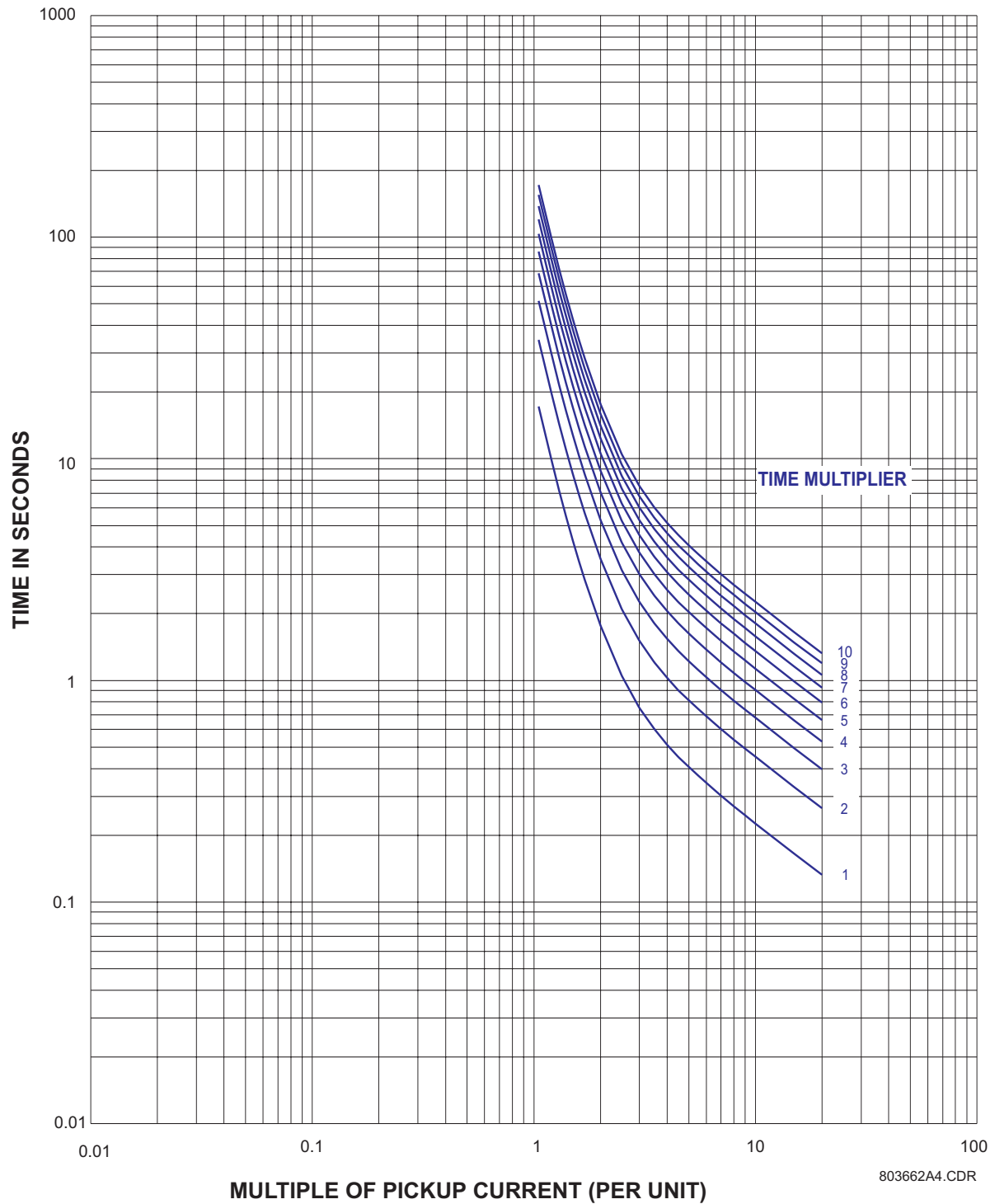
Figure 5-2: ANSI NORMAL INVERSE CURVES
