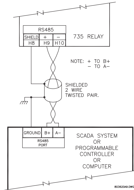
Figure 2-11: RS485 CONNECTION
