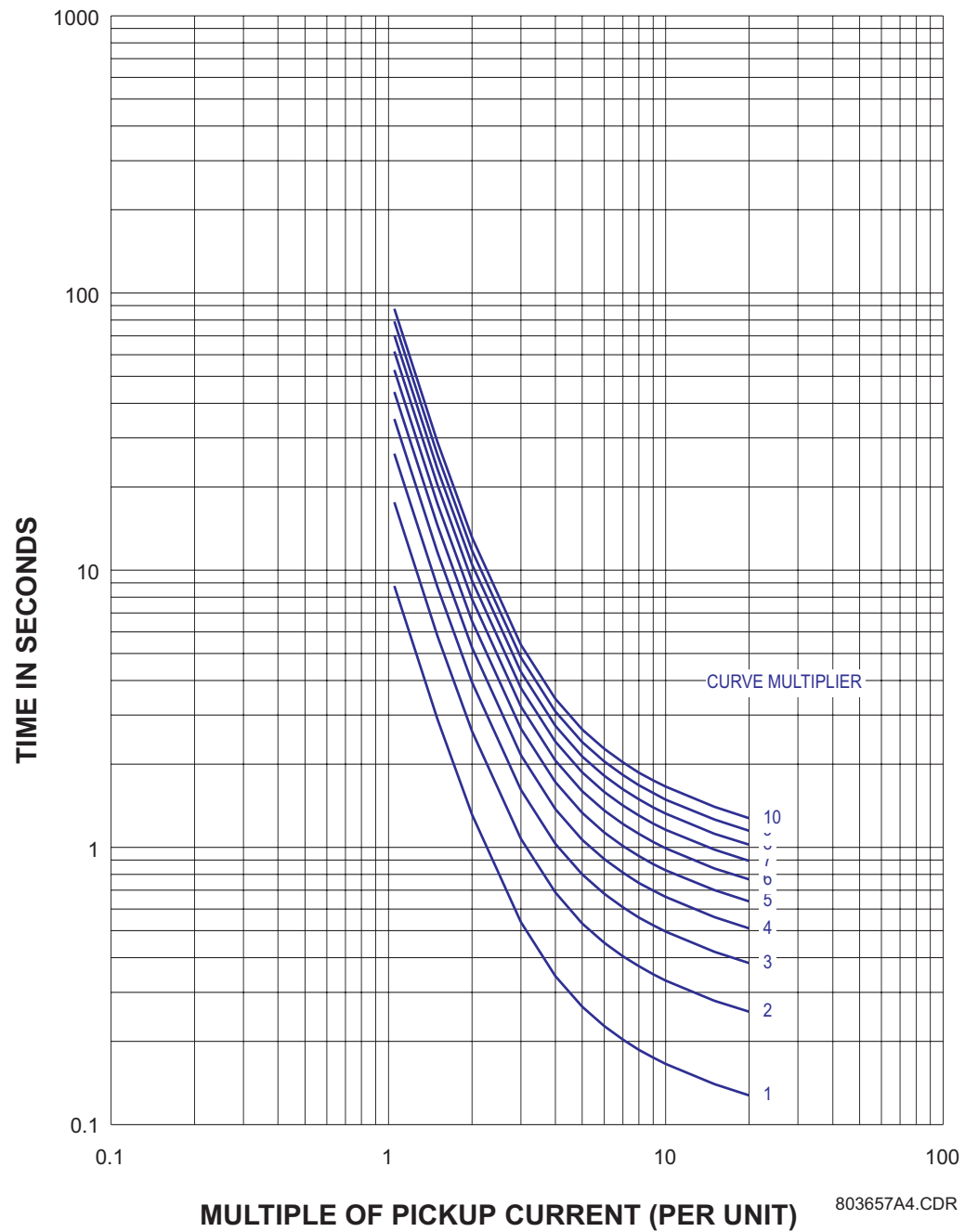
Figure 5–8: IAC VERY INVERSE CURVES
