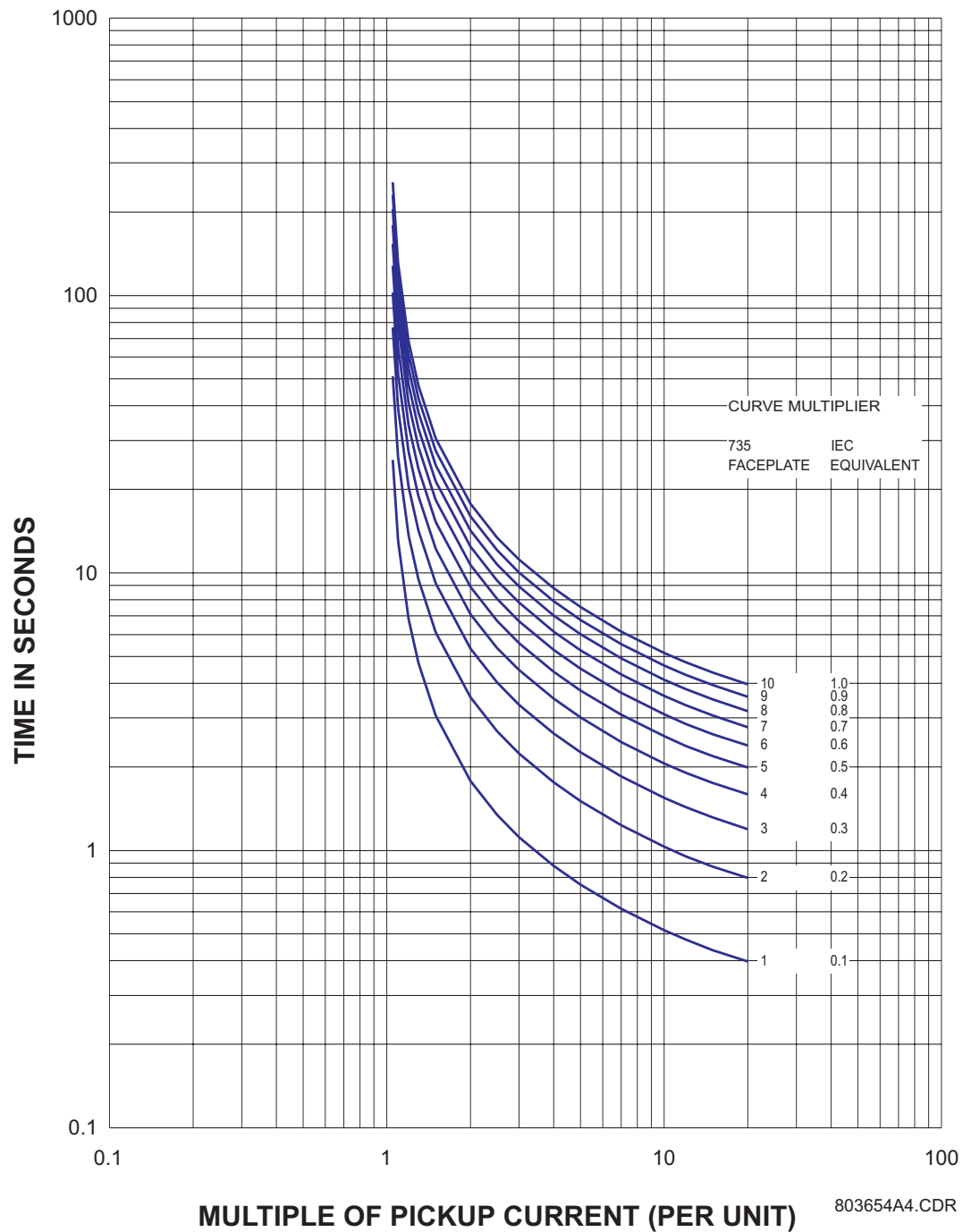
Figure 5–10: IEC SHORT TIME CURVES
