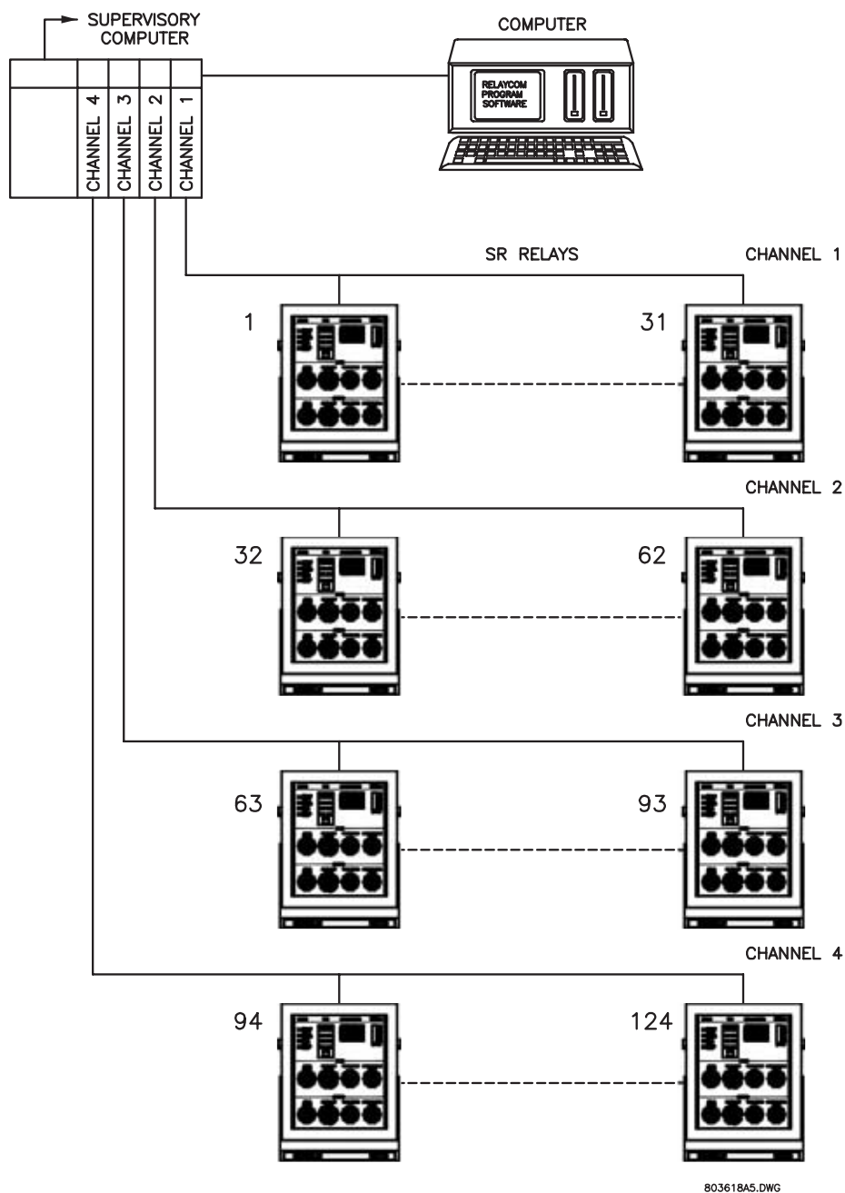
Figure 2-13: 4 CHANNEL, 124 RELAY SYSTEM
