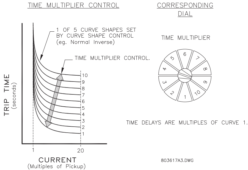
Figure 3-4: PHASE MULTIPLIER TIME SETTING
