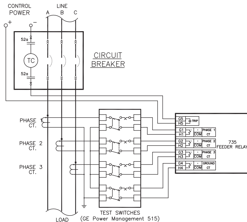
Figure 2-10: BACKUP WIRING – RESIDUAL
