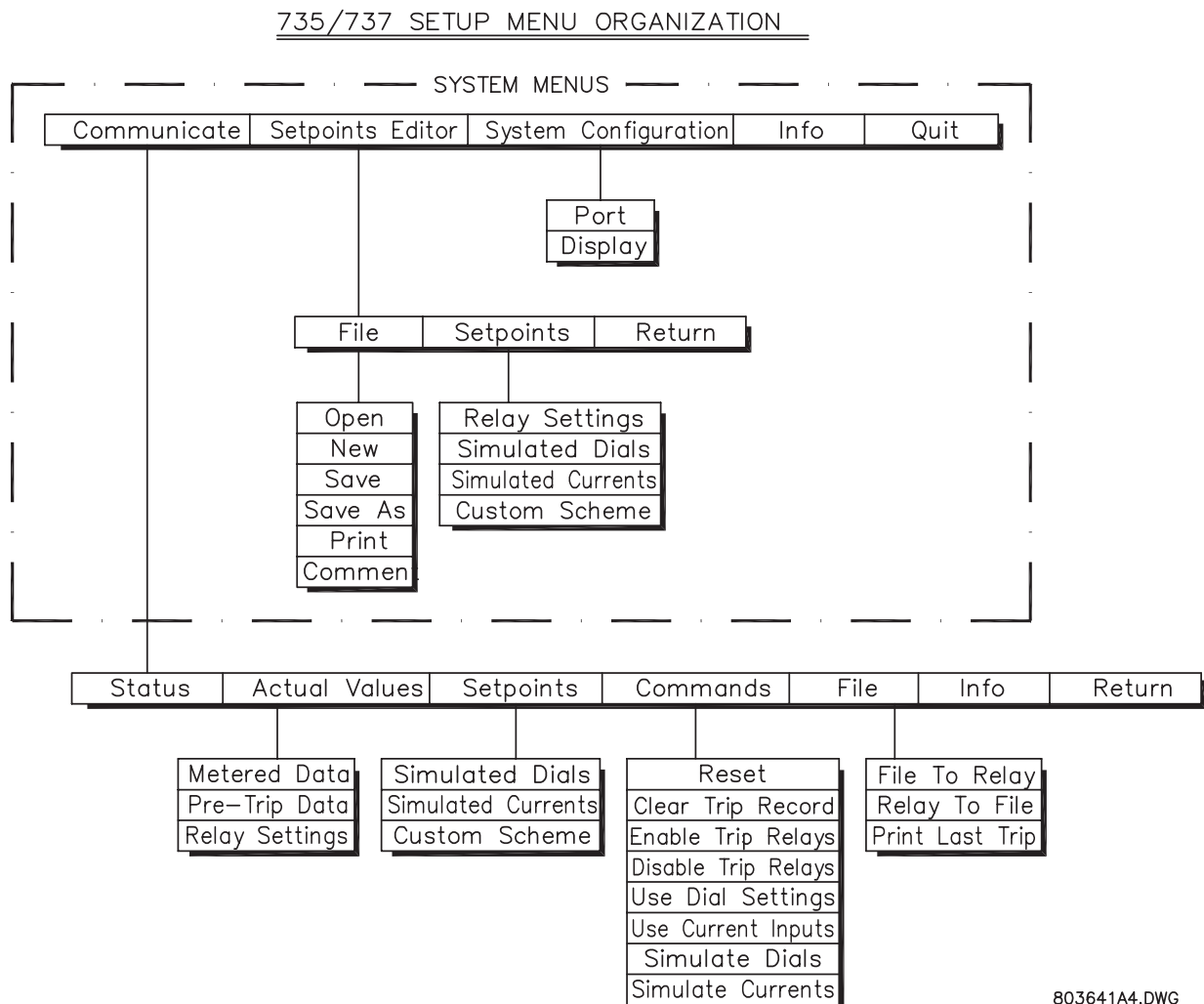
Figure 3–10: SETUP SOFTWARE SYSTEM MENUS
