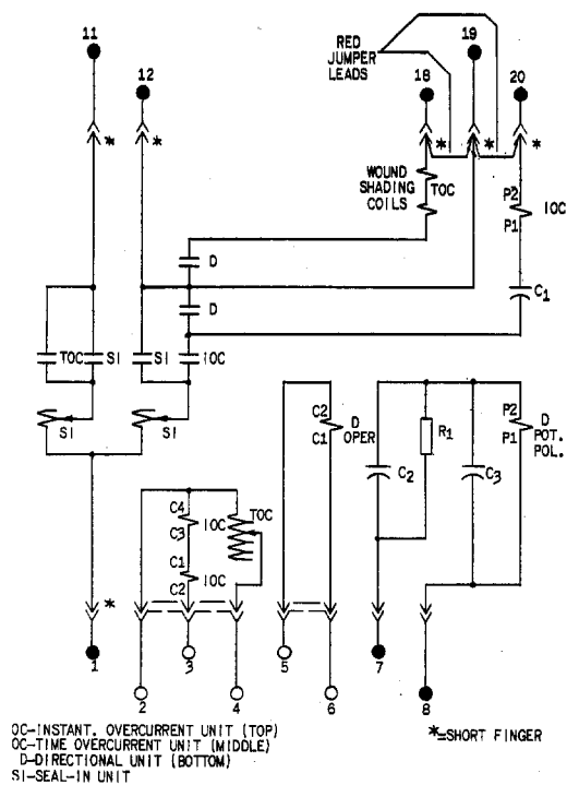
Fig. 2 Internal Connections For Type JBC51E Relay (Front View)
