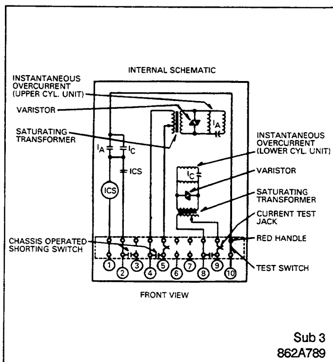
Fig. 3. Internal Schematic of KC-2 Relay with 1 Amp ICS Unit.
