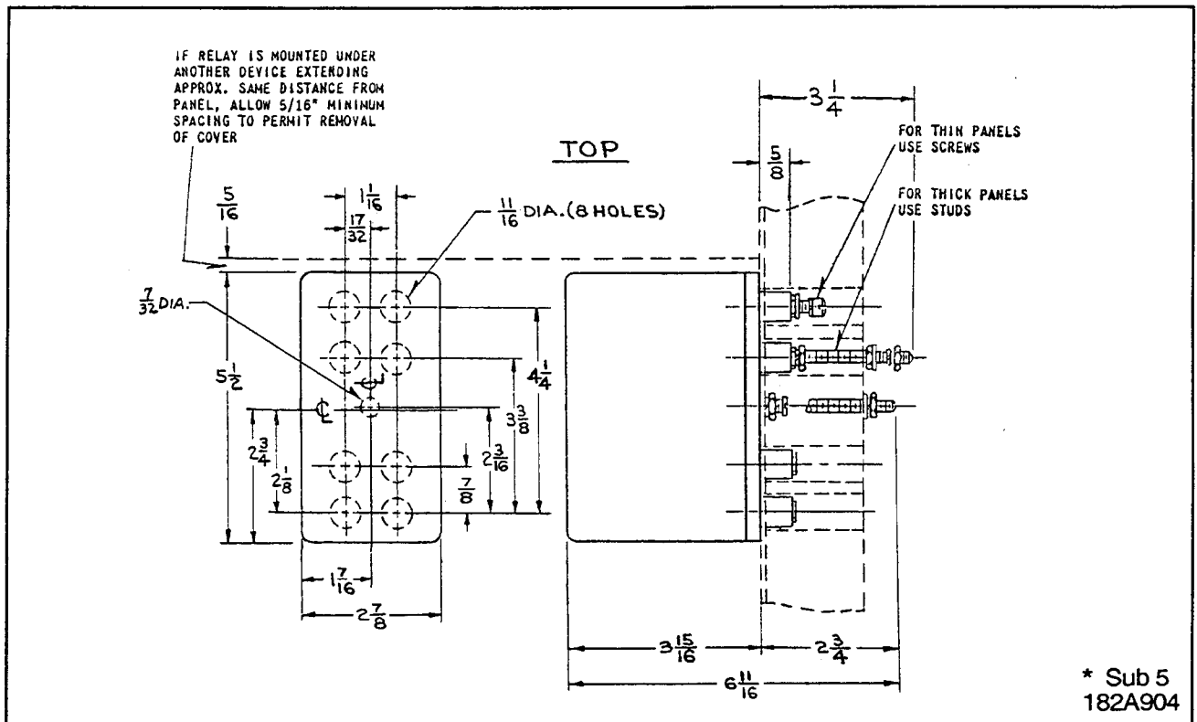
Figure 6. Outline and Drilling Plan for the Type TR-1 Auxiliary Tripping Relay in the Projection (molded base, glass window cover) case.
