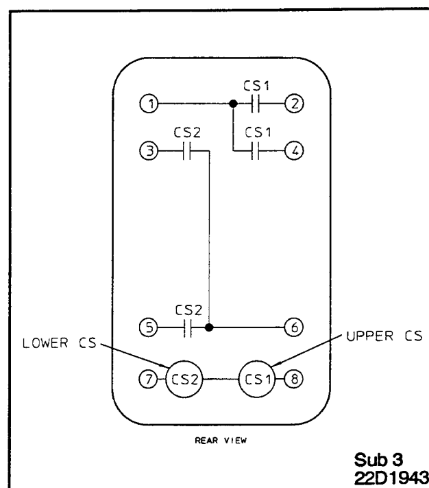
Figure 2. Internal Schematic of the two unit TR-1 Auxiliary Tripping Relay.
