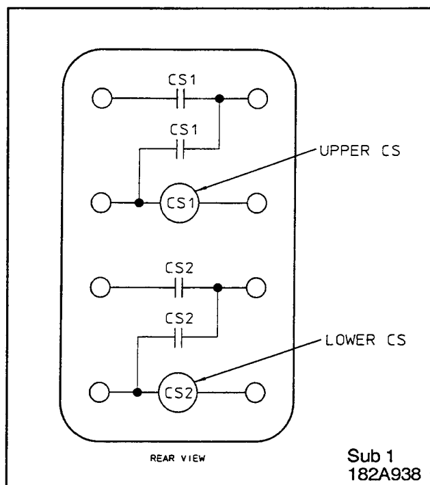
Figure 3. Internal Schematic of the two unit Type TR-1 Auxiliary Tripping Relay with Independent CS Circuits.
