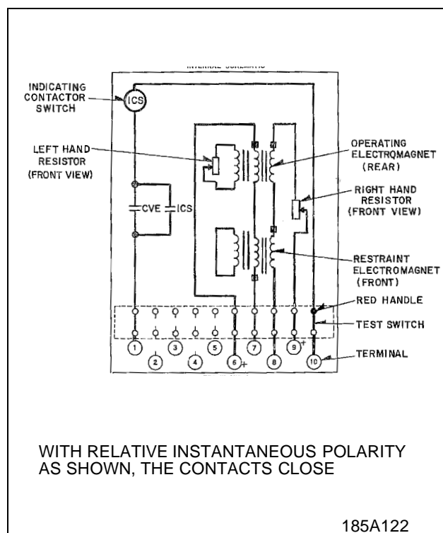
Figure 18. Internal Schematic CVE Relay with ICS Unit.
