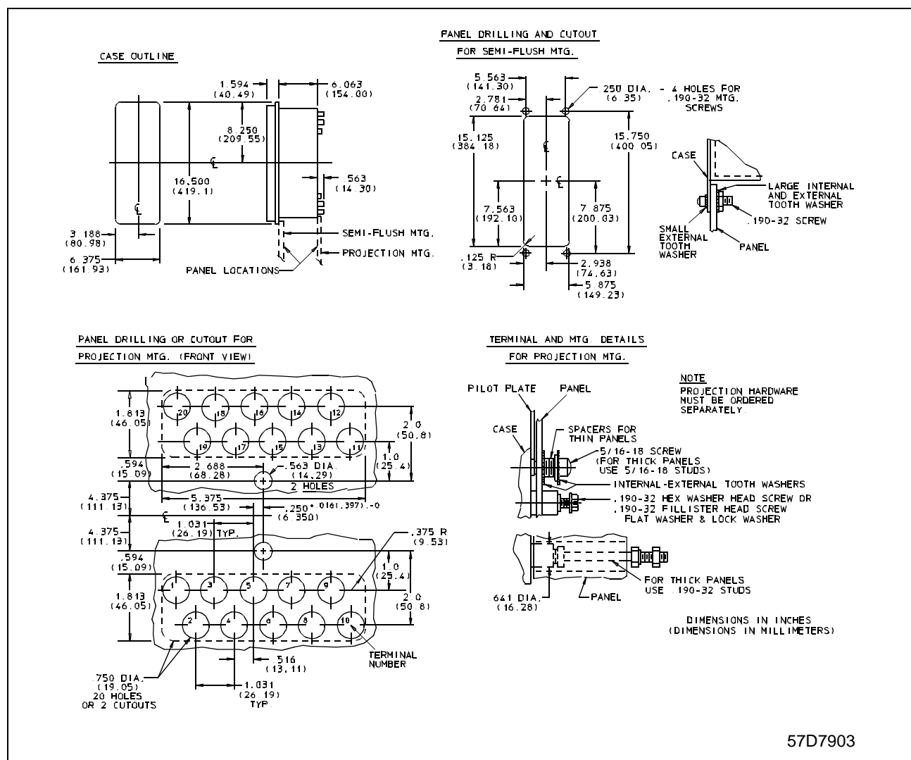
Figure 33. Outline &amp; Drilling diagram for Relay Case Type FT-32.
