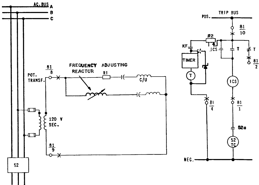
Figure 10: External Connections for the Type KF Under-frequency Relay with dc Operated Auxiliary Time Delay Unit.
