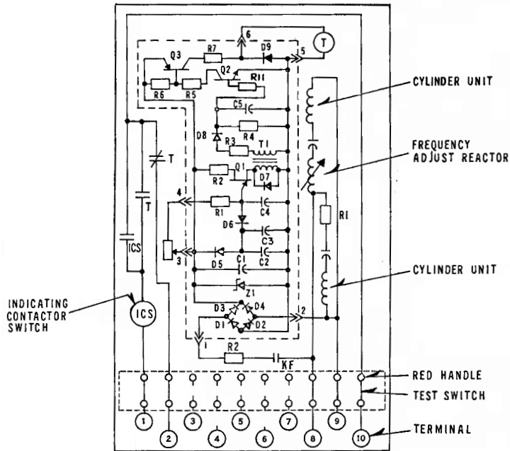
Figure 2: Internal Schematic of Type KF Relay with ac Operated Adjustable Auxiliary Time Delay Unit.
