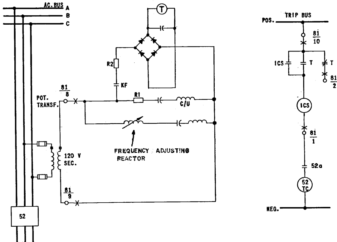
Figure 9: External Connections for the Type KF Under-frequency Relay with ac Operated Auxiliary Time Delay Unit.
