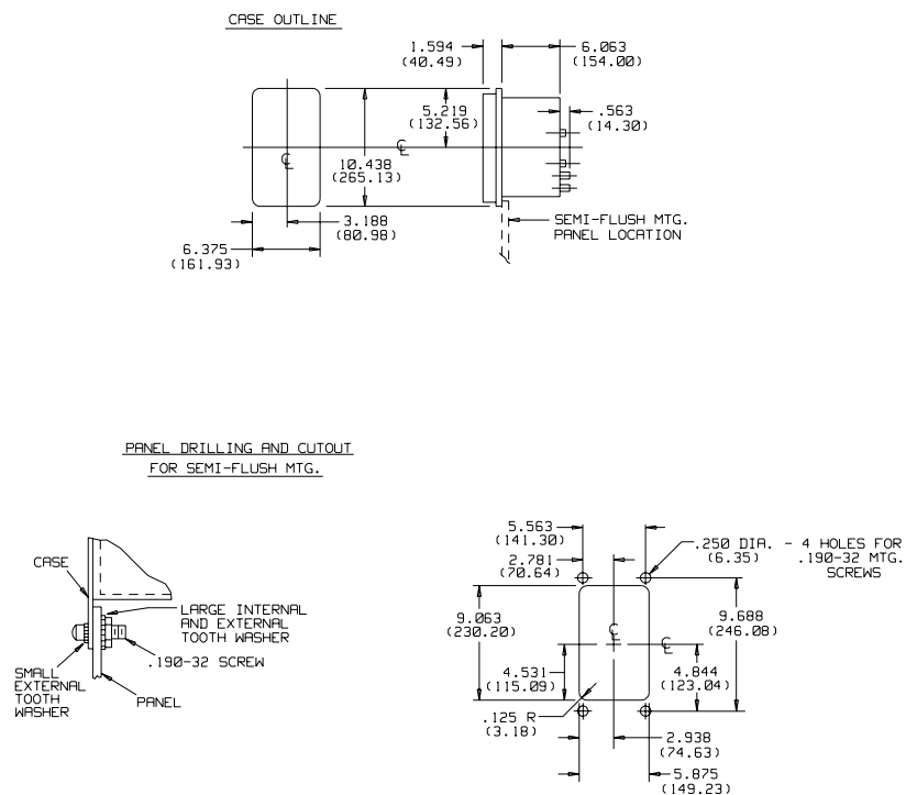
Figure 12: Outline & Drilling Plan for the Type KF Relay in Type FT 21 Case.
