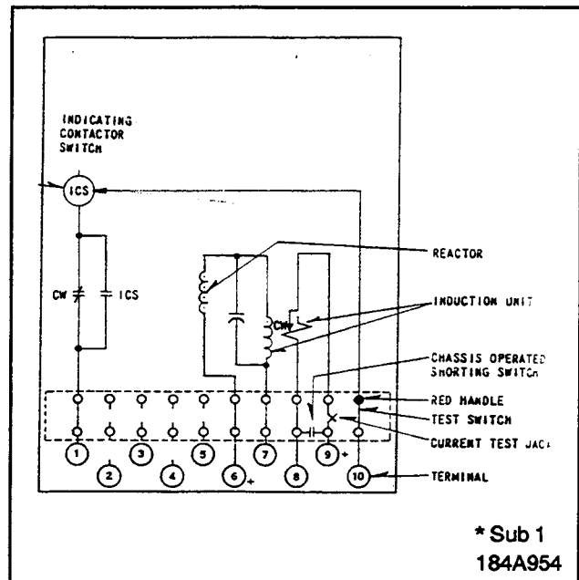
Figure 3. Internal Schematic of the Under Power Type CW Relay in the Type FT 21 Case.
