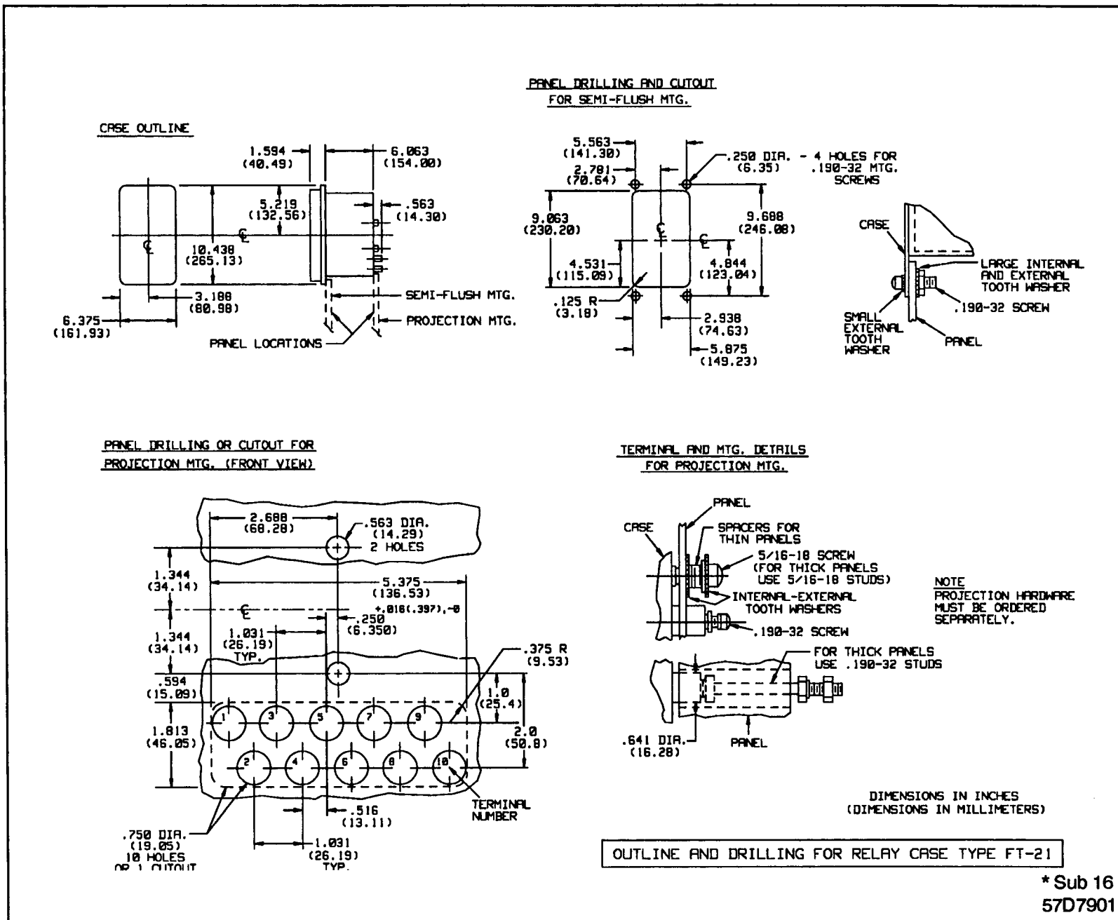
Figure 8. Outline and Drilling Plan for the Type CW Relay in the Type FT 21 Case.
