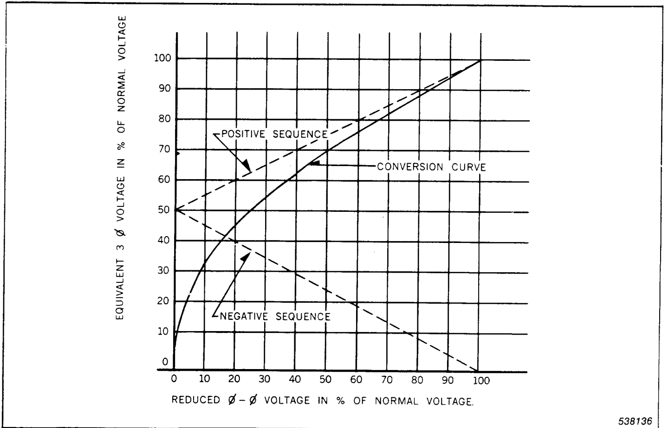
Fig. 4. Conversion curve for three phase vs. phase to phase voltages for the type KP Voltage Relay.
