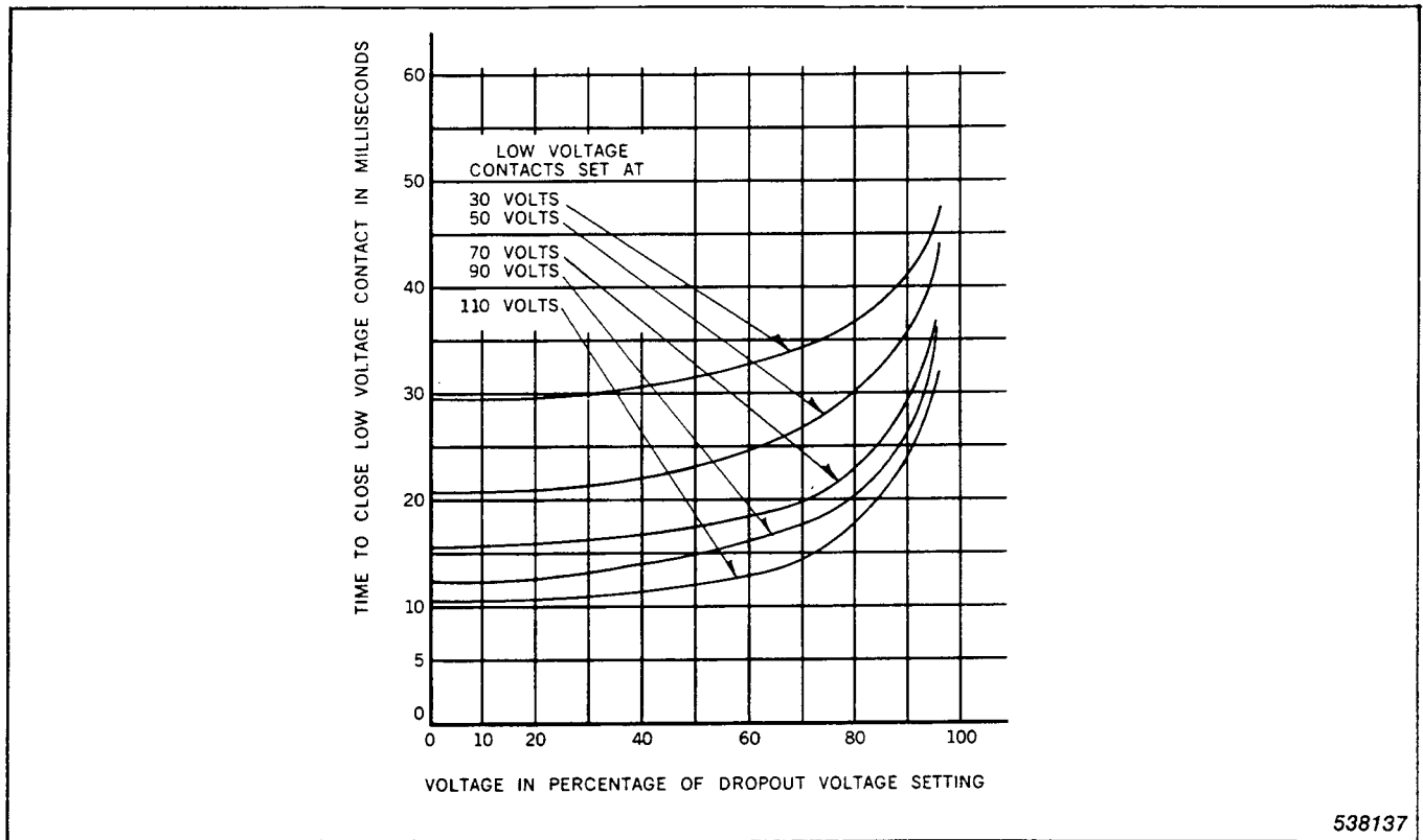
Fig. 5. Typical undervoltage time curves for the type KP Voltage Relay.
