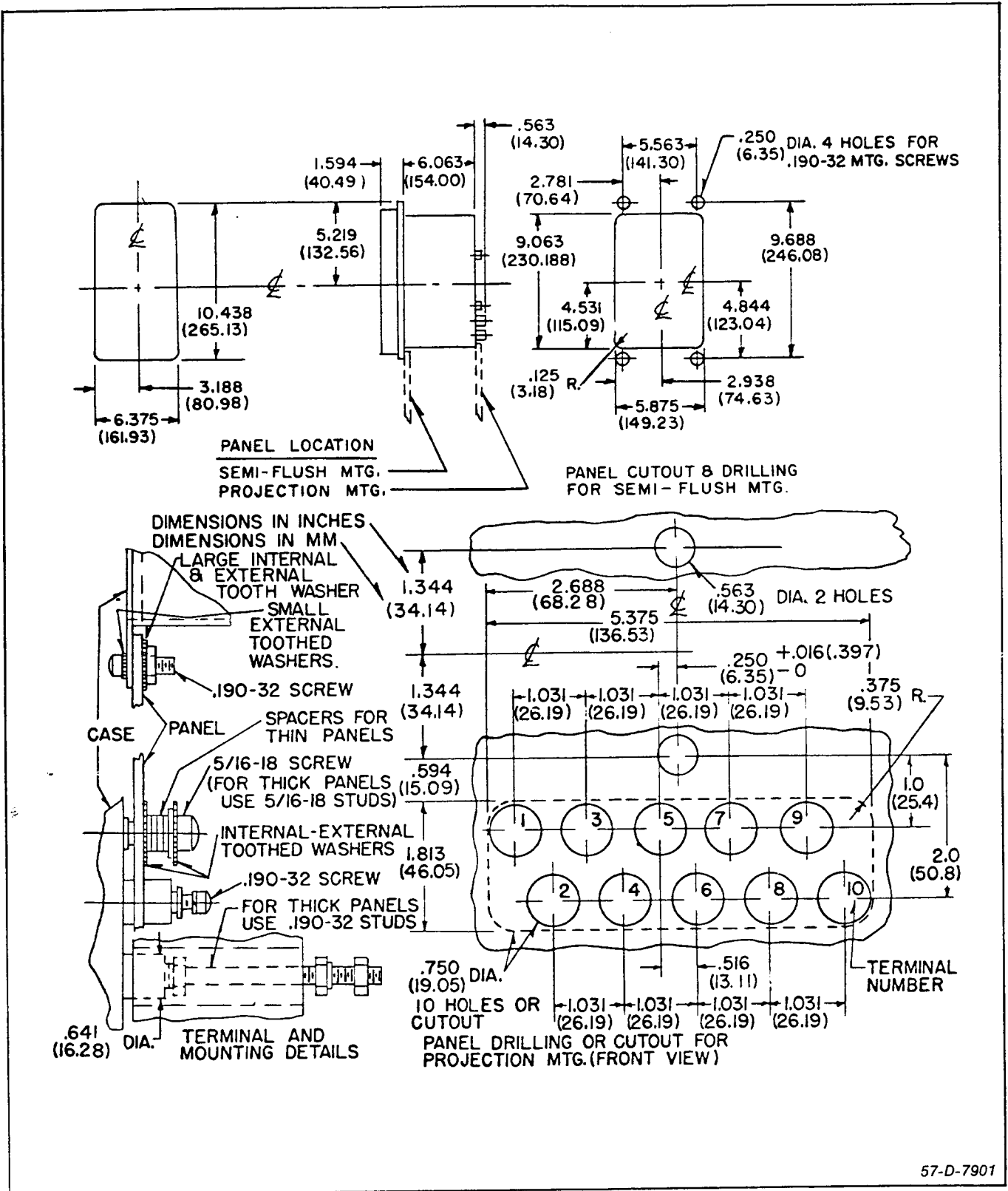
Fig. 8. Outline and drilling plan for the Type KP Voltage Relay in the type FT21 case.
