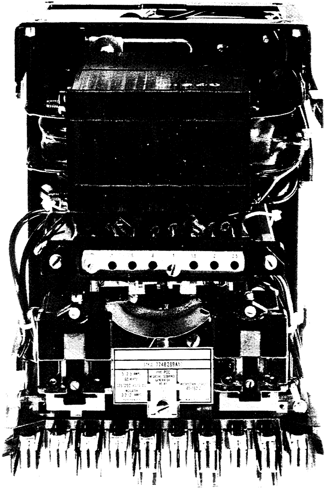
⊕ Fig. 1. Type POQ Relay in FT-21 case (Front View).
