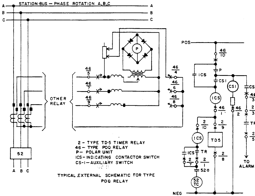
Fig. 5. External Schematic for Type POQ Relay.
