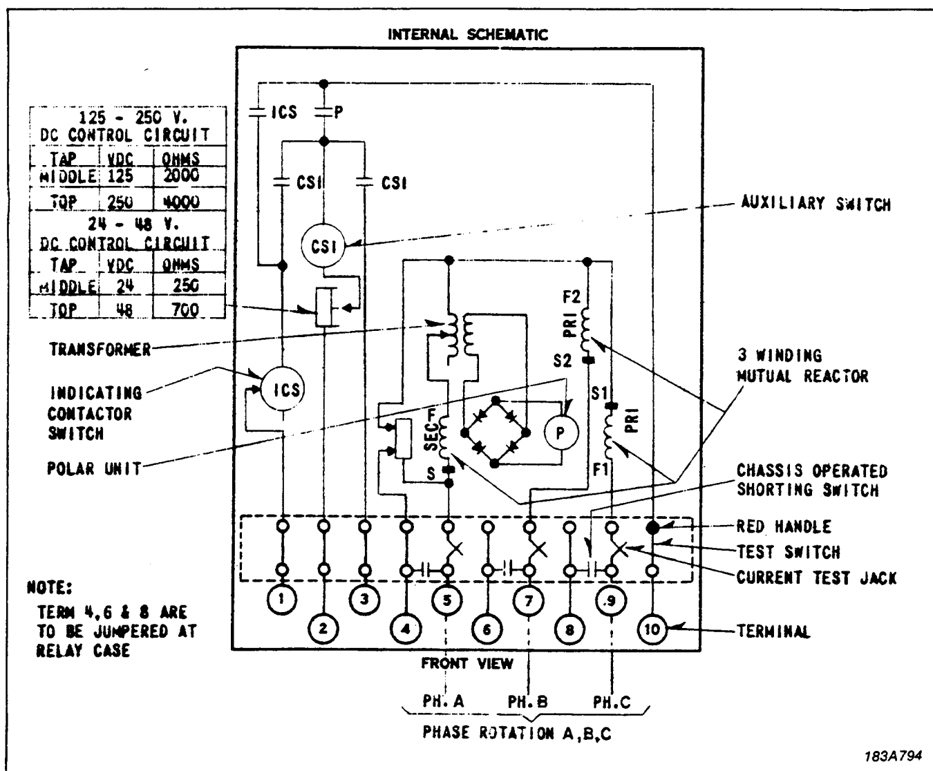
Fig. 3. Internal Schematic of the Type POQ Relay in FT-21 case.
