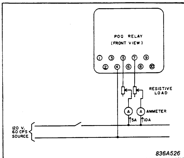
Fig. 6. Test connections for the Type POQ Relay.
