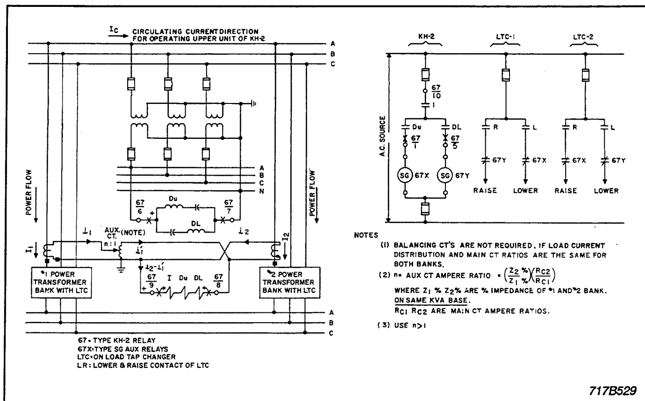
Figure 3. External Schematic
