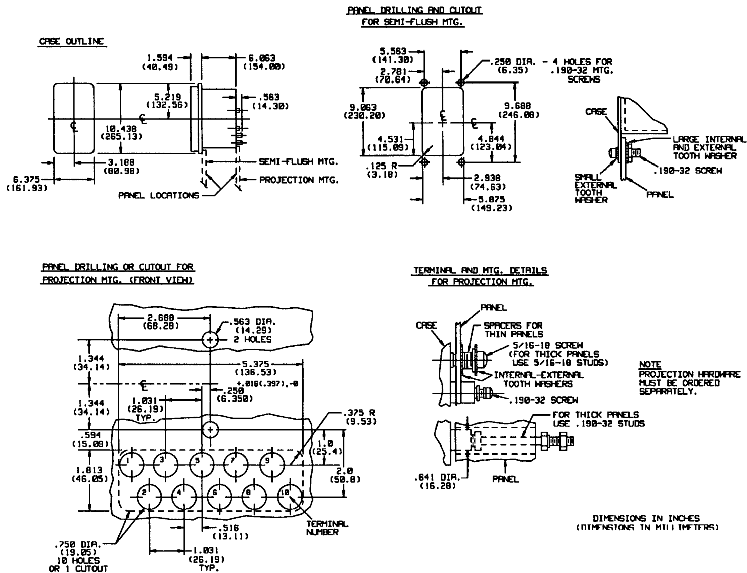
Figure 4. Outline and Drilling (FT-21 Case)
