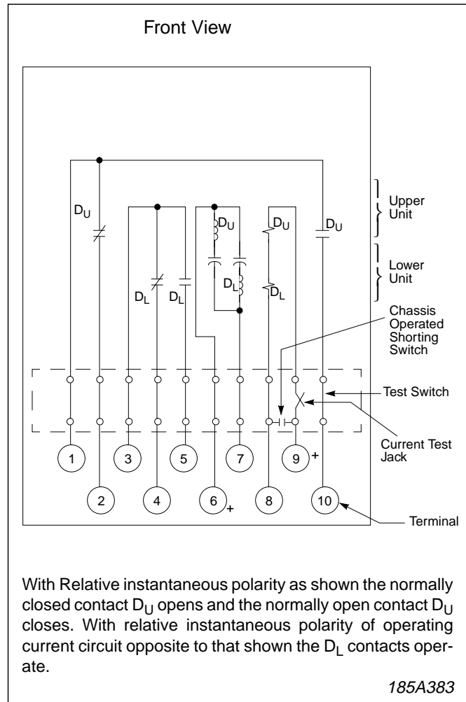
Figure 1. Internal Schematic (Without IT Unit).
