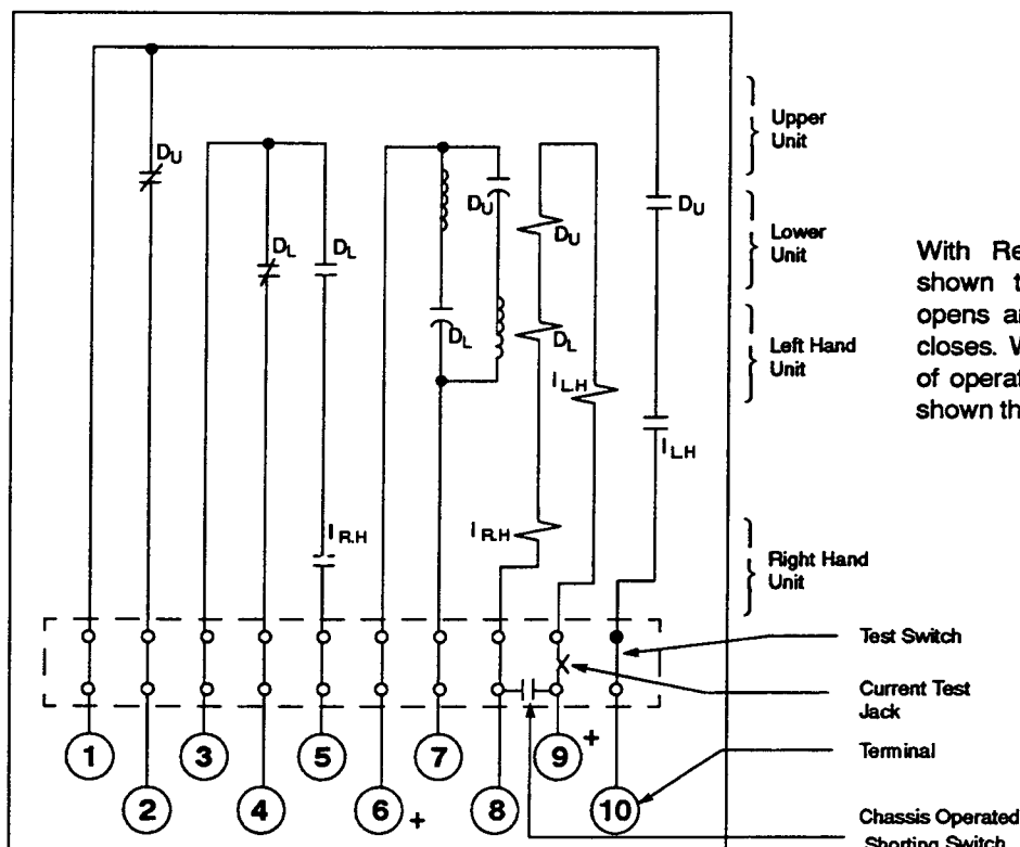
Figure 2a. Internal Schematic (with IT Units) (.5 to 2 amp range)
