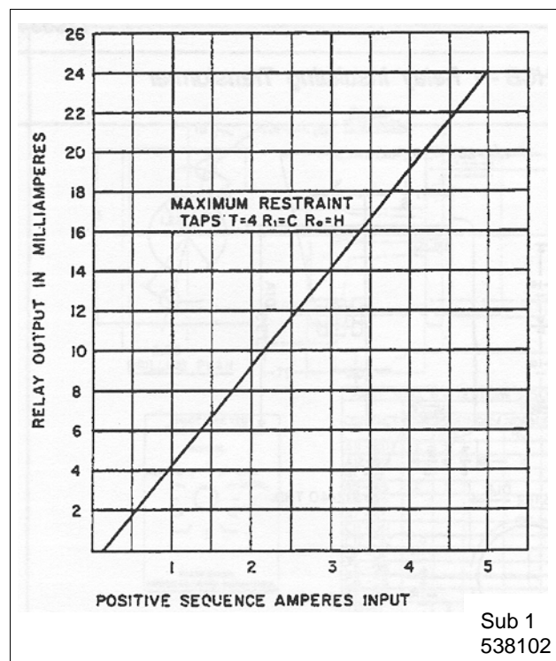
Figure 13: Typical Curve of Relay Output vs. Positive Sequence Input - Test Switch in Local Position.
