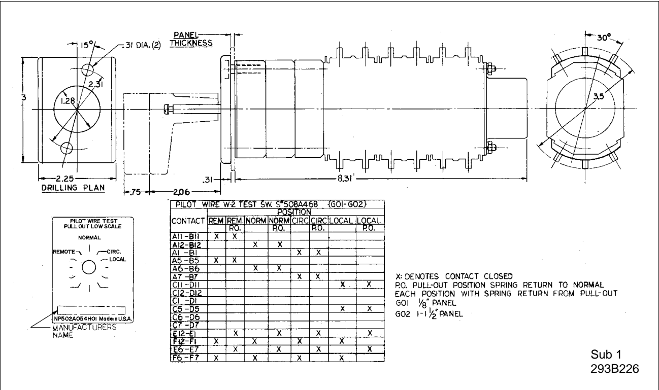
Figure 18: Outline and Drilling Plan of the Type W-2 Test Switch.
