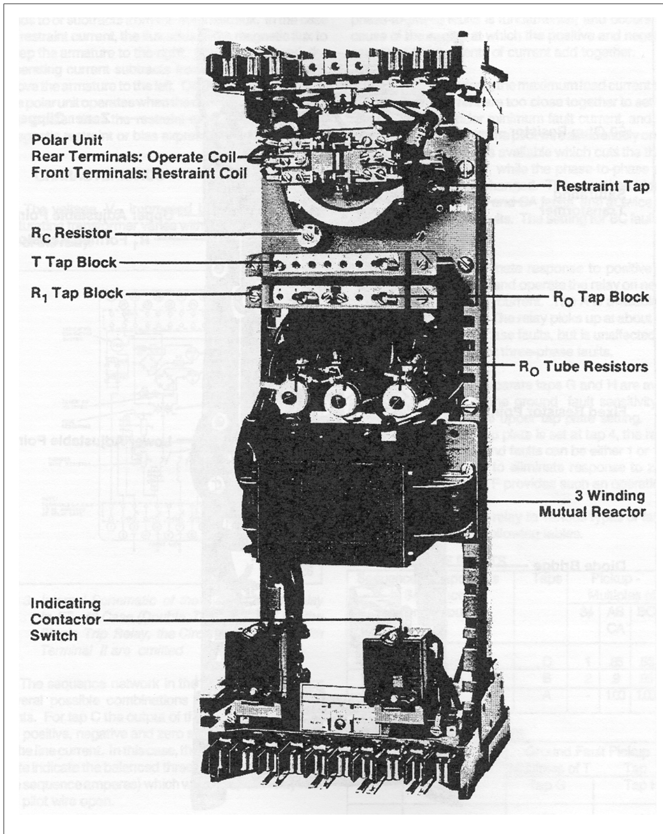
Figure 1: Type HCB -1 Relay Without Case (Front View)
