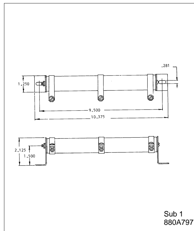
Figure 14: Outline and Drilling Plan of S#290B664G65 Balancing Resistor for Three-Terminal Line Application.
