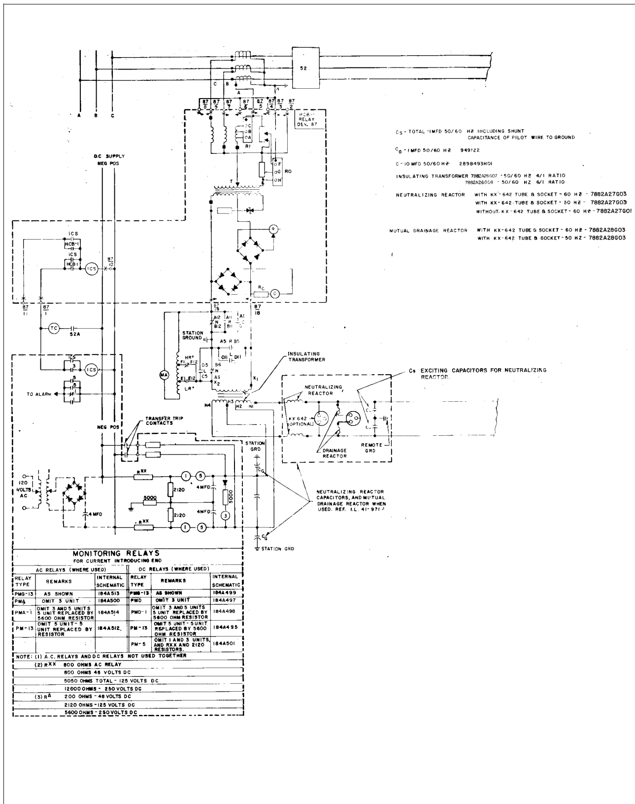
Figure 10: Typical HCB-1 Relay System
