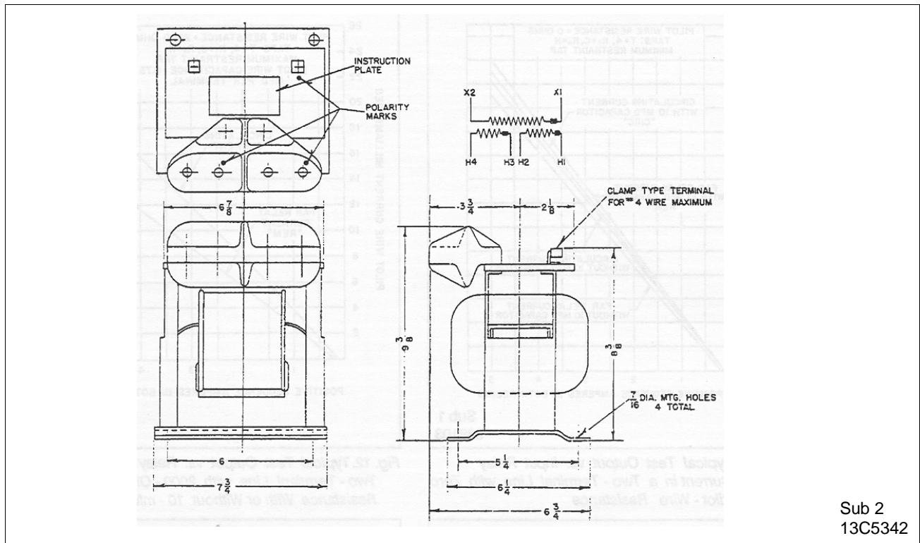
Figure 15: Outline and Drilling Plan of HCB-1 Relay Insulating Transformer
