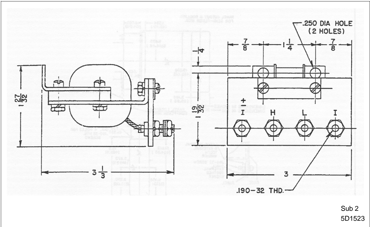
Figure 17: Outline of the Test Milliameter Auxiliary Transformer.
