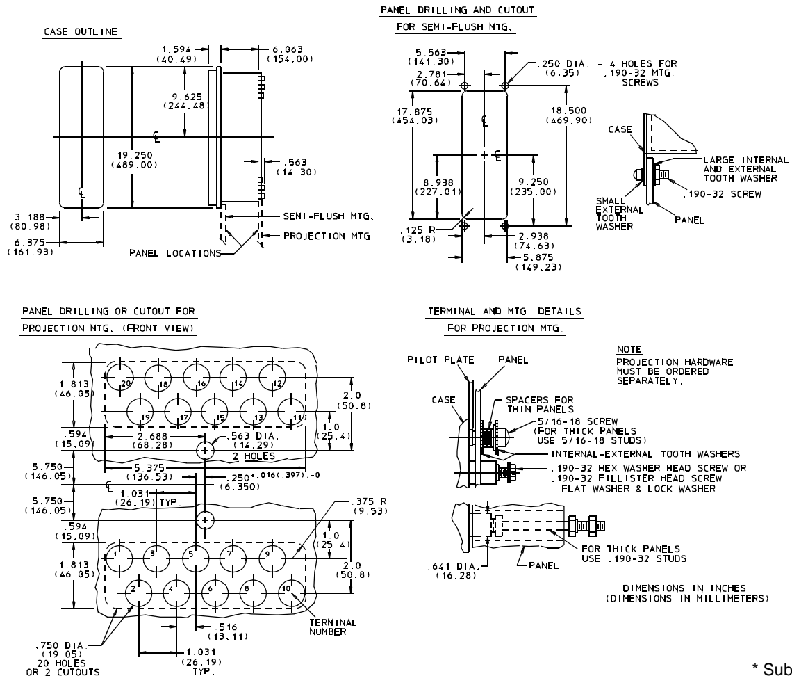
Figure 19: Outline and Drilling Plan for the Type HCB-1 Relay in the Type FT-42 Case.
