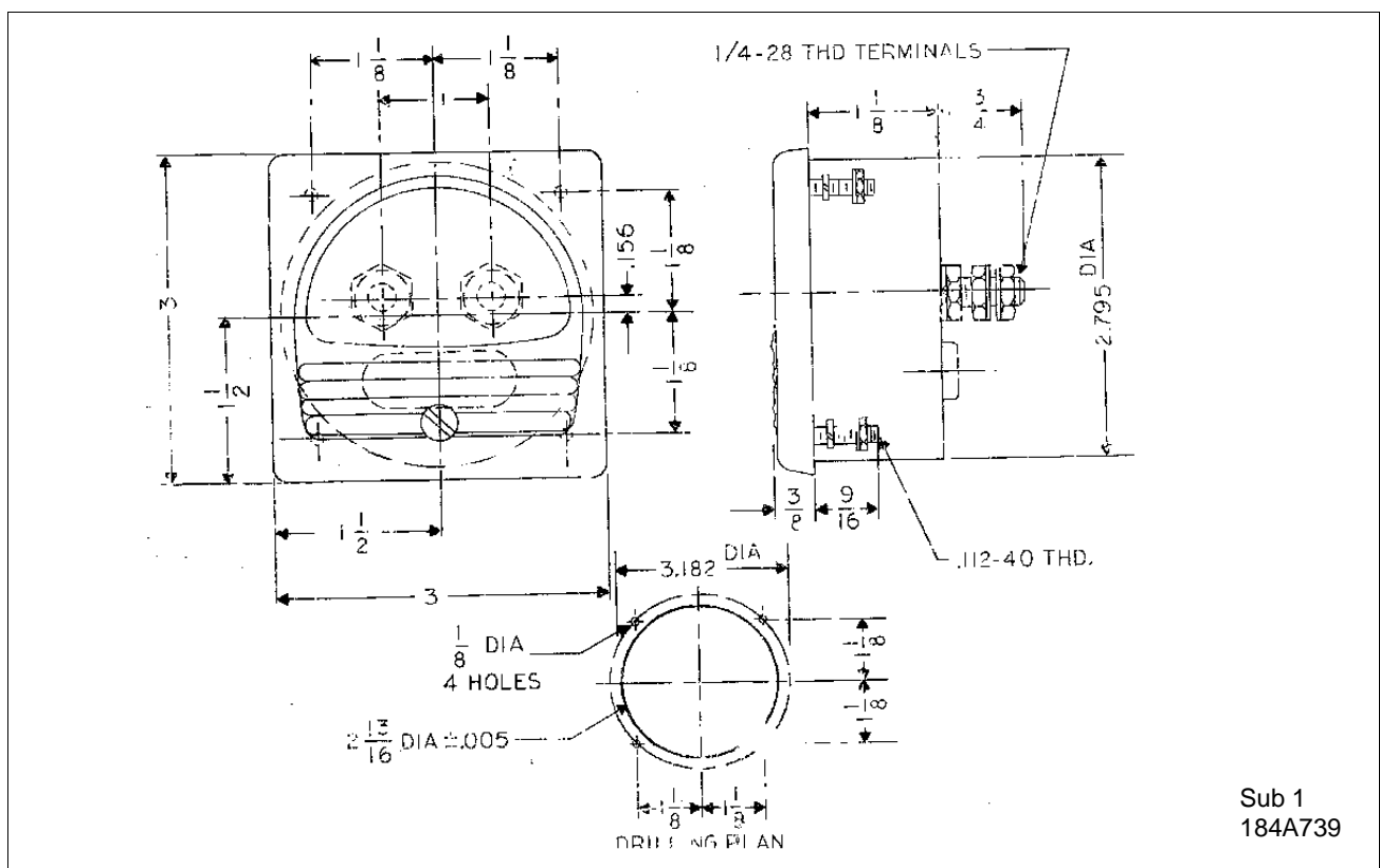
Figure 16: Outline and Drilling Plan of the Semi-Flush - Type Test Milliammeter
