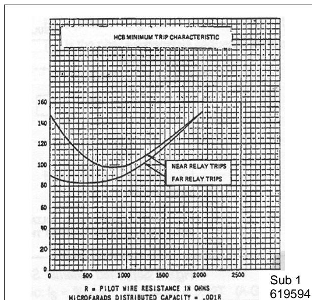
Figure 6: Typical Curves Showing the Effect of the Pilot-wire on Minimum Trip Current, Two-Terminal Line (Maximum Resistant Tap). Insulating Transformer 4/1 ratio
