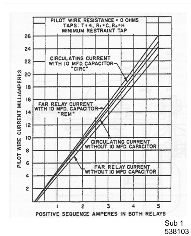
Figure 11: Typical Test Output vs. Input Relay Current in a Two-Terminal Line with Zero Pilot-Wire Resistance.
