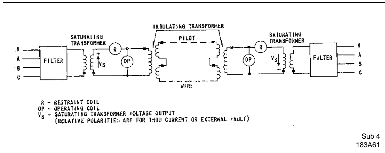
Figure 4. Simplified External Schematic of the HCB-1 Relay System
