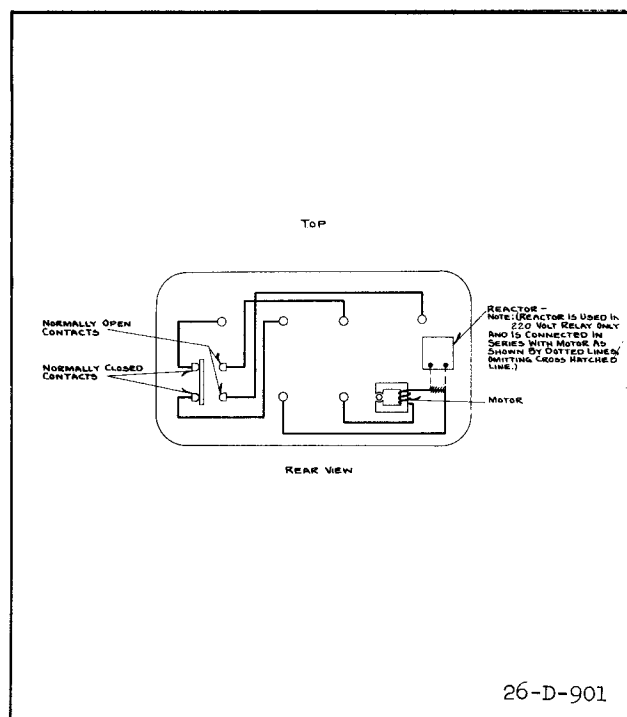
Fig. 2—Internal Connections of Six-Terminal Type TD Relay.
