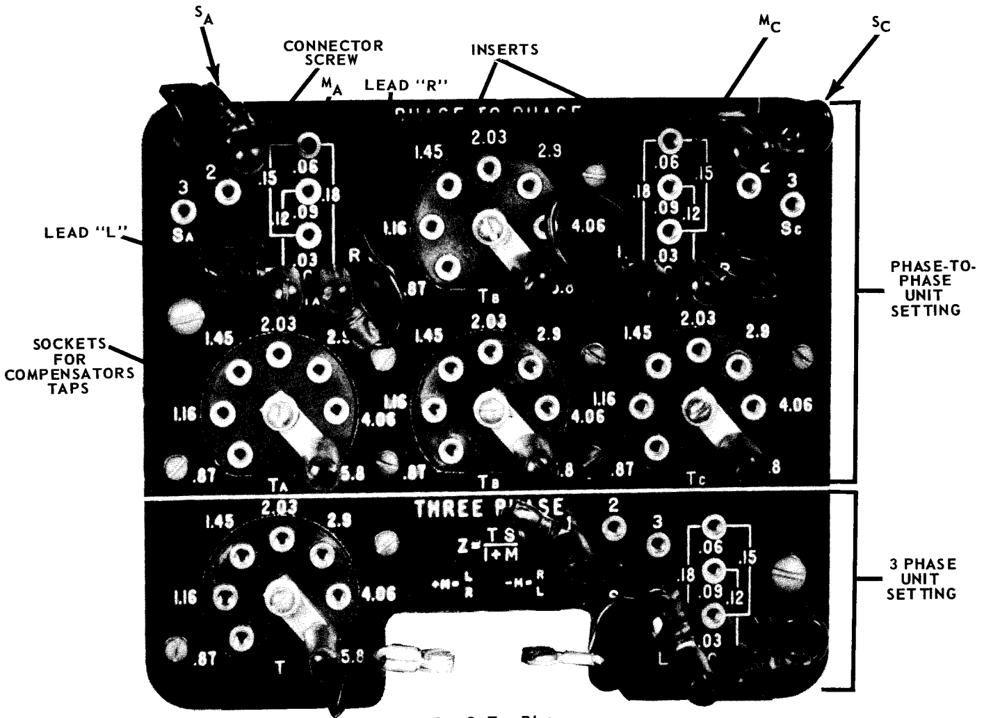
Fig. 3 Tap Plate
