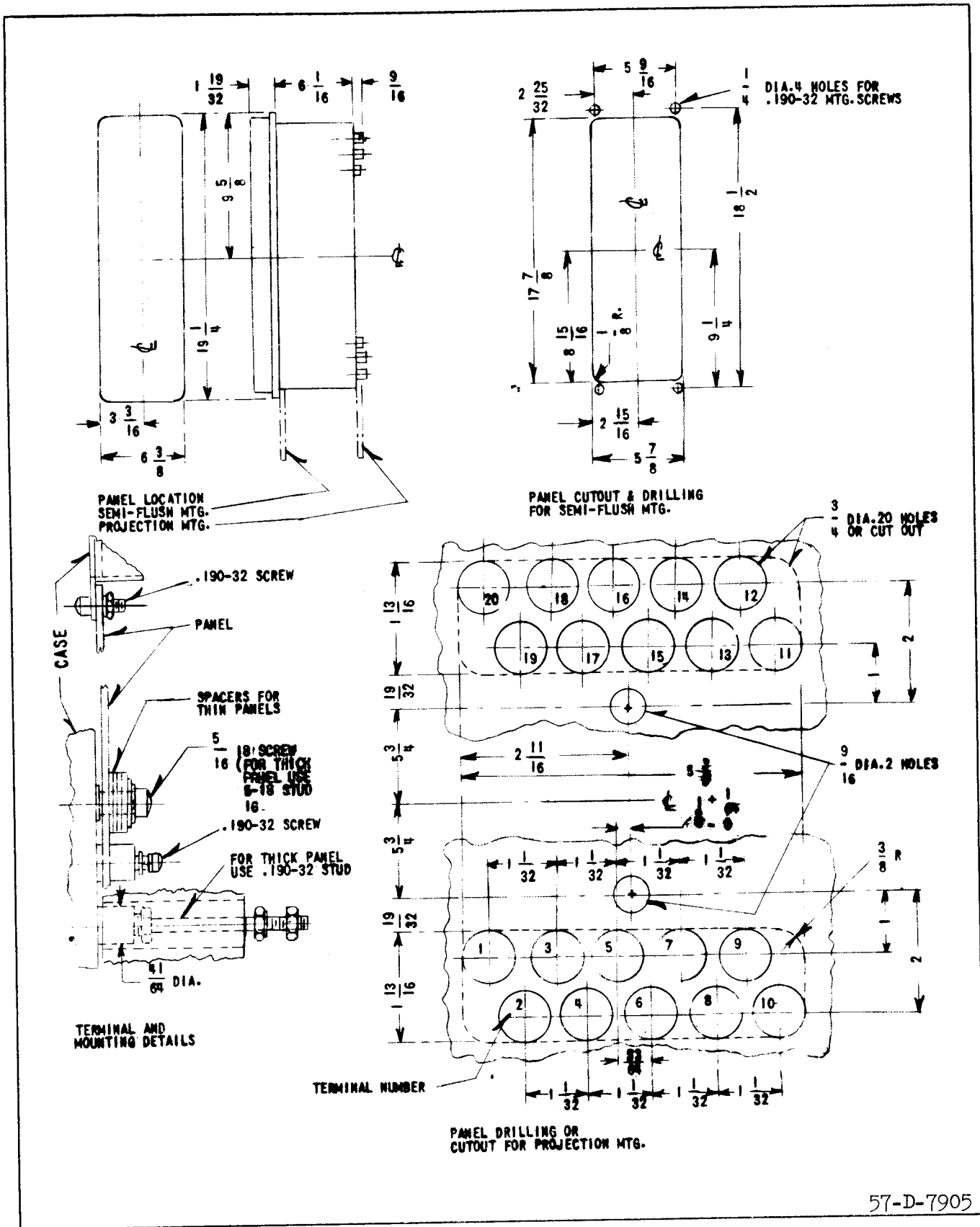
Fig. 24 Outline and Drilling Plan for the Type KD-4 and KD-41 Relays in The Type FT 42 Case.
