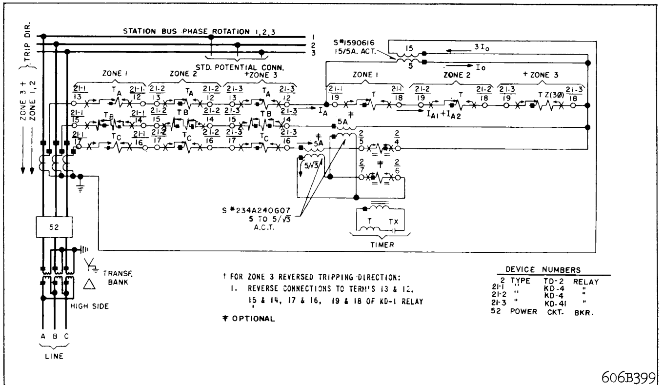
Fig. 20 A.C. External Schematic of Two Type KD-4 & One KD-41 Relay – Wye-Delta Bank Termination with Grounded Wye on Relay Side.
