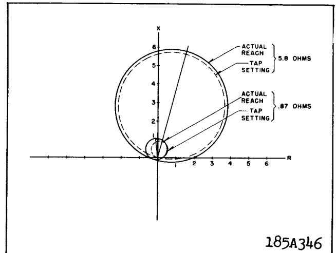
Fig. 11 Impedance Circle for Three-Phase Unit in Type KD-41 Relay.
