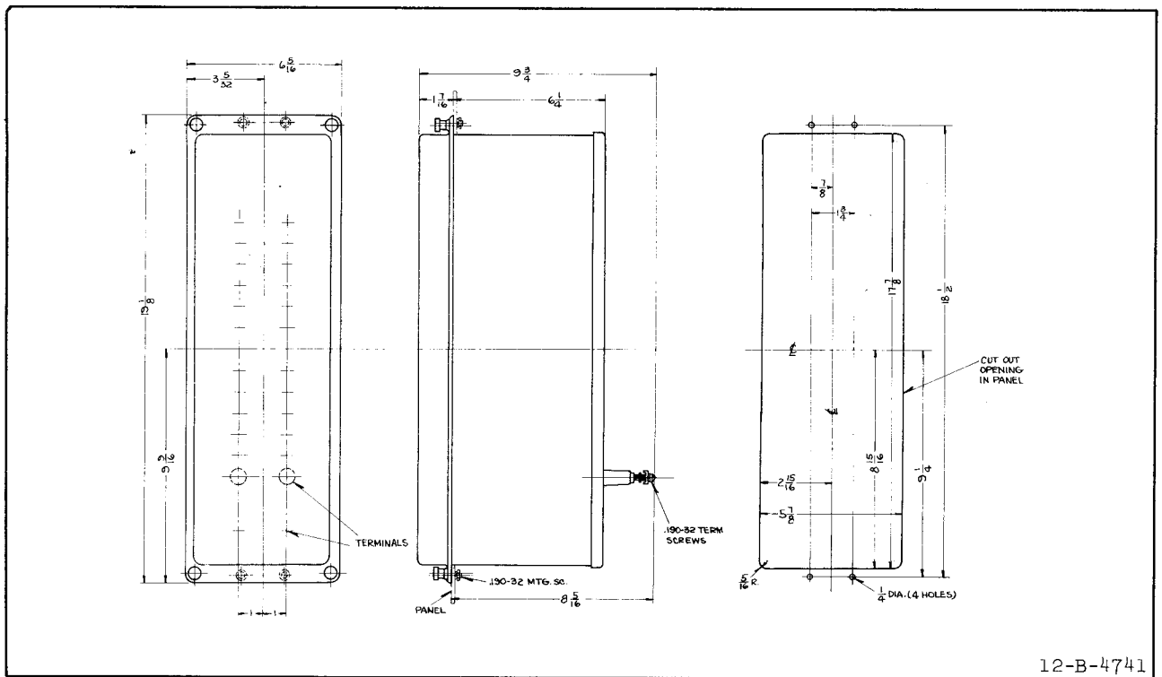
Fig. 9—Outline and Drilling Plan for the M20D Semi-Flush Type FT Case. See the Internal Schematics for the Terminals Supplied. For Reference Only.
