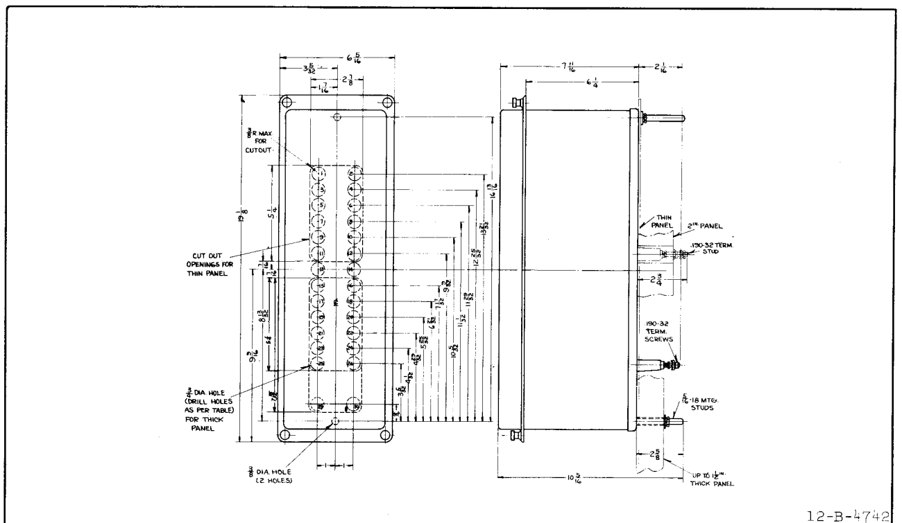
Fig. 10—Outline and Drilling Plan for the M20D Projection Type FT Case. See the Internal Schematic for the Terminals Supplied. For Reference Only.
