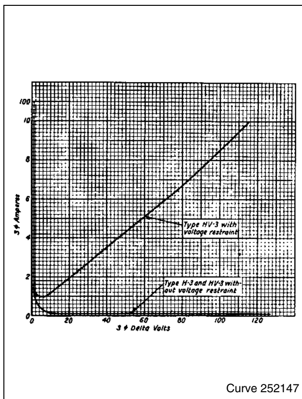
Fig. 5. Typical Sensitivity Curve for 50 and 60 Hertz, H-3 and HV-3 Relays - at Maximum Torque Angle.
