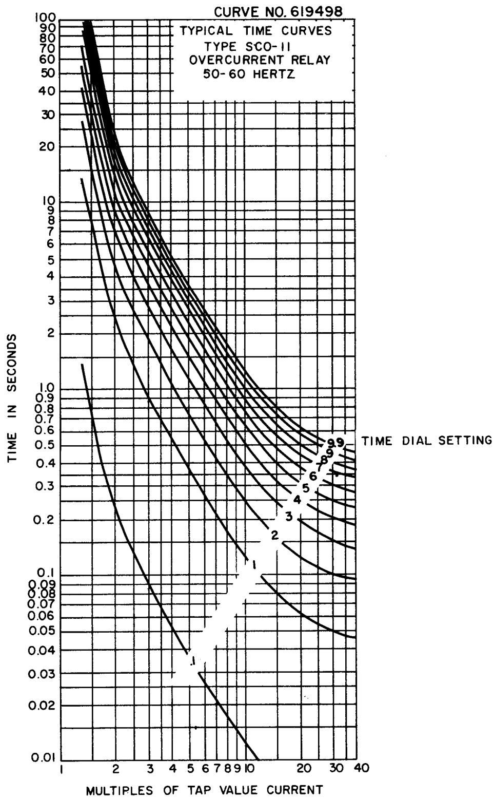
Fig. 13. Typical Time Curves of the TYPE SCO-11 Relay
