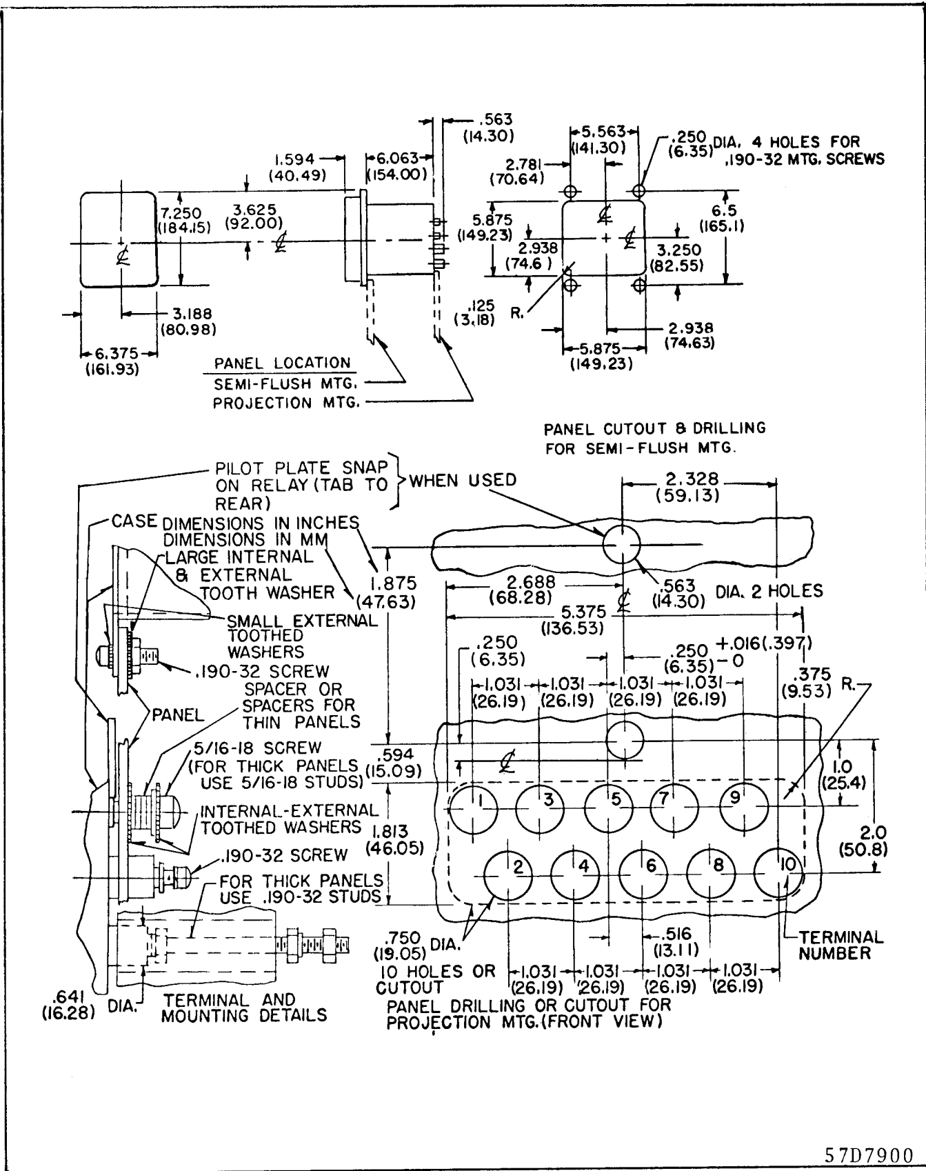
Fig. 20. Outline and Drilling Plan for Type SCO Relay Single Phase in FT-11 Case
