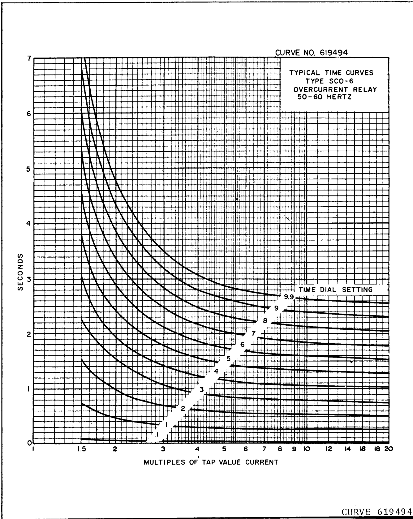
Fig. 9. Typical Time Curves of the Type SCO-6 Relay
