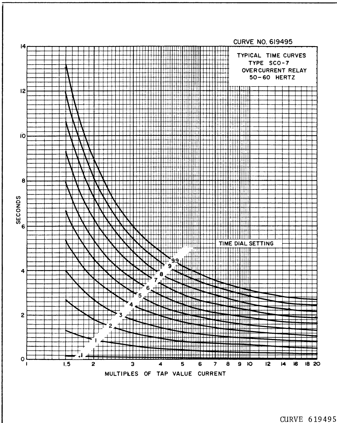
Fig. 10. Typical Time Curves of the Type SCO-7 Relay
