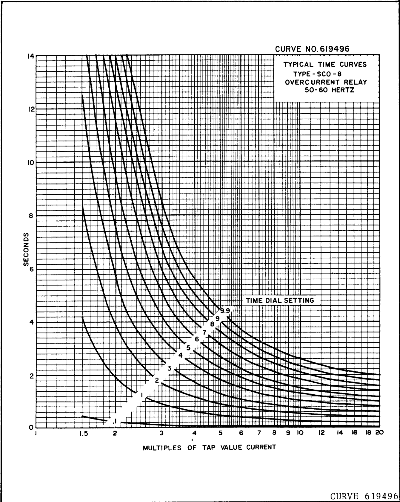
Fig. 11. Typical Time Curves of the Type SCO-8 Relay
