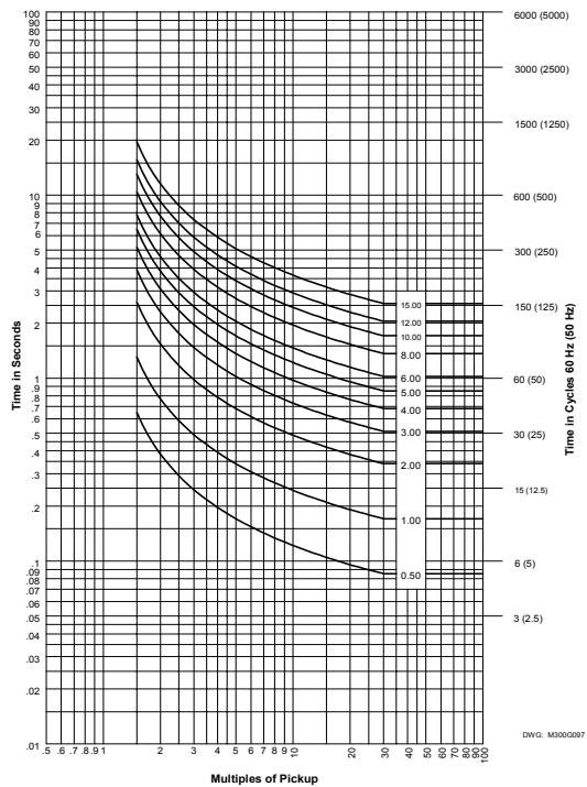
Figure 2.27: U.S. Moderately Inverse Curve: U1
