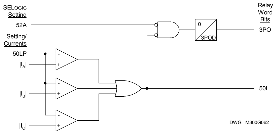
Figure 2.55: Pole Open Logic Diagram
