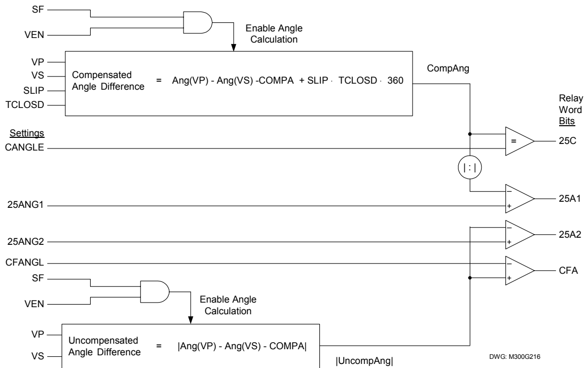
Figure 4.13: Synch-Check Function Angle Elements
