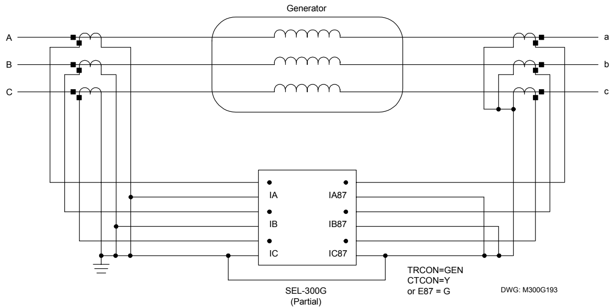
Figure B.1: Protected Generator With No Step-Up Transformer
