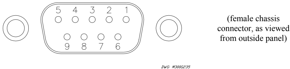
Figure 10.1: DB-9 Connector Pinout for EIA-232 Serial Ports
