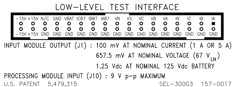
Figure 7.4: Low-Level Test Interface, 0300G3
