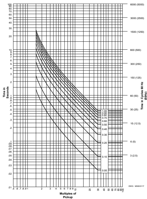
Figure 2.33: I.E.C. Class B Curve (Very Inverse): C2
