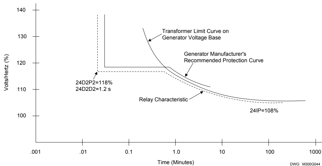
Figure 2.9: Composite Inverse/Definite-Time Overexcitation Characteristic, 24CCS=ID
