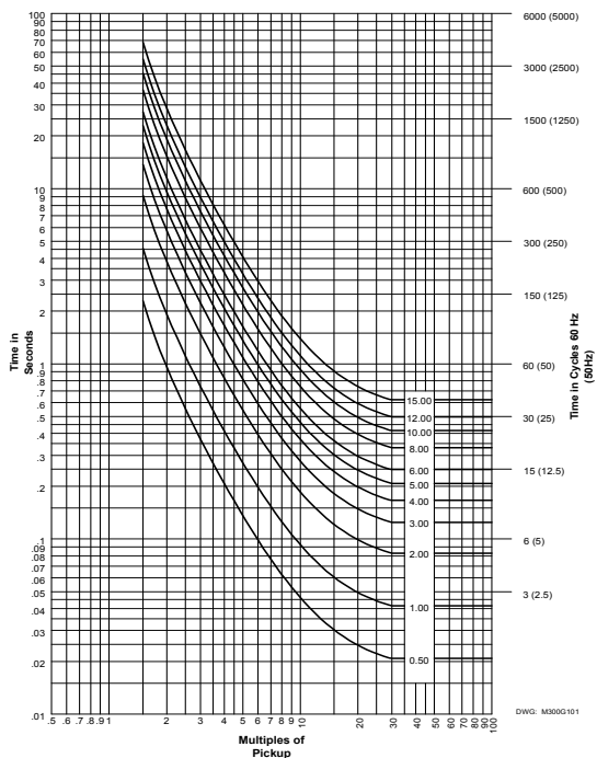
Figure 2.30: U.S. Extremely Inverse Curve: U4
