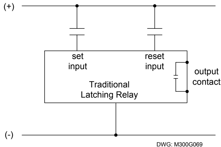
Figure 4.3: Traditional Latching Relay
