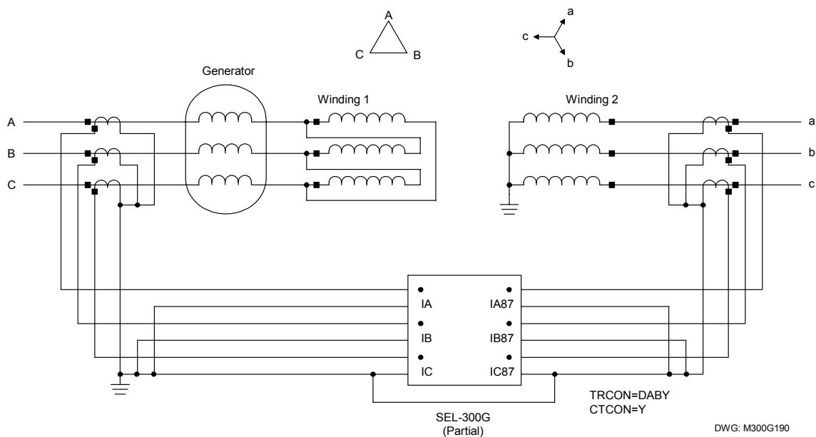
Figure B.3: Delta-Wye Power Transformer With Wye High-Side CT Connections
