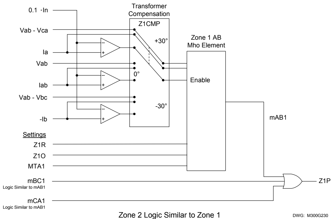
Figure 2.6: Zone 1 Mho Element Logic
