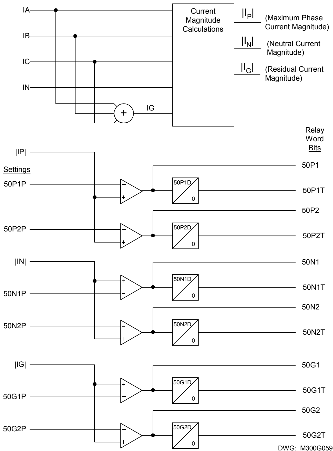
Figure 2.23: Definite-Time Overcurrent Element Logic Diagram
