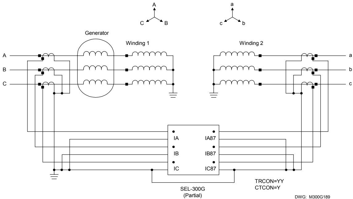
Figure B.10: Wye-Wye Power Transformer With Wye High-Side CT Connections
