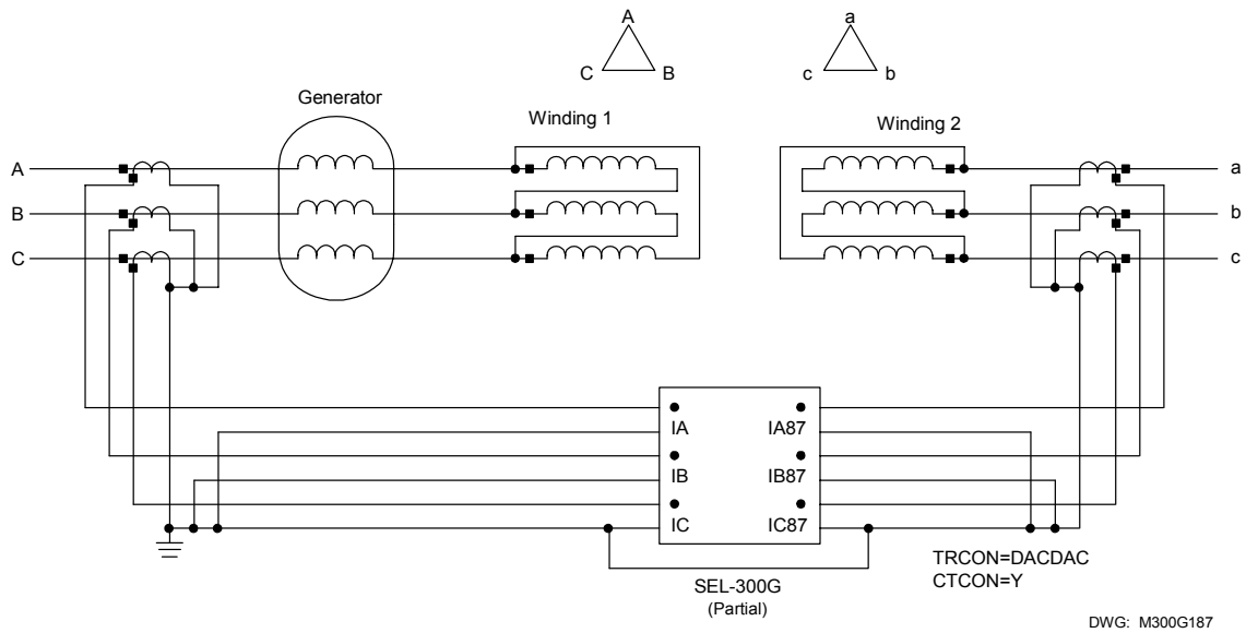
Figure B.6: Delta-Delta Power Transformer With Wye High-Side CT Connections
