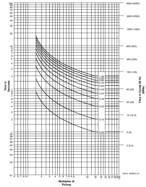
Figure 2.32: I.E.C. Class A Curve (Standard Inverse): C1
