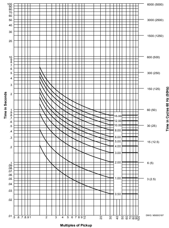
Figure 2.31: U.S. Short-Time Inverse Curve: U5
