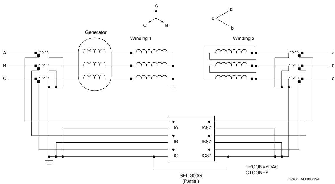
Figure B.8: Wye-Delta Power Transformer With Wye High-Side Connections
