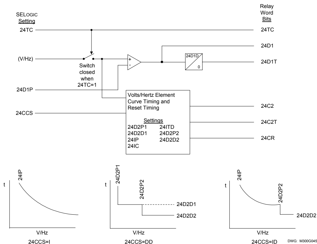
Figure 2.13: Volts/Hertz Element Logic Diagram
