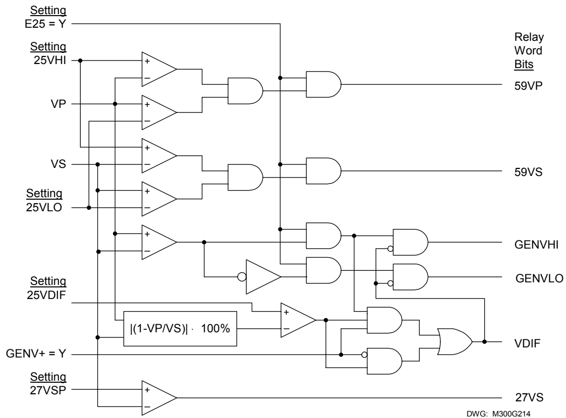
Figure 4.10: Synch-Check Function Voltage Elements
