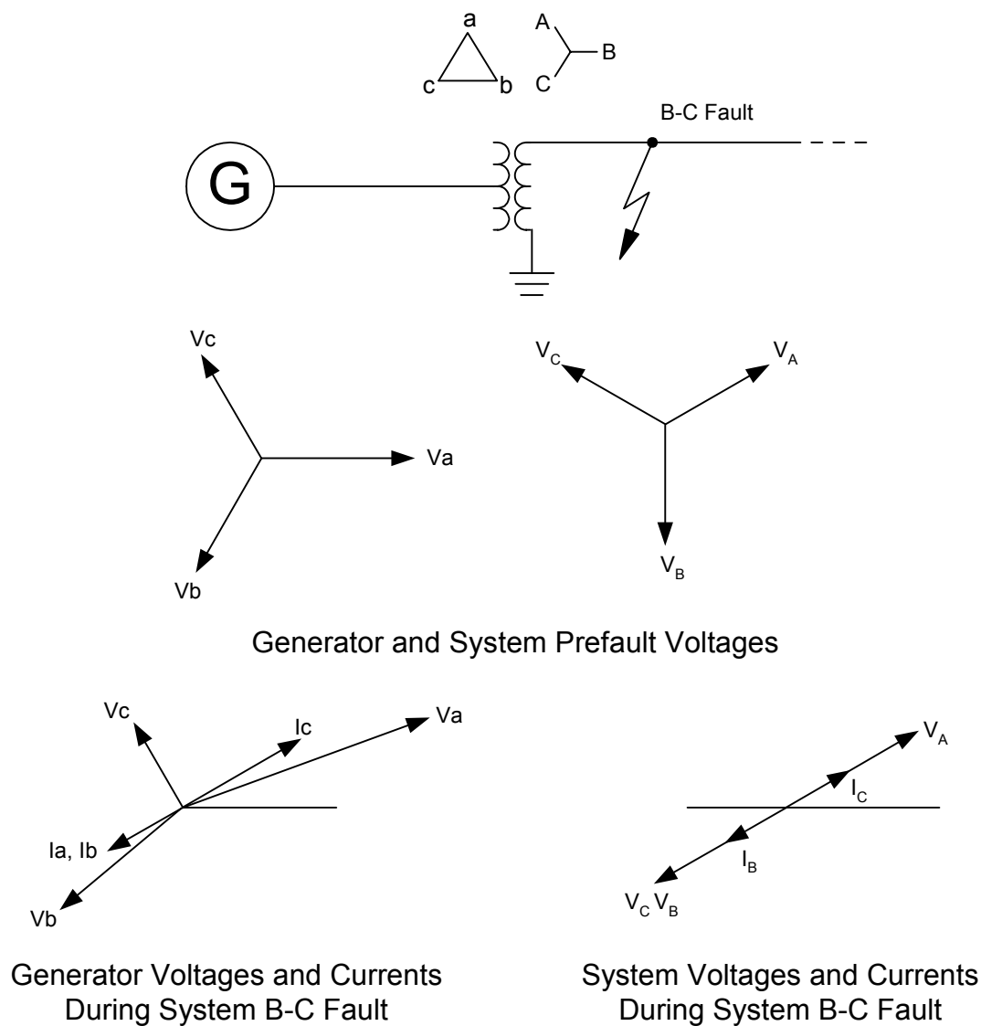
Figure 7.11: Generator Voltage and Current Relationships During a System Phase-to-Phase Fault
