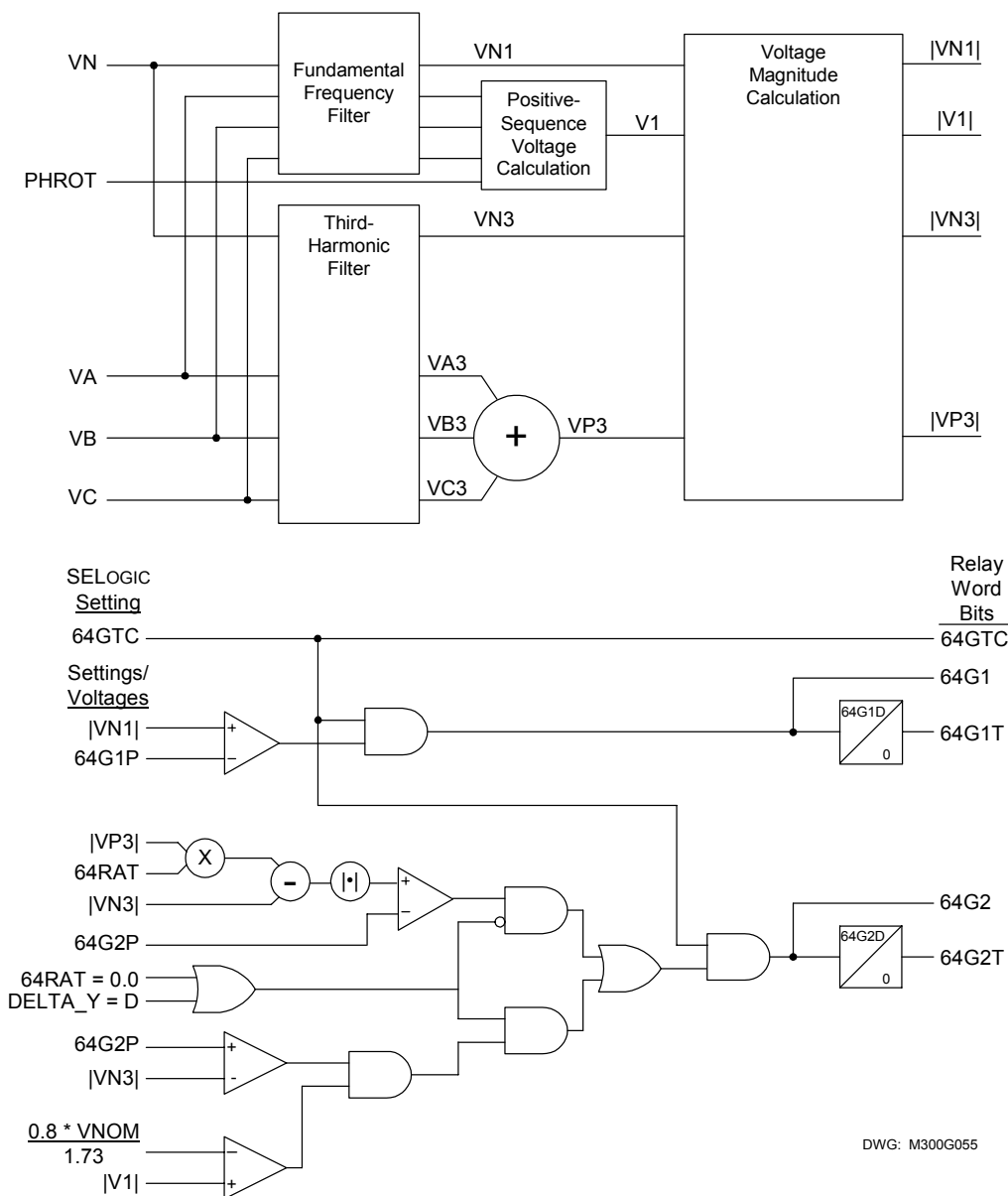
Figure 2.43: 64G Logic Diagram
