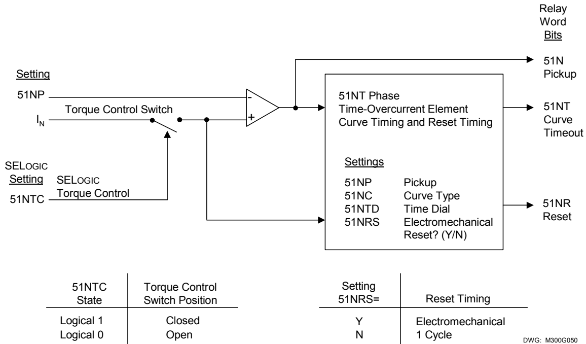
Figure 2.25: Neutral Ground Time-Overcurrent Element 51NT
