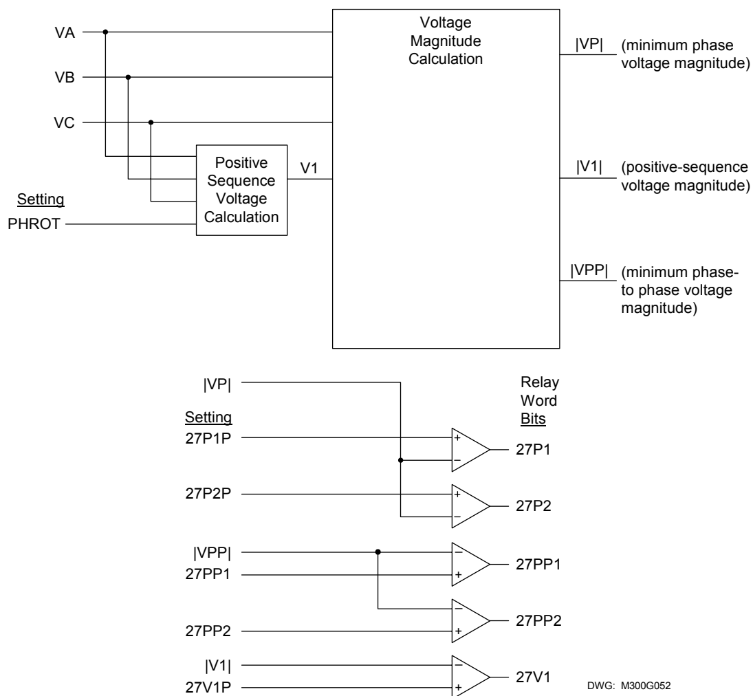
Figure 2.40: Undervoltage Element Logic Diagram
