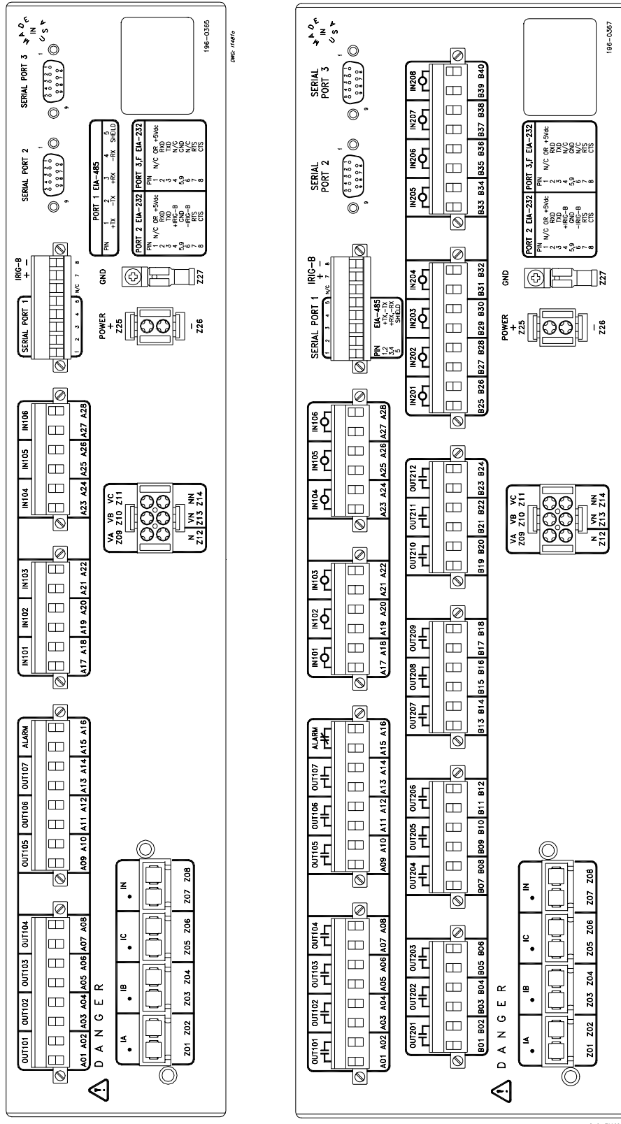
Figure 5.8: SEL300G0 Relay Rear-Panel Drawings for Rack- and Panel-Mount Relays (2U and 3U), Connectorized Version
