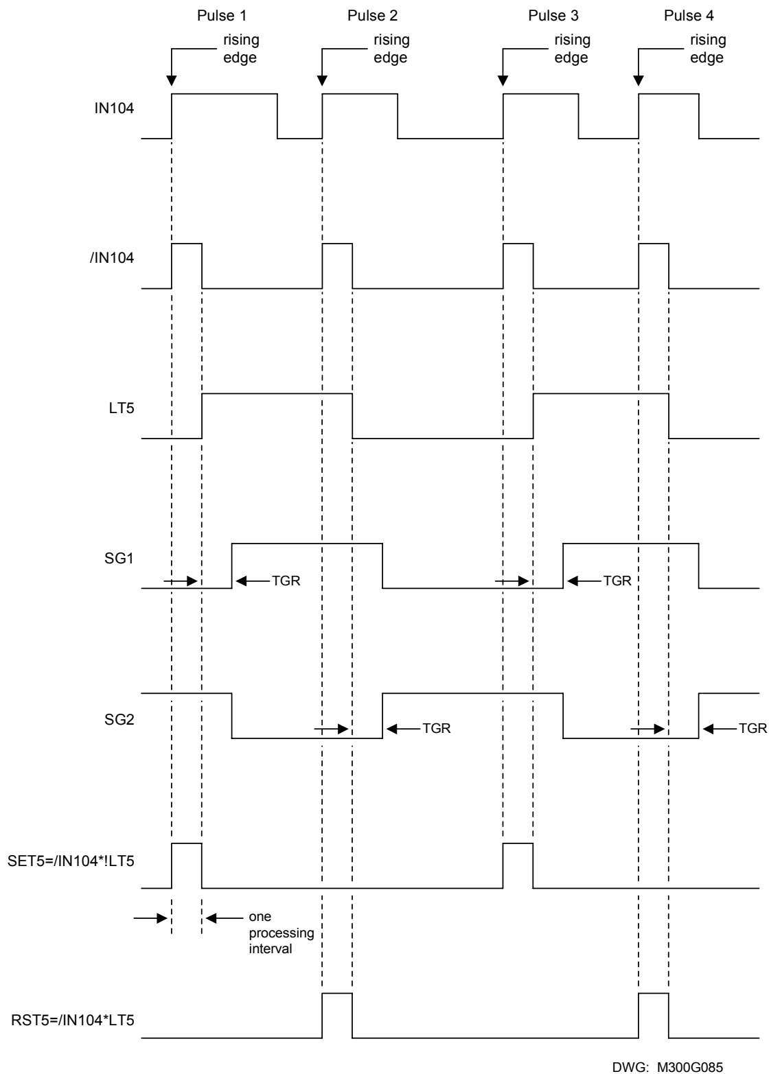
Figure 3.8: Latch Control Switch Operation Time Line
