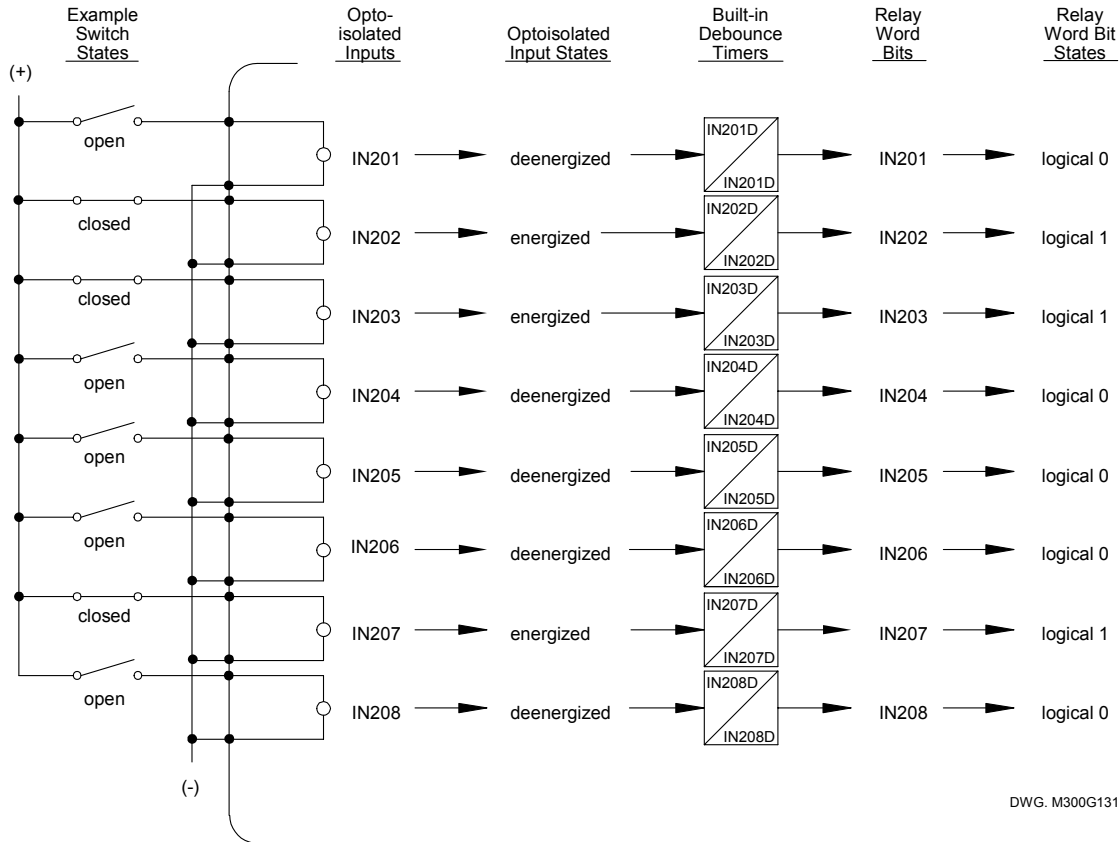
Figure 3.13: Example Operation of Optoisolated Inputs IN201 Through IN208 - Extra I/O Board (Models 0300G_1 and 0300G_Y)
