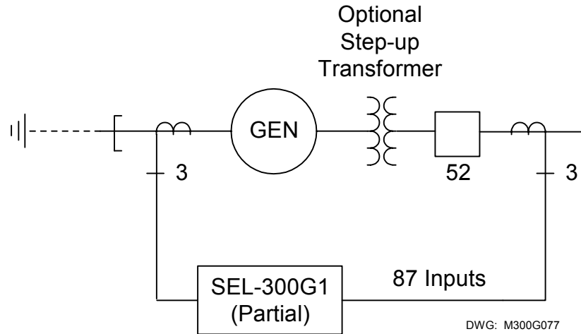
Figure 4.27: Generator/Breaker Topology Where SEL-300G1 Relay Offers Breaker Failure Protection
