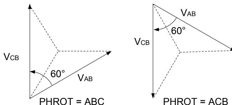
Figure 7.8: Open-Delta AC Potential Connection Test Voltage Signals
