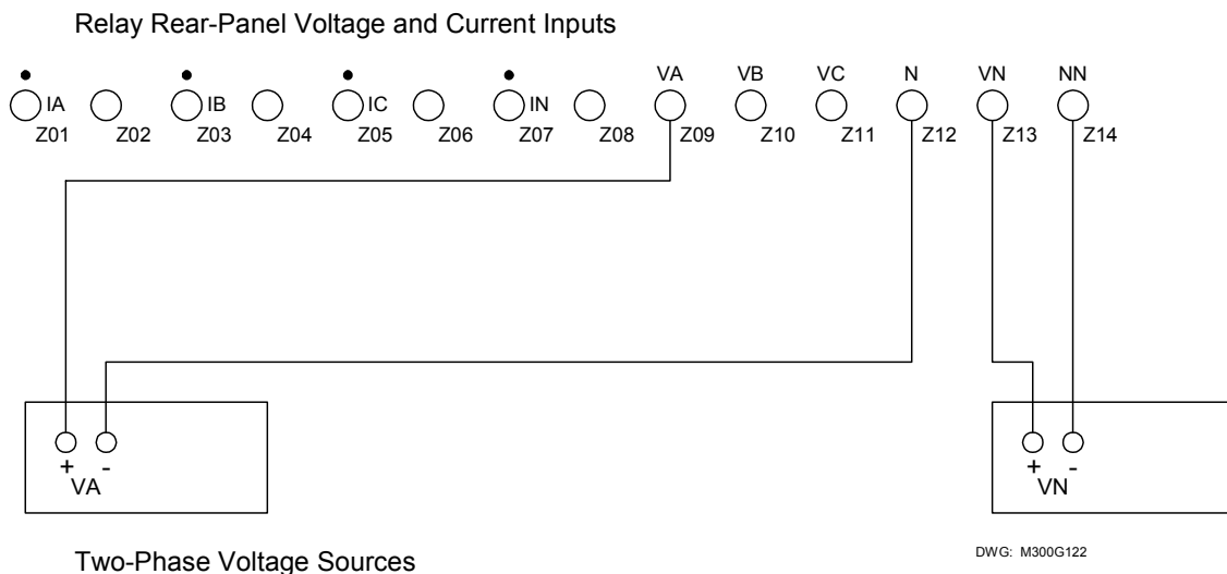
Figure 7.27: 64G2 Element Test Connections, 64RAT \neq 0
