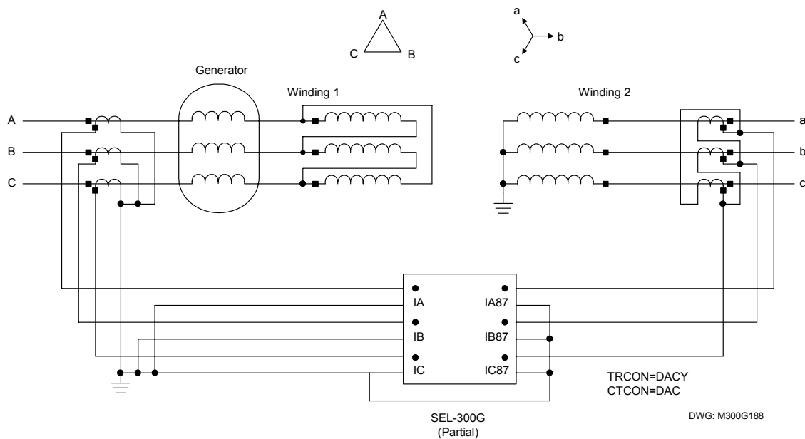
Figure B.4: Delta-Wye Power Transformer With Delta High-Side CT Connections
