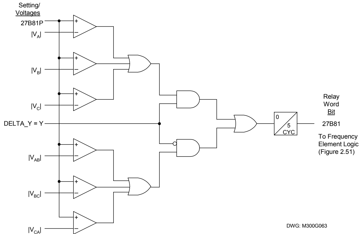
Figure 2.50: Frequency Element Voltage Supervision Logic
