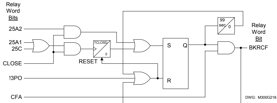
Figure 4.14: Breaker Close Failure Logic Diagram
