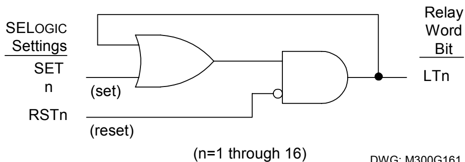
Figure 4.4: Latch Control Switches Drive Latch Bits LT1 Through LT16
