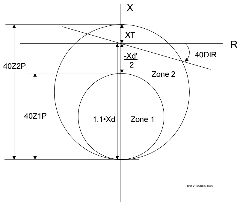
Figure 2.18: Loss-of-Field Element Operating Characteristic, Positive Zone 2 Offset
