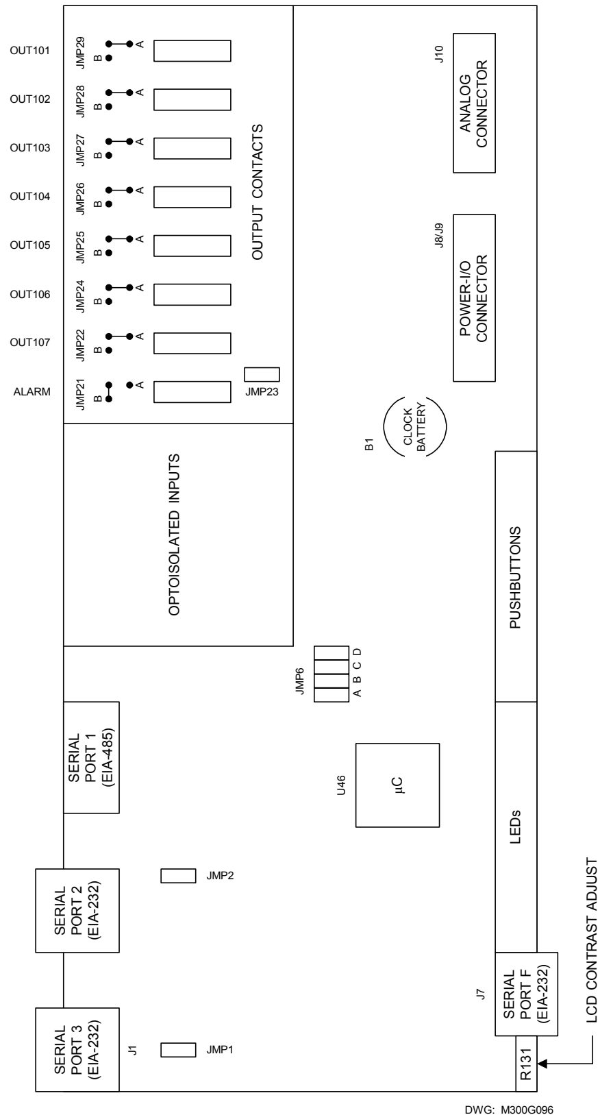
Figure 5.25: Jumper, Connector, and Major Component Locations on the SEL-300G Relay Main Board (All Models)
