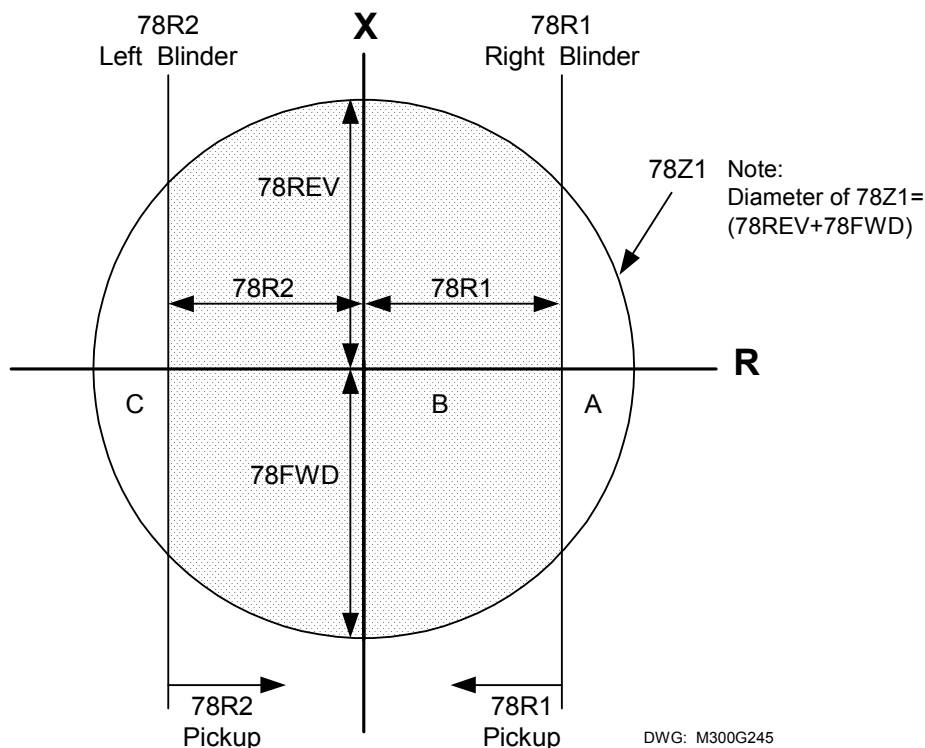
Figure 2.44: Single Blinder Scheme Operating Characteristics
