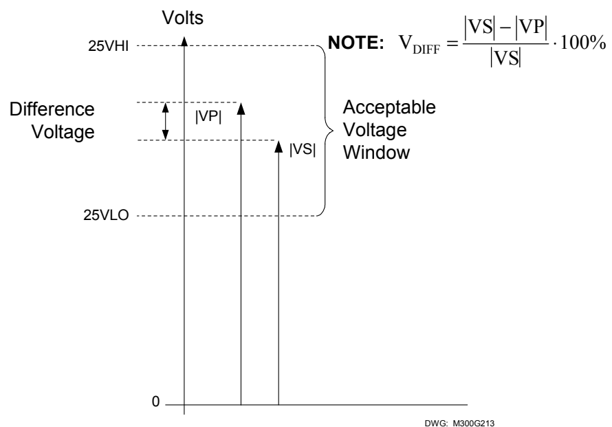
Figure 4.11: Synch-Check Function Voltage Element Characteristic
