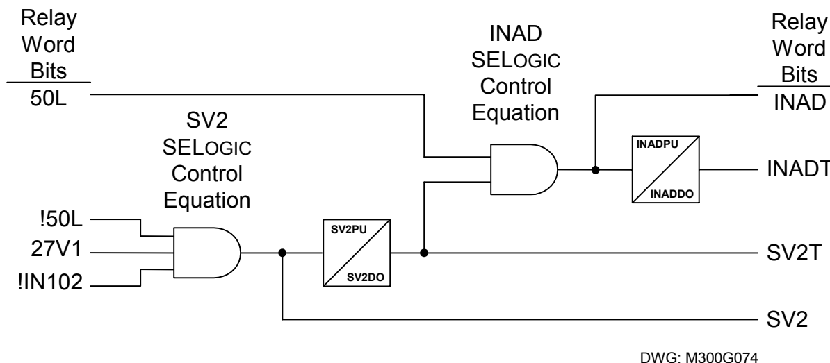
Figure 4.26: Inadvertent Energization Logic Diagram
