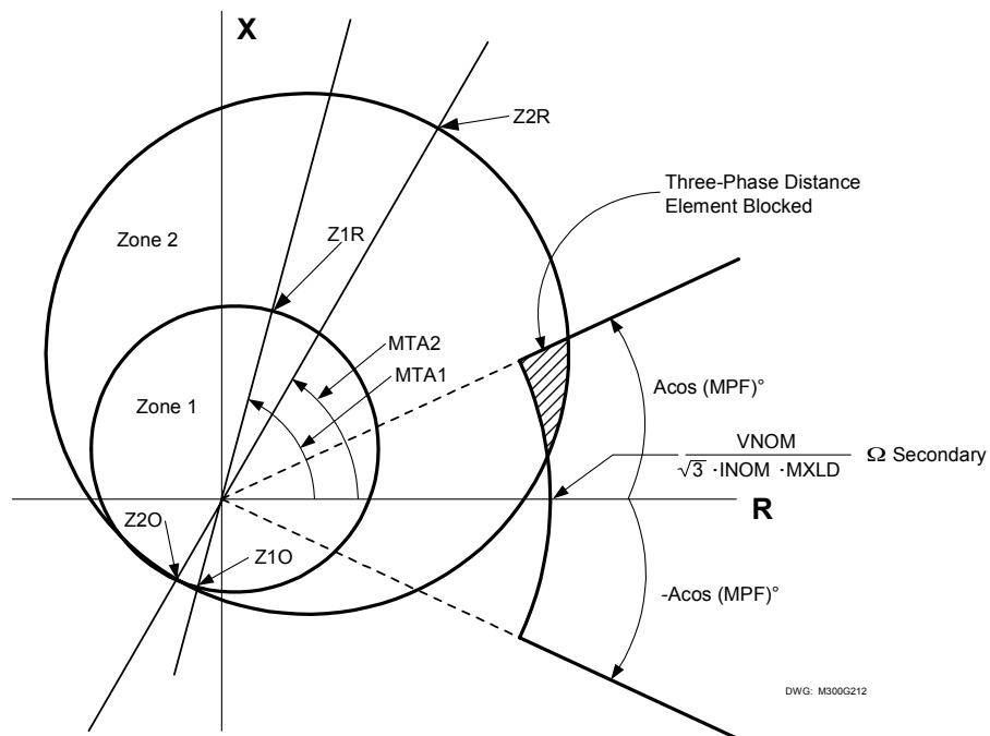
Figure 2.5 Distance Element Operating Characteristics
