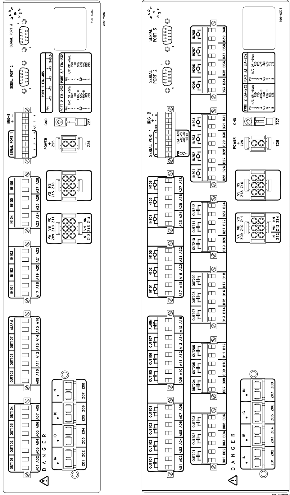
Figure 5.10: SEL-300G2 Relay Rear-Panel Drawings for Rack- and Panel-Mount Relays (2U and 3U), Connectorized Version
