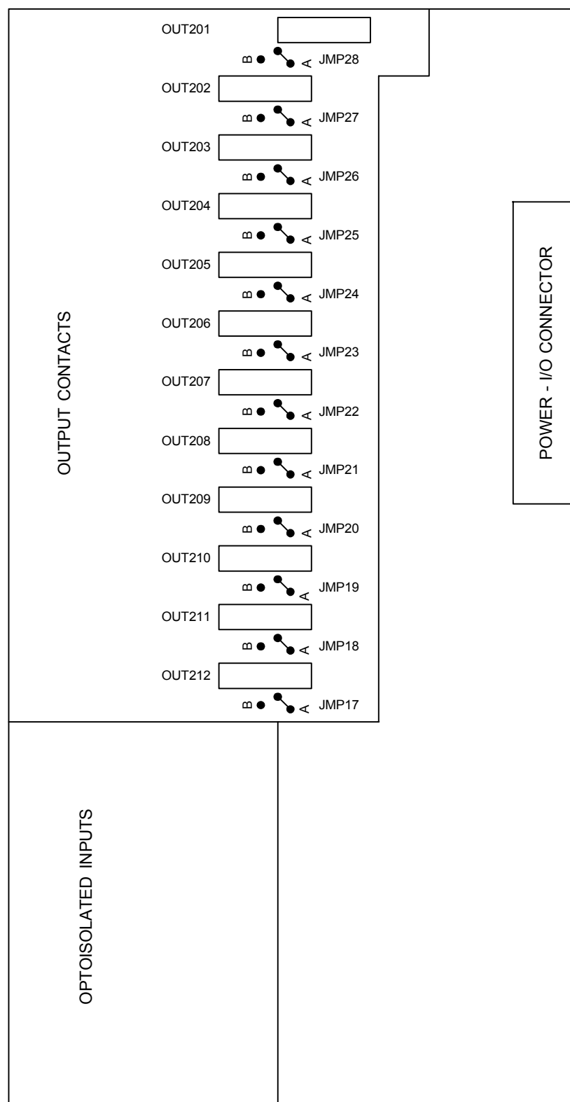
Figure 5.26: Jumper, Connector, and Major Component Locations on the SEL-300G Relay Extra I/O Board (Models 0300G_1 and 0300G_Y)
