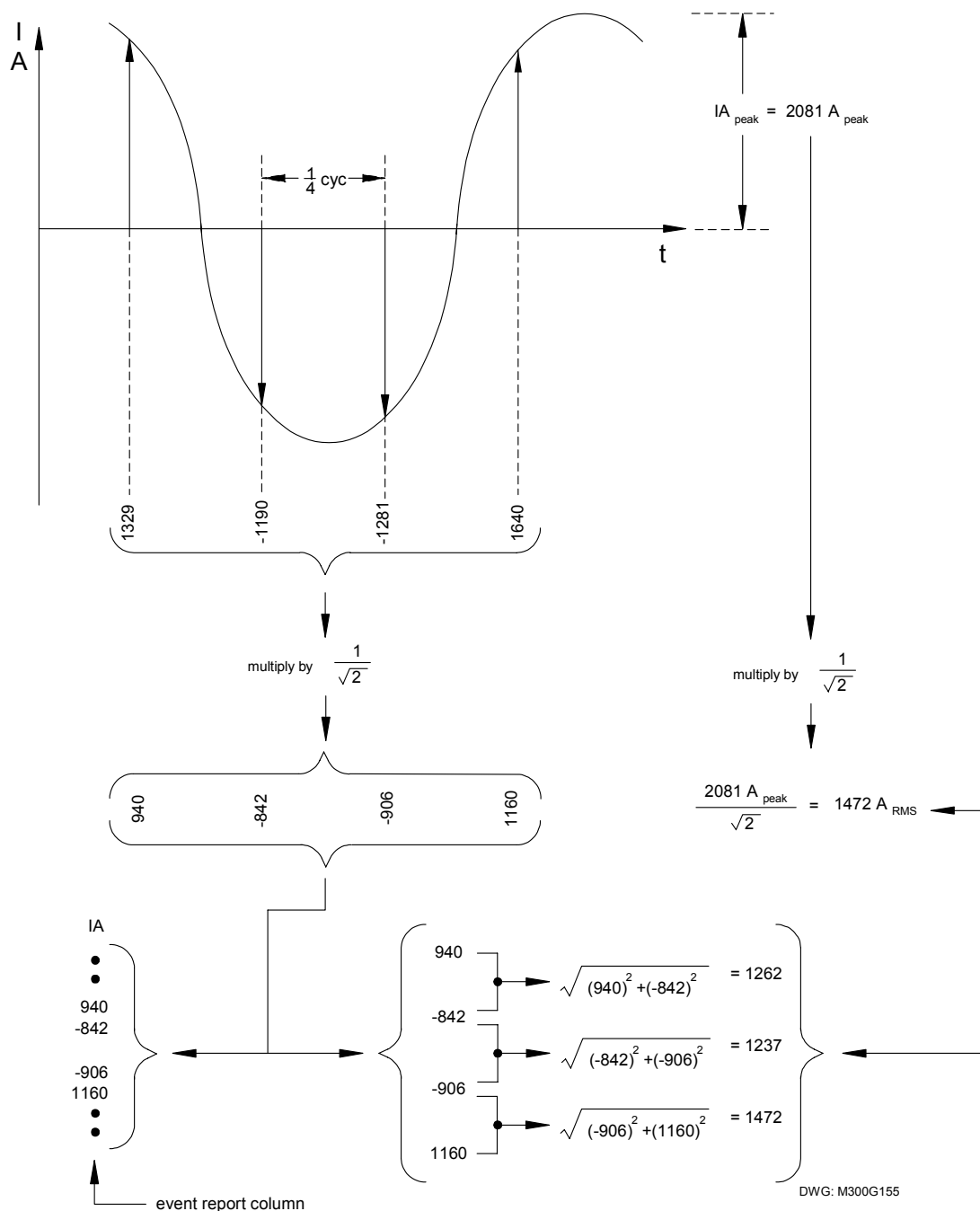
Figure 11.3: Derivation of Event Report Current Values and RMS Current Values From Sampled Current Waveform
