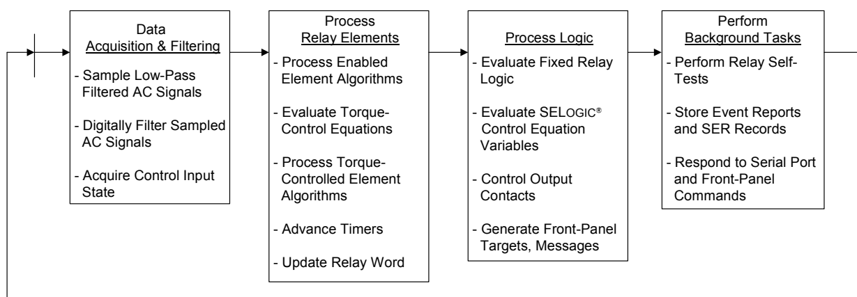
Figure 2.1: Relay Processing Order
