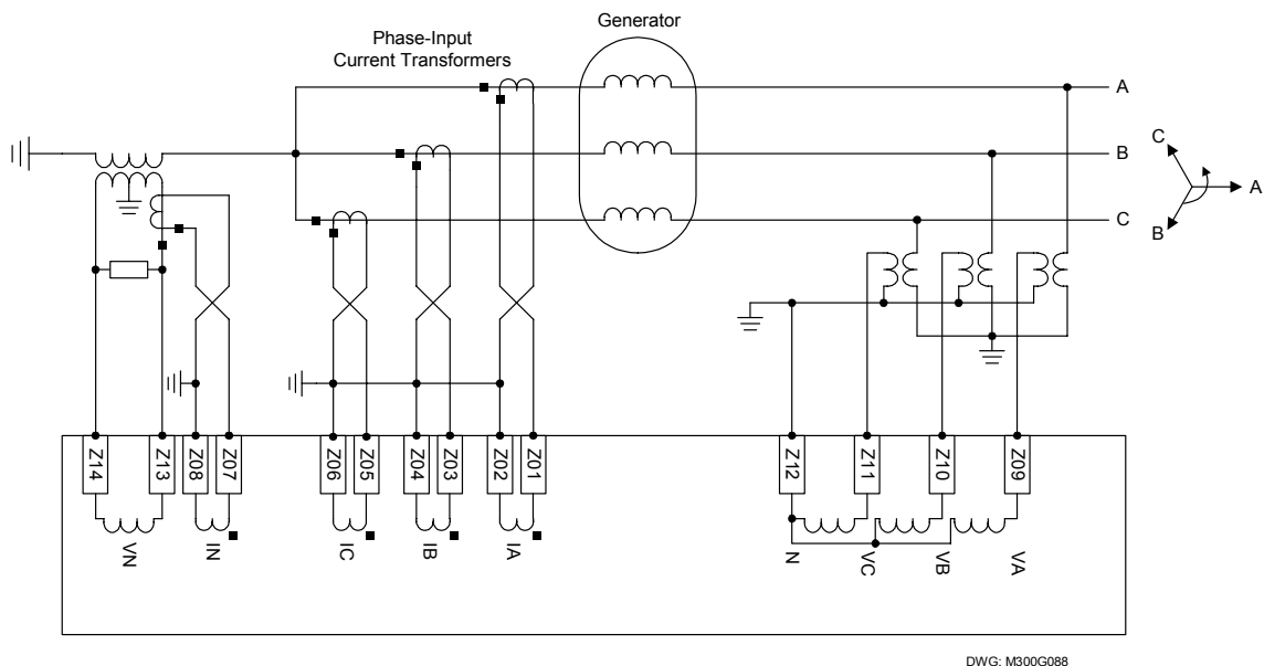
Figure 5.14: SEL-300G0 Relay AC Connection Example — High-Impedance Grounded Generator Without Current Differential Protection
