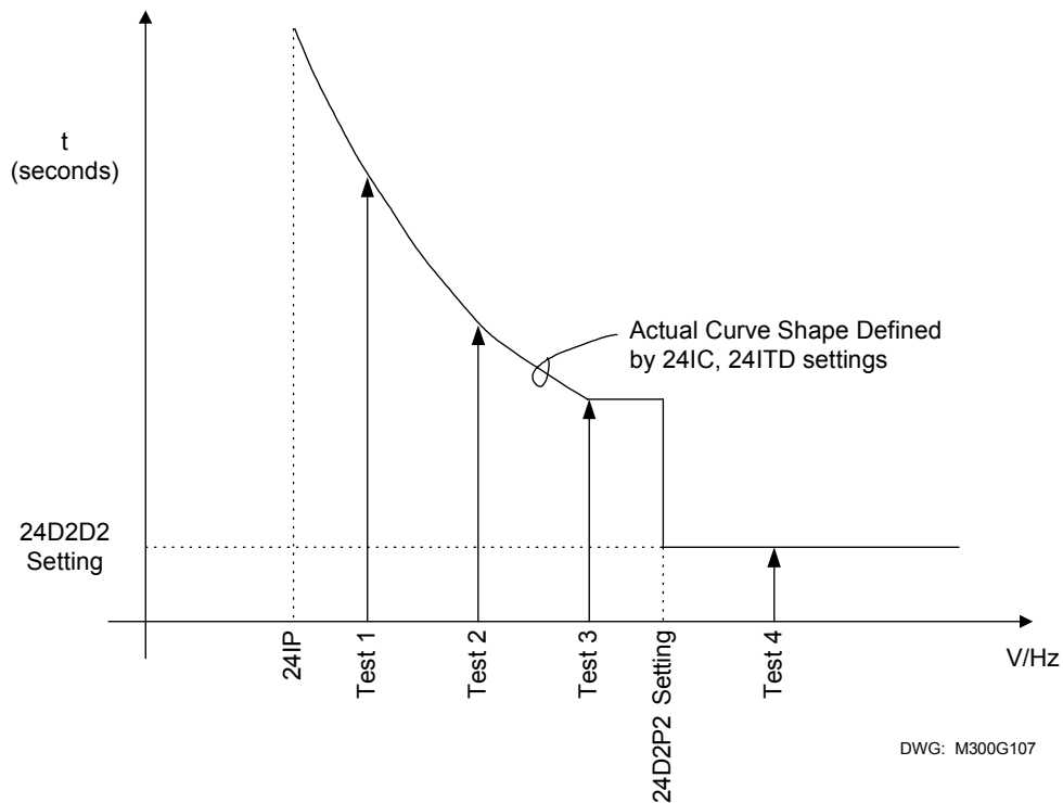
Figure 7.15: 24C2 Time-Delay Test Points, 24CCS = ID
