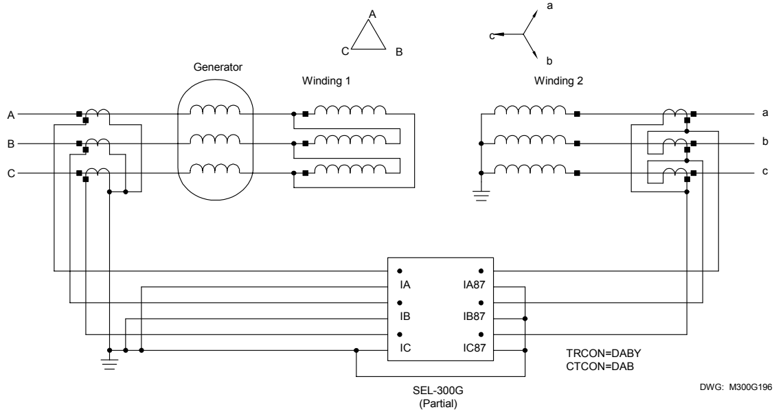
Figure B.5: Delta-Wye Power Transformer With Delta High-Side CT Connections
