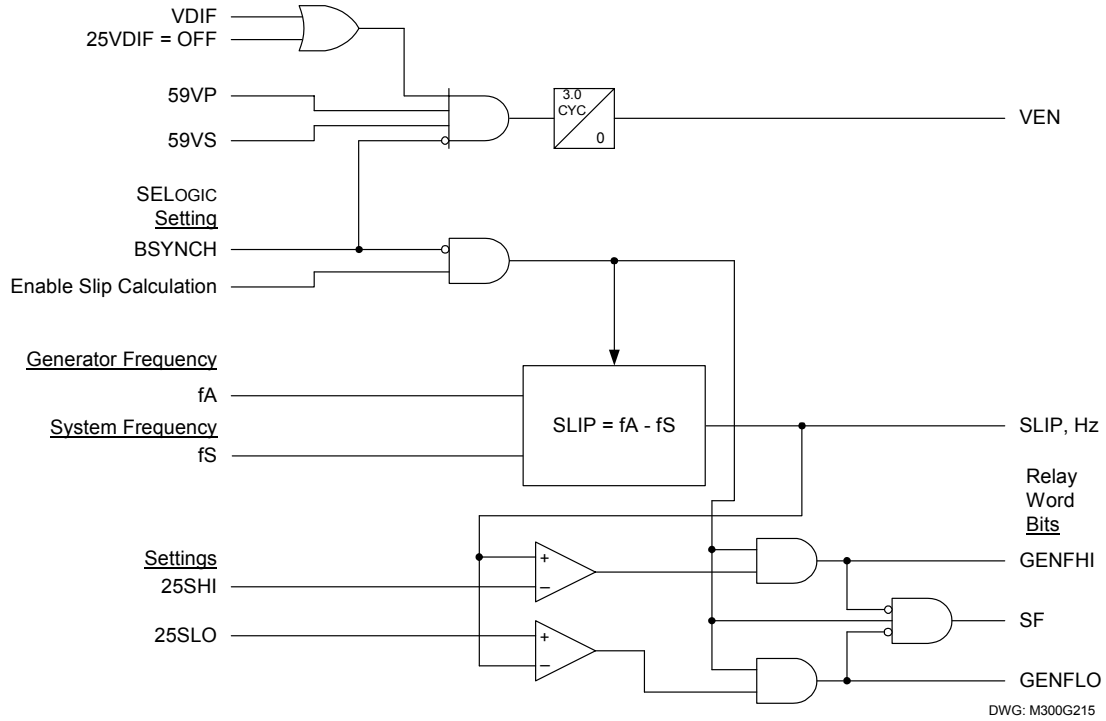
Figure 4.12 Synch-Check Function Slip Elements
