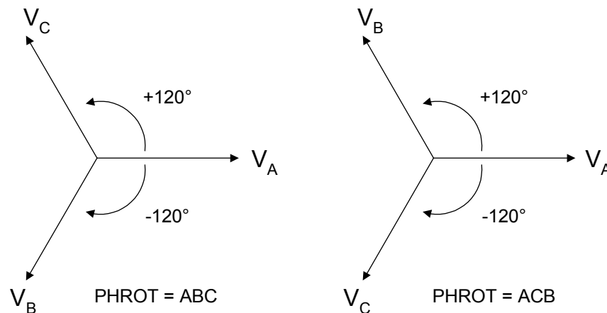
Figure 7.7: Three-Phase AC Connection Test Voltage Signals
