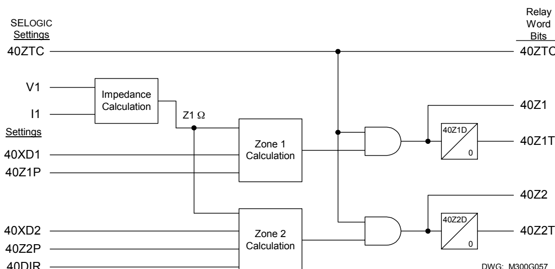
Figure 2.16: Loss-of-Field Logic Diagram
