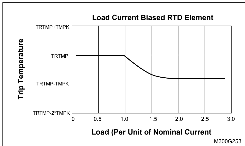
Figure 2.54: Winding RTD Trip Characteristics with BLMT = 2.00
