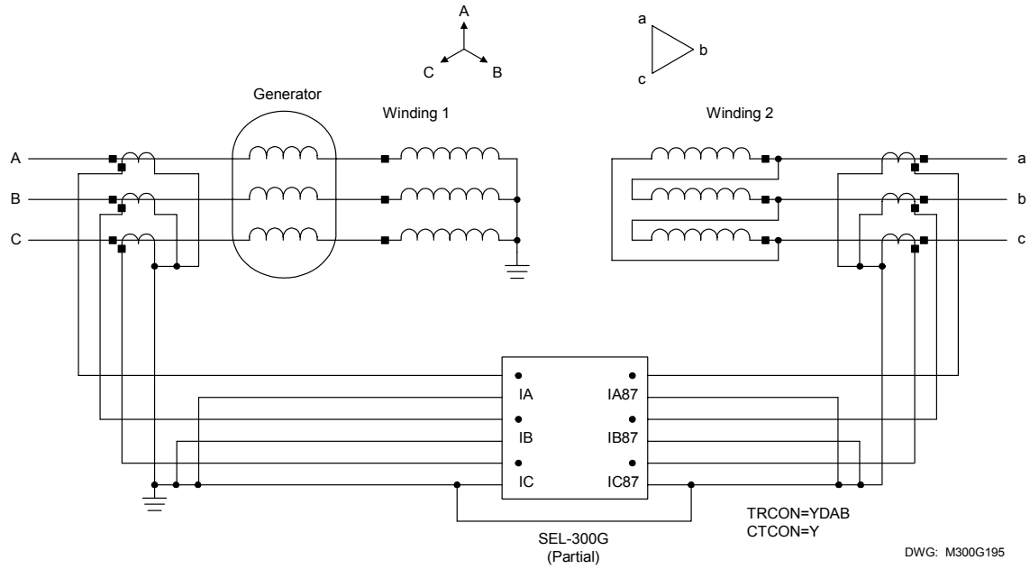
Figure B.9: Wye-Delta Power Transformer With Wye High-Side Connections
