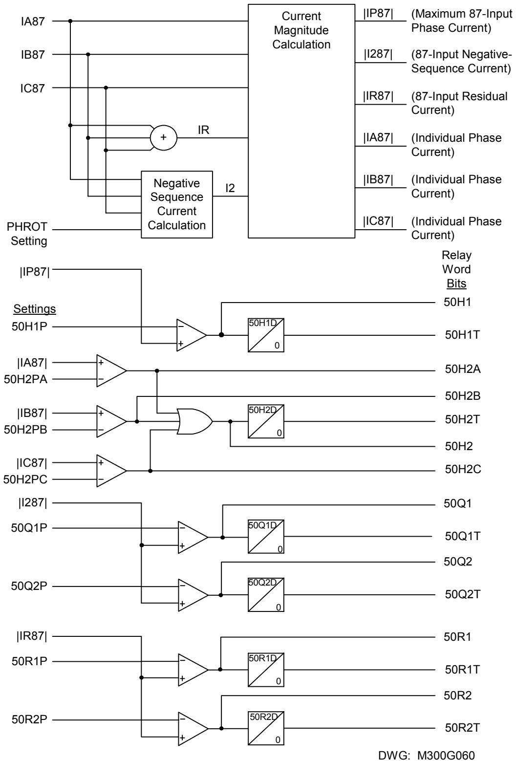
Figure 2.24: 87-Input Definite-Time Overcurrent Element Logic Diagram
