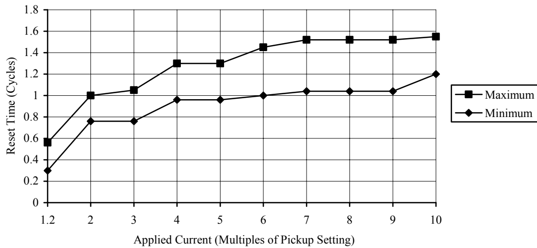
Figure 2.22: Instantaneous Overcurrent Element Reset Time Curve
