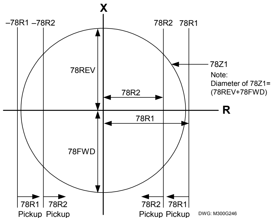
Figure 2.47: Double Blinder Scheme Operating Characteristics
