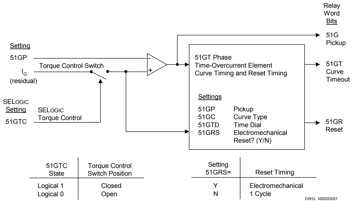
Figure 2.26: Residual Ground Time-Overcurrent Element 51GT
