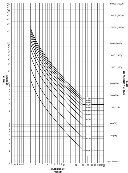
Figure 2.35: I.E.C. Long-Time Inverse Curve: C4
