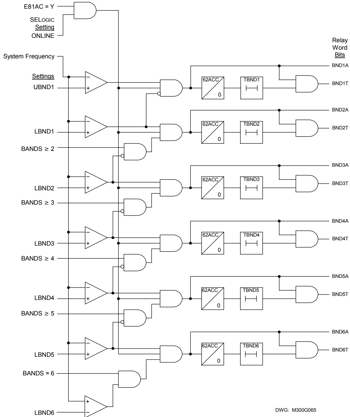
Figure 2.53: Abnormal Frequency Protection Logic Diagram
