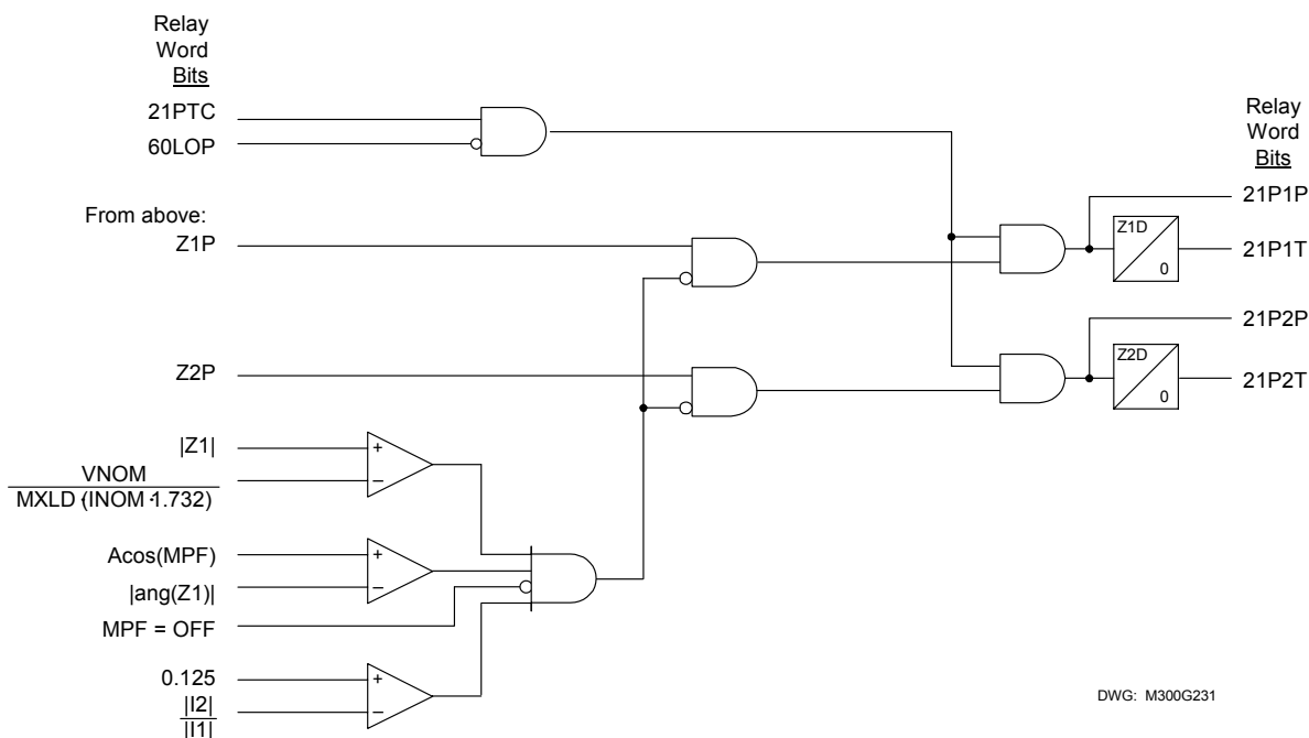
Figure 2.7: Phase Distance Element Logic
