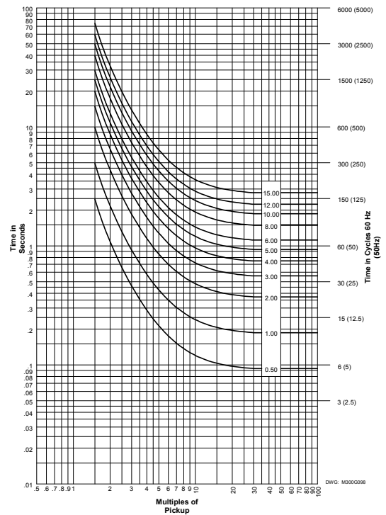
Figure 2.28: U.S. Inverse Curve: U2
