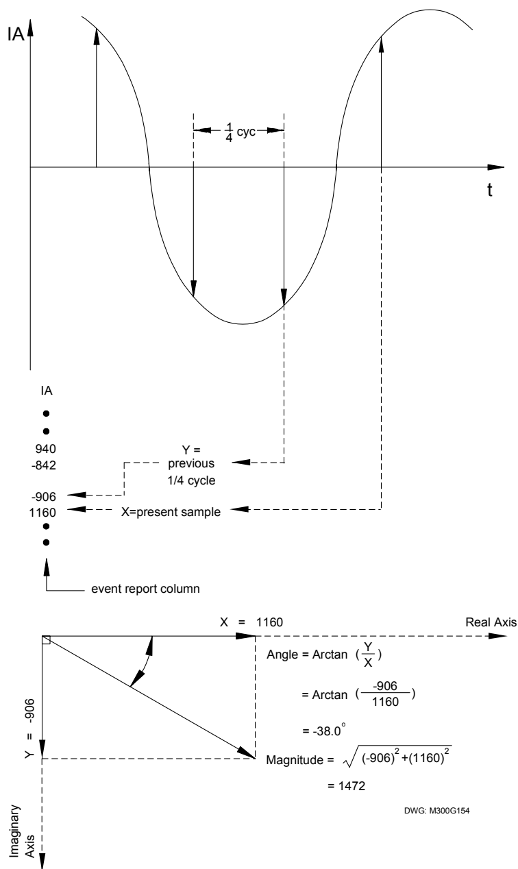
Figure 11.4: Derivation of Phasor RMS Current Values From Event Report Current Values
