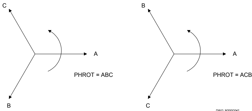
Figure 2.4: Phase Rotation Settings
