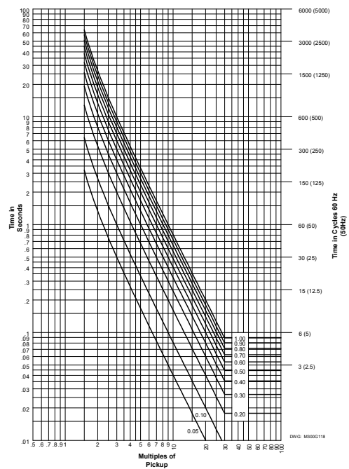
Figure 2.34: I.E.C. Class C Curve (Extremely Inverse): C3
