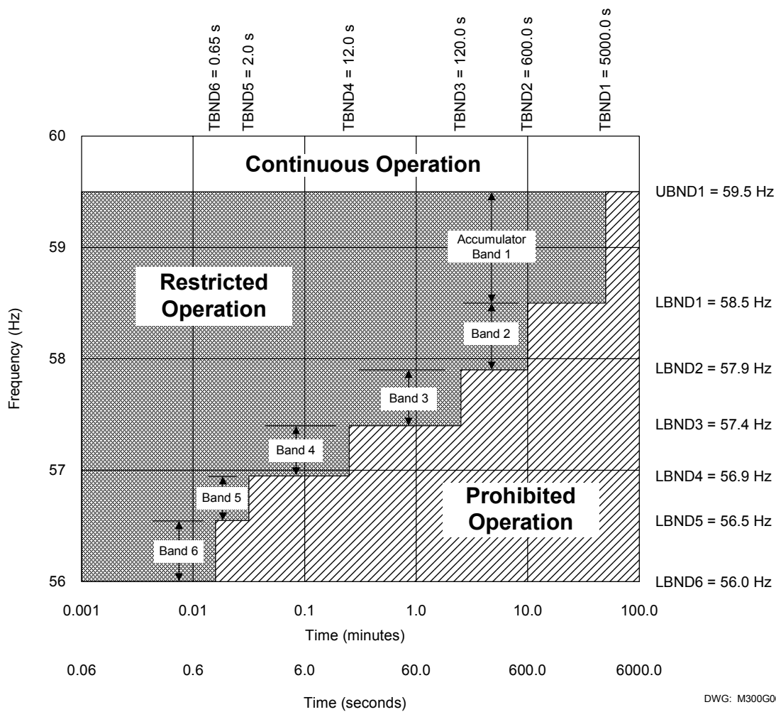
Figure 2.52: Example Turbine Operating Limitations During Abnormal Frequency
