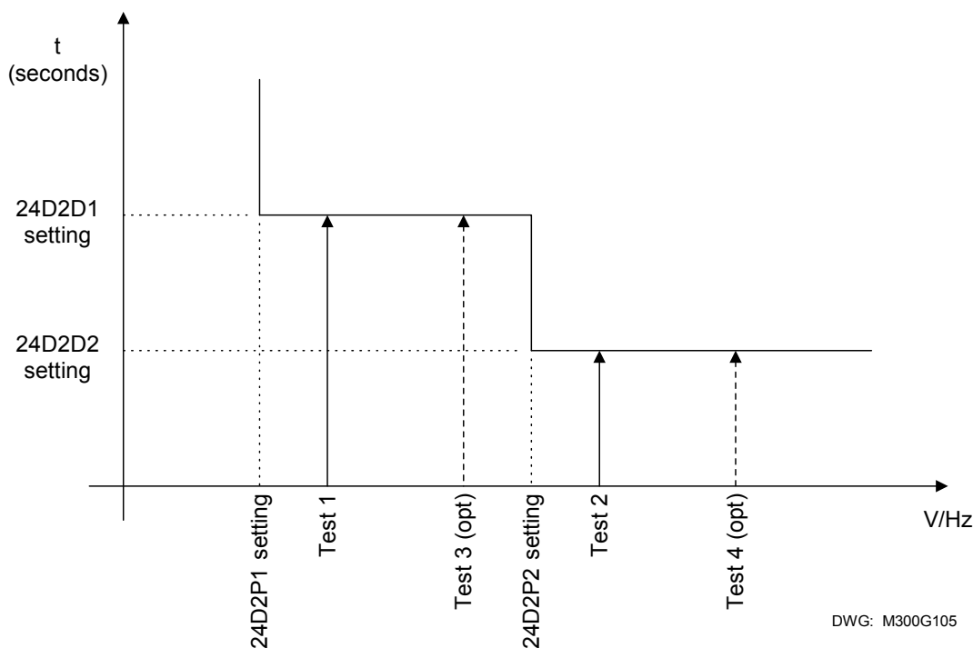
Figure 7.13: 24C2 Time-Delay Test Points, 24CCS = DD
