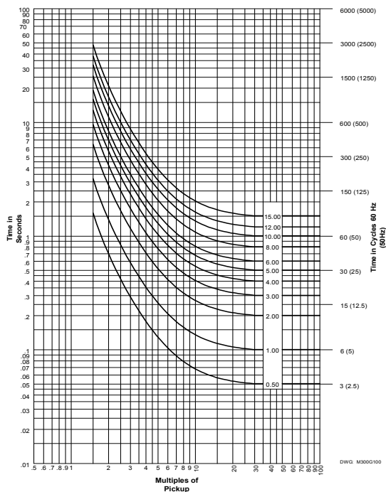
Figure 2.29: U.S. Very Inverse Curve: U3
