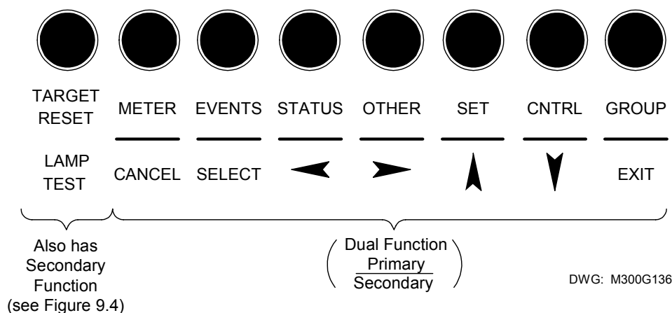
Figure 9.1: SEL-300G Relay Front-Panel Pushbuttons – Overview
