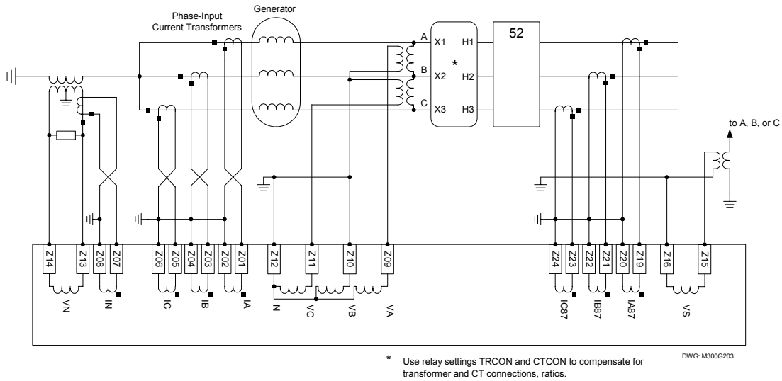
Figure 5.23: SEL-300G3 Relay AC Connection Example - High-Impedance Grounded Generator With Open-Delta PTs, Step-Up Transformer Included in Differential Zone, and Synch-Check
