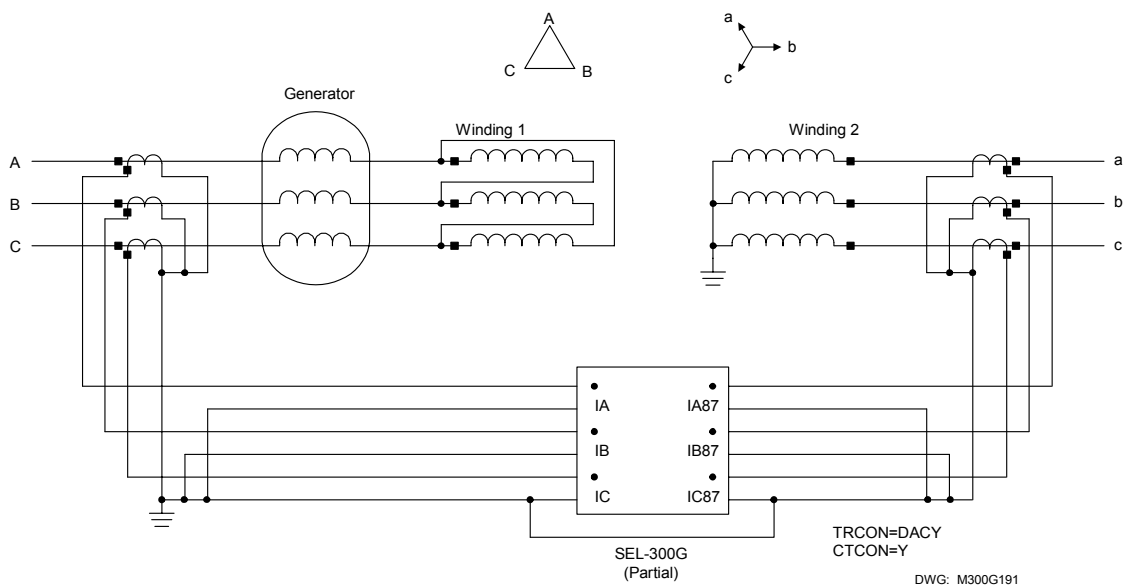
Figure B.2: Delta-Wye Power Transformer With Wye High-Side CT Connections
