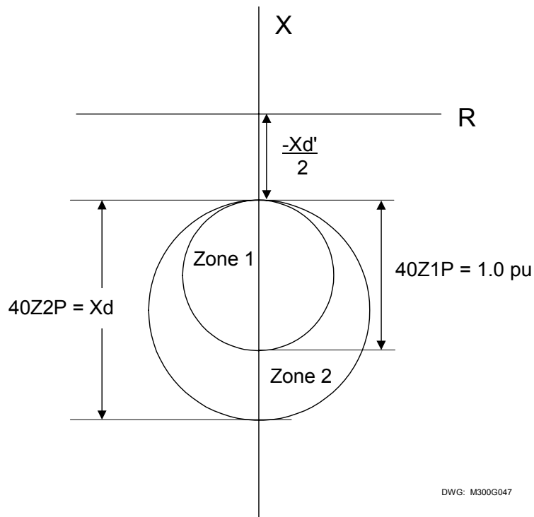
Figure 2.17: Loss-of-Field Element Operating Characteristic, Negative Zone 2 Offset
