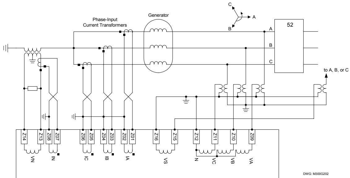
Figure 5.20: SEL-300G2 Relay High-Impedance Grounded Generator With Synch-Check and Without Current Differential Protection
