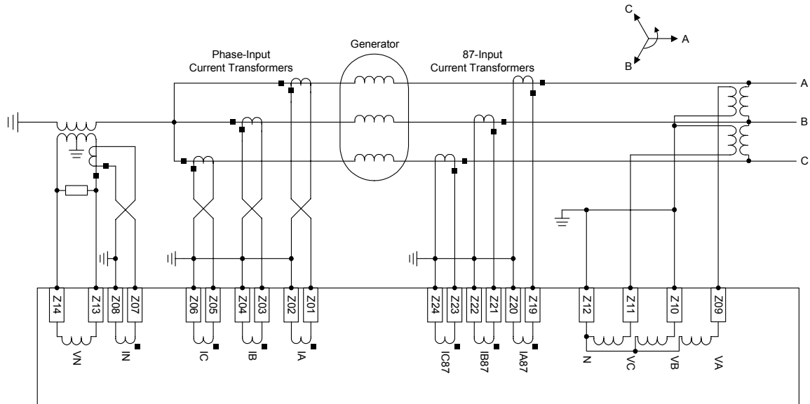
Figure 5.19: SEL-300G1 Relay Applied Using Open-Delta Potentials
