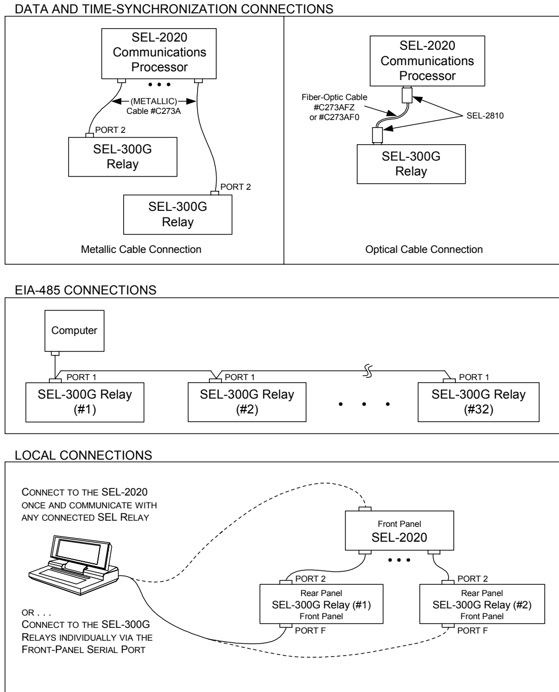
Figure 1.5: SEL-300G Relay Communication Connection Examples
