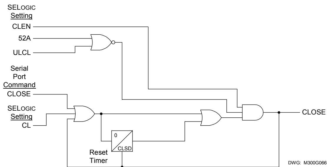
Figure 4.8: Close Logic
