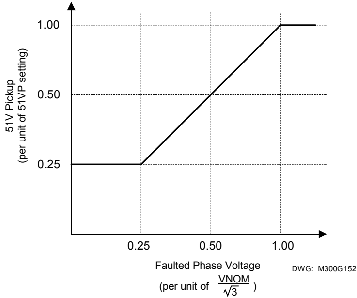
Figure 2.39: 51V Element Voltage Restraint Characteristic
