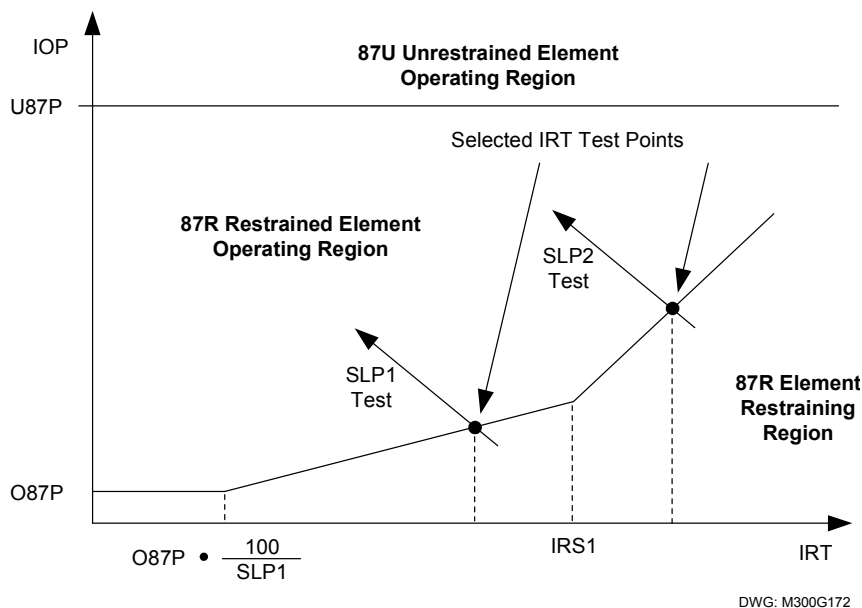
Figure 7.32: Percentage Restraint Differential Characteristic
