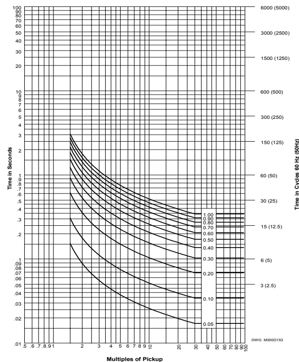
Figure 2.36: I.E.C. Short-Time Inverse Curve: C5
