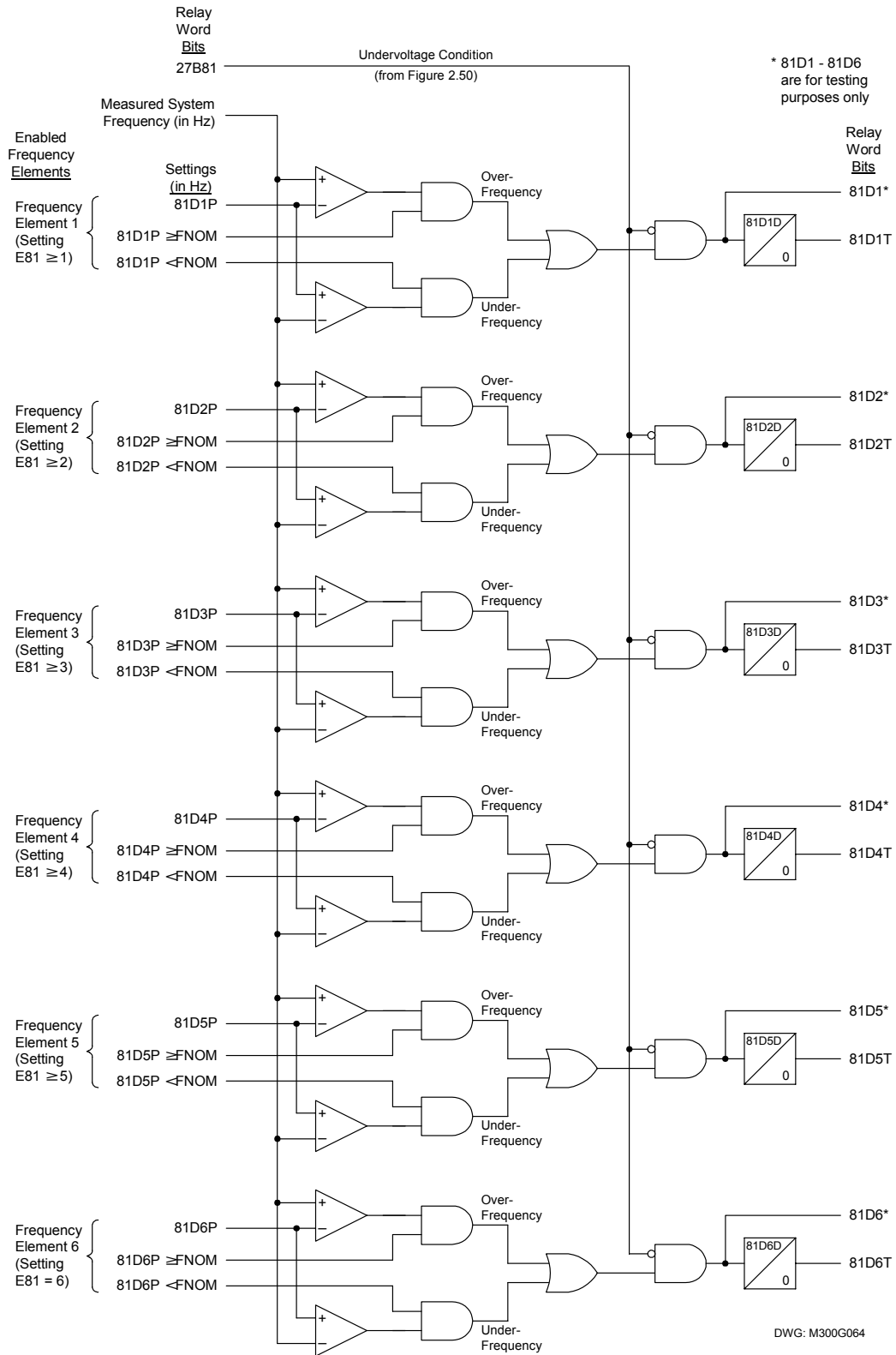
Figure 2.51: Frequency Element Logic
