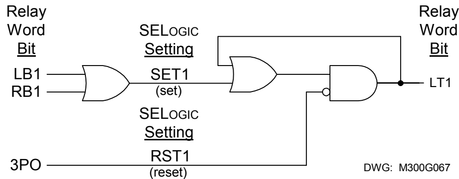
Figure 4.5: Latch Control Switch to Shut Down Generator
