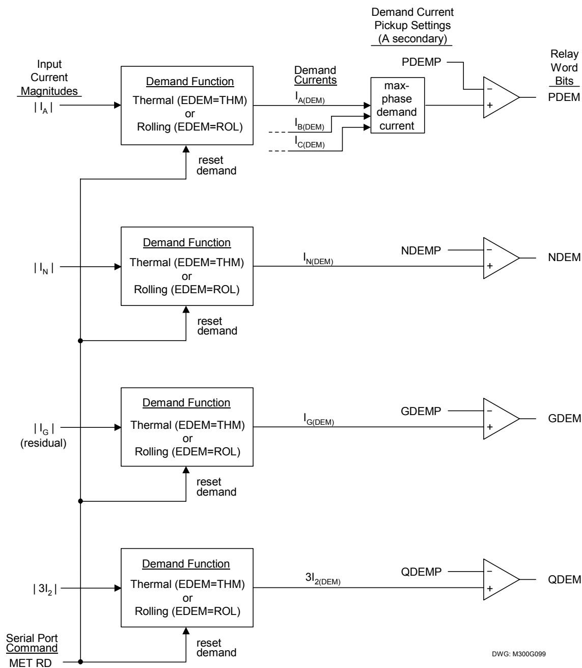
Figure 3.3: Demand Current Logic Outputs
