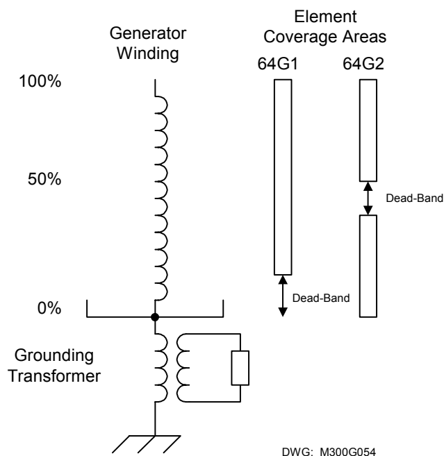
Figure 2.42: 64G Element Operating Characteristic
