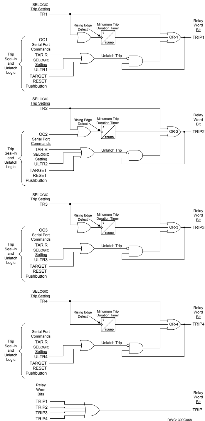
Figure 4.6: Trip Logic
