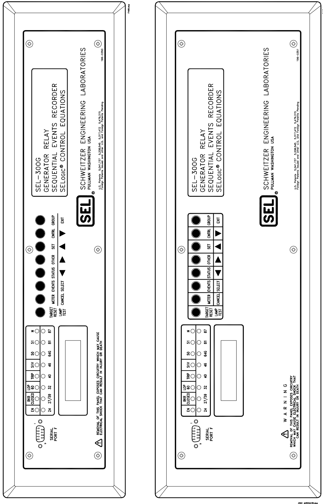
Figure 5.3: SEL-300G Relay Front-Panel Drawings for Panel-Mount Relays (2U and 3U), Screw-Terminal Block, and Connectorized Versions
