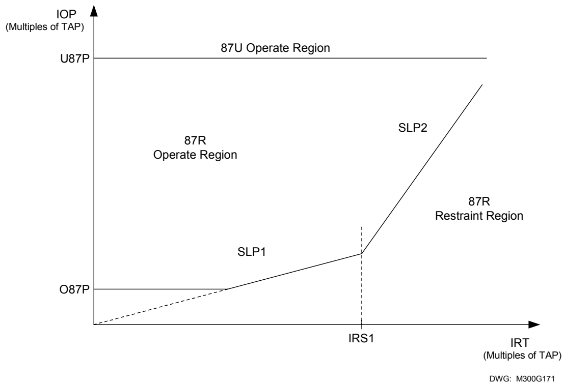
Figure 13.8: Differential Element Operating Characteristics
