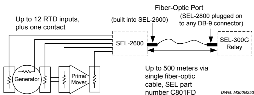
Figure 1.4: Generator Thermal Protection with SEL-2600 & SEL-300G Relay
