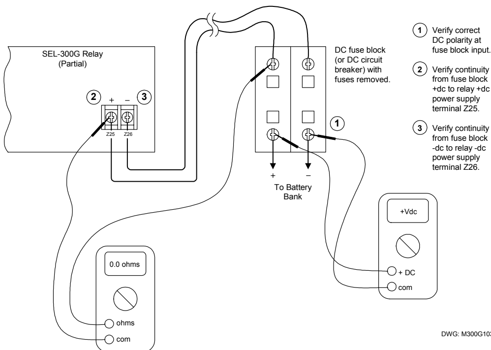
Figure 7.6: DC Supply Polarity, Continuity Checks
