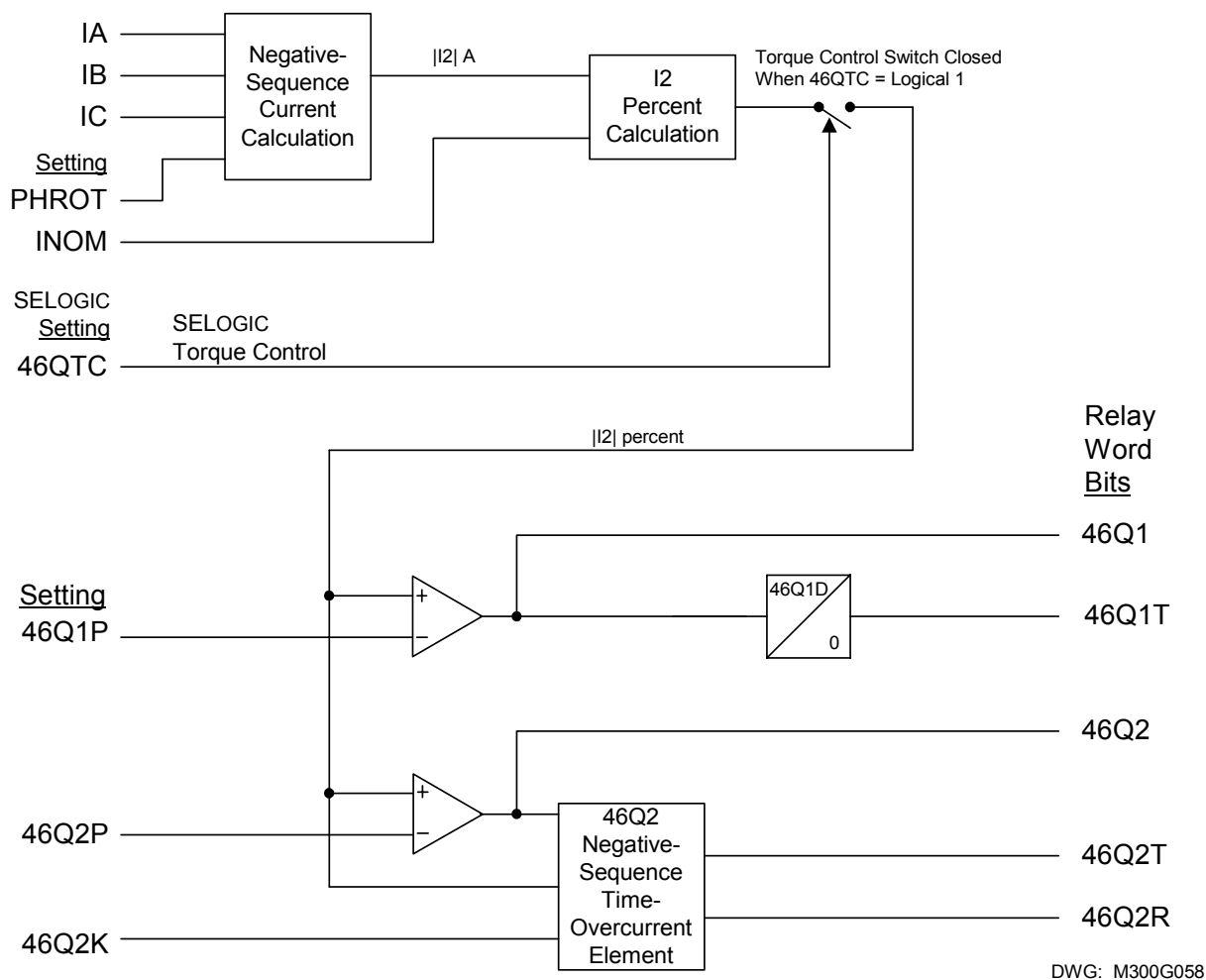
Figure 2.19: Negative-Sequence Overcurrent Element Logic Diagram
