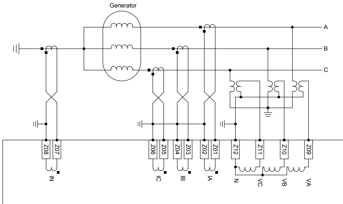
Figure 5.17: SEL-300G0 Relay AC Connection Example — Solidly Grounded Generator With Ground Differential Protection (87N)
