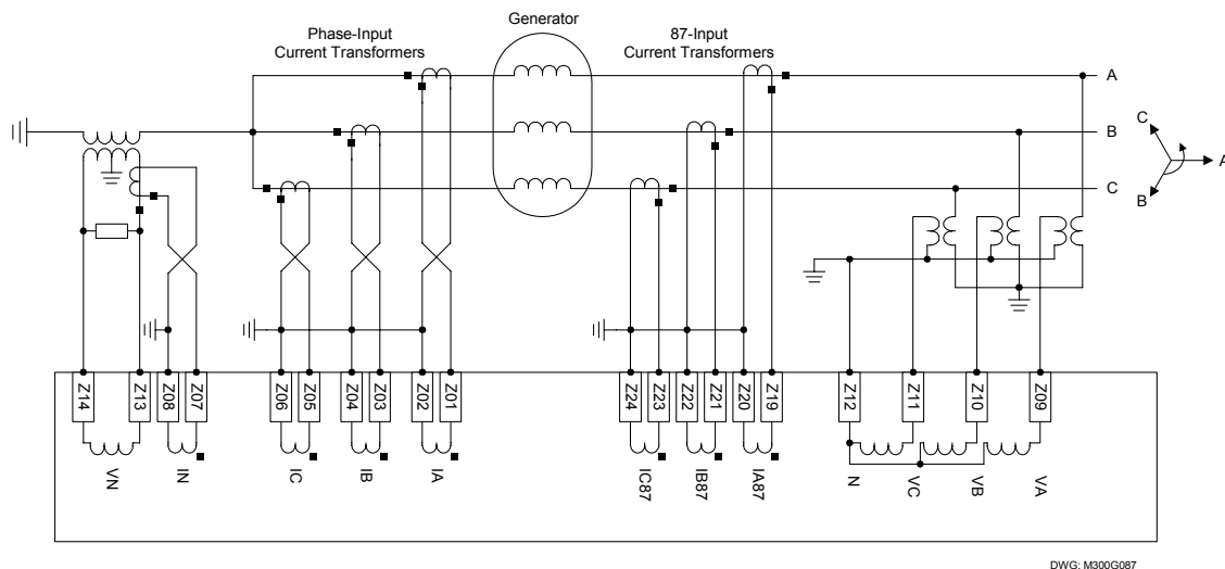
Figure 5.13: SEL-300G1 Relay AC Connection Example — High-Impedance Grounded Generator With Current Differential Protection
