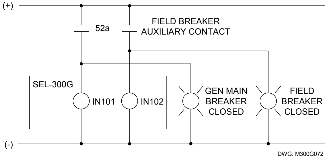
Figure 4.24: Traditional Panel Light Installations
