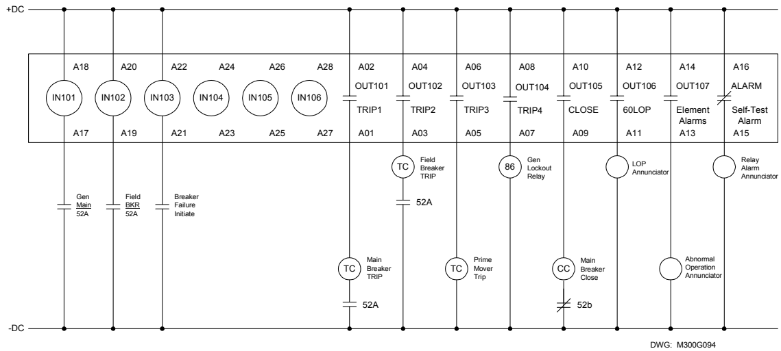
Figure 5.24: SEL-300G Relay DC Connection Example
