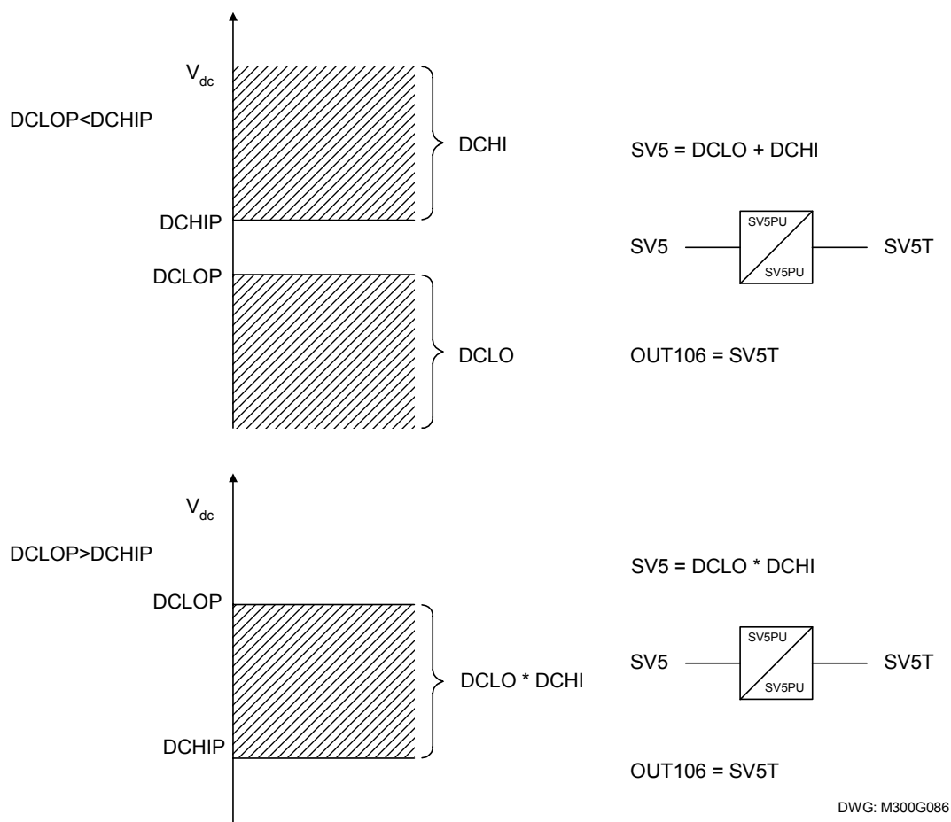
Figure 3.5: Create DC Voltage Elements with SELogic Control Equations
