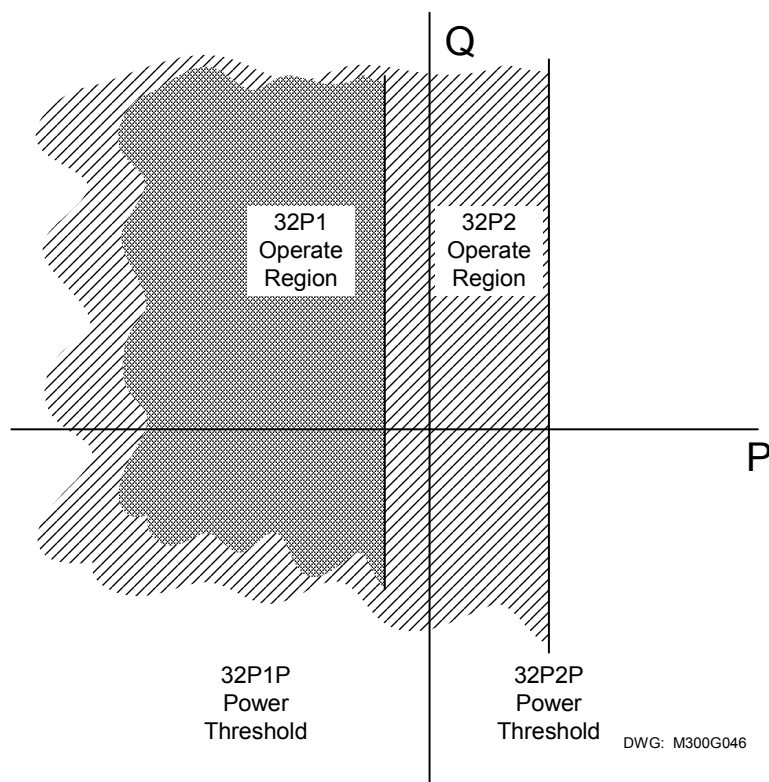
Figure 2.14: Reverse/Low-Forward Power Element Operating Characteristic
