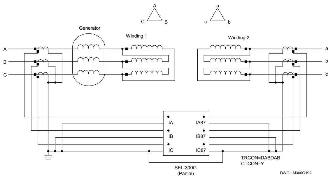
Figure B.7: Delta-Delta Power Transformer With Wye High-Side Connections
