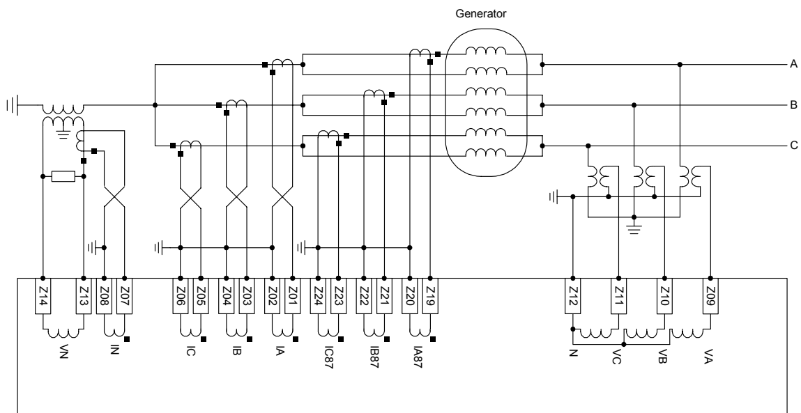
Figure 5.18: SEL-300G1 Relay AC Connection Example — High-Impedance Grounded Generator With Split-Phase Current Differential Protection
