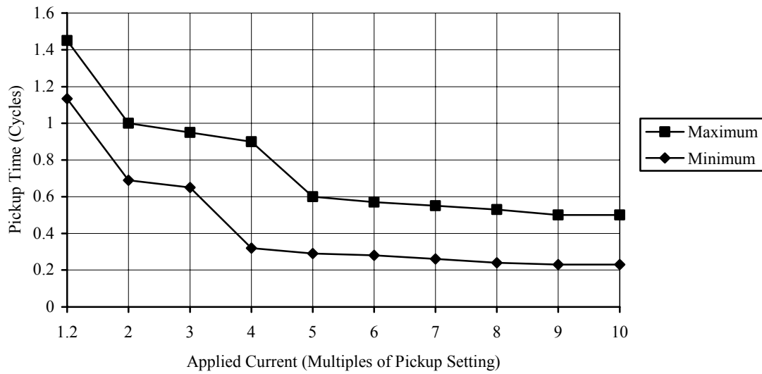
Figure 2.21: Instantaneous Overcurrent Element Pickup Time Curve
