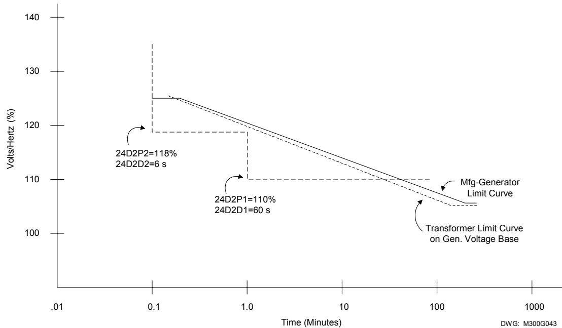
Figure 2.8: Dual-Level Volts/Hertz Time-Delay Characteristic, 24CCS=DD
