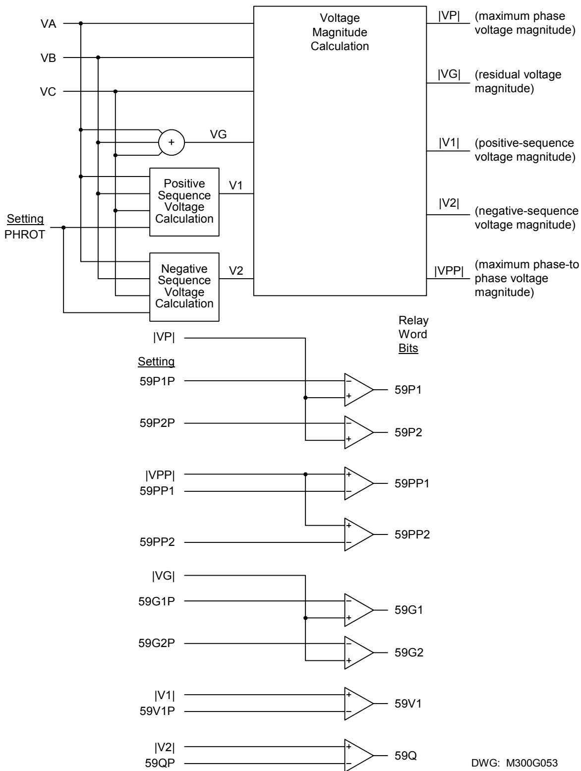
Figure 2.41: Overvoltage Element Logic Diagram
