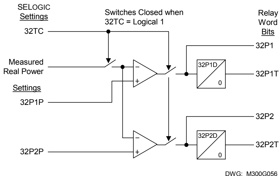
Figure 2.15: Reverse/Low-Forward Power Element Logic Diagram
