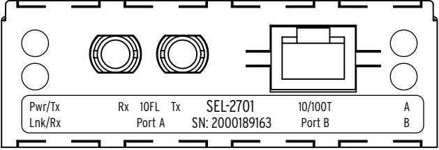
Figure 2.7 10BASE-FL and 10/100BASE-T Port Configuration.
