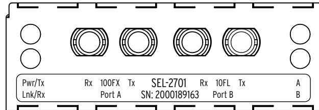
Figure 2.9 100BASE-FX and 10BASE-FL Port Configuration.
