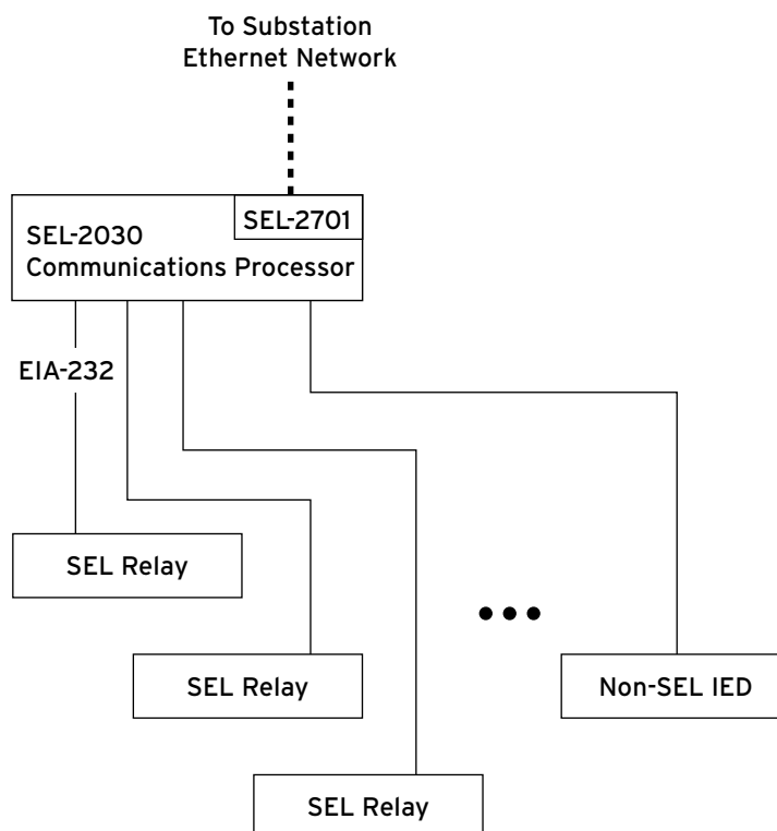
Figure 1.3 SEL Relays on Ethernet Network Using the SEL-2030.
