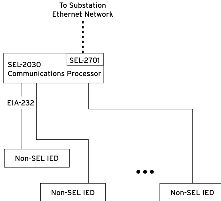
Figure 1.4 Non-SEL EIA-232 IEDs on Ethernet Network Using the SEL-2030.
