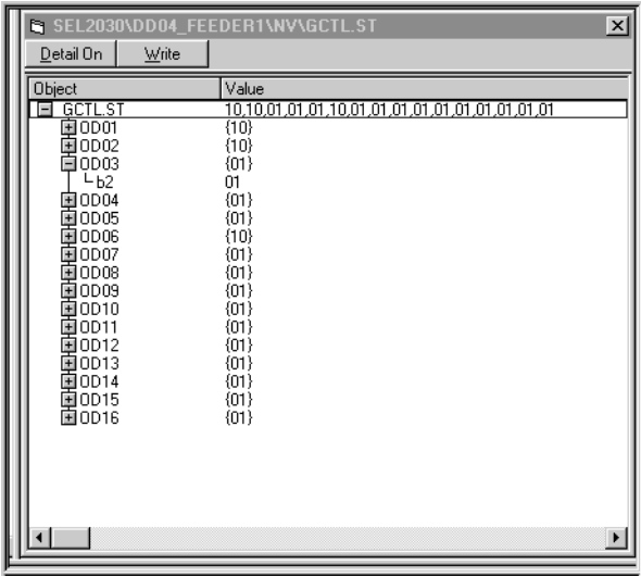
Figure C.6 GCTL Model With RB3 ST (status) Point.
