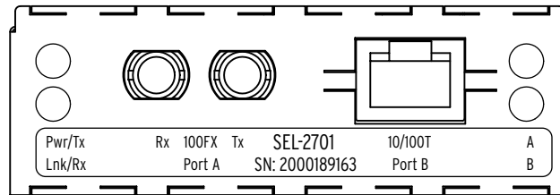
Figure 2.8 100BASE-FX and 10/100BASE-T Port Configuration.
