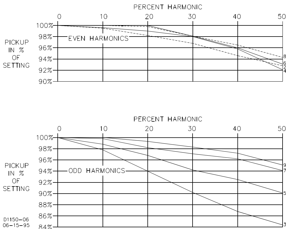
Figure 1-2. Harmonic Rejection
