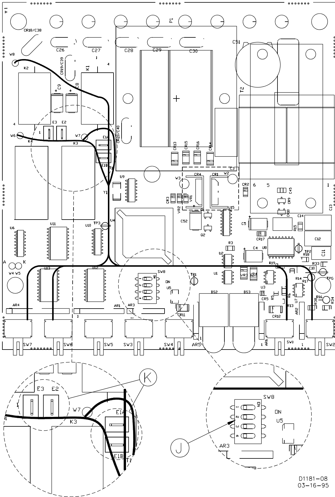
Figure 2-2. BE1-50/51M-222, Location of Controls and Indicators
