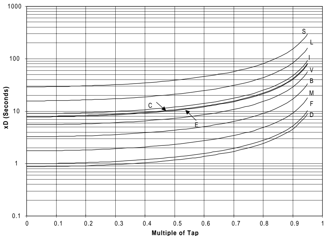
Figure 1-6. Integrating Reset Characteristic Curve
