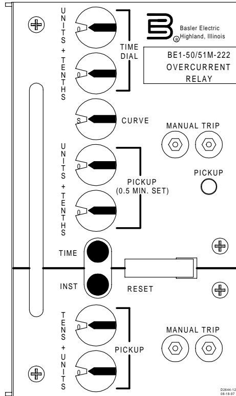
Figure 1-1. BE1-50/51M-222 Overcurrent Relay, C1 Case
