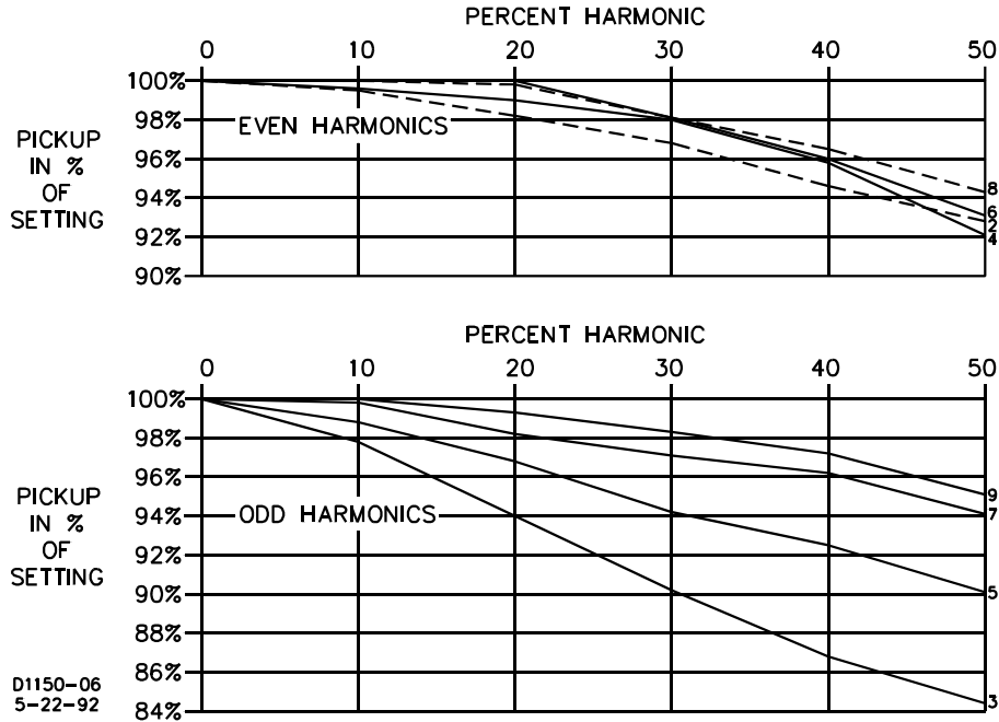
Figure 1-4. Harmonic Response
