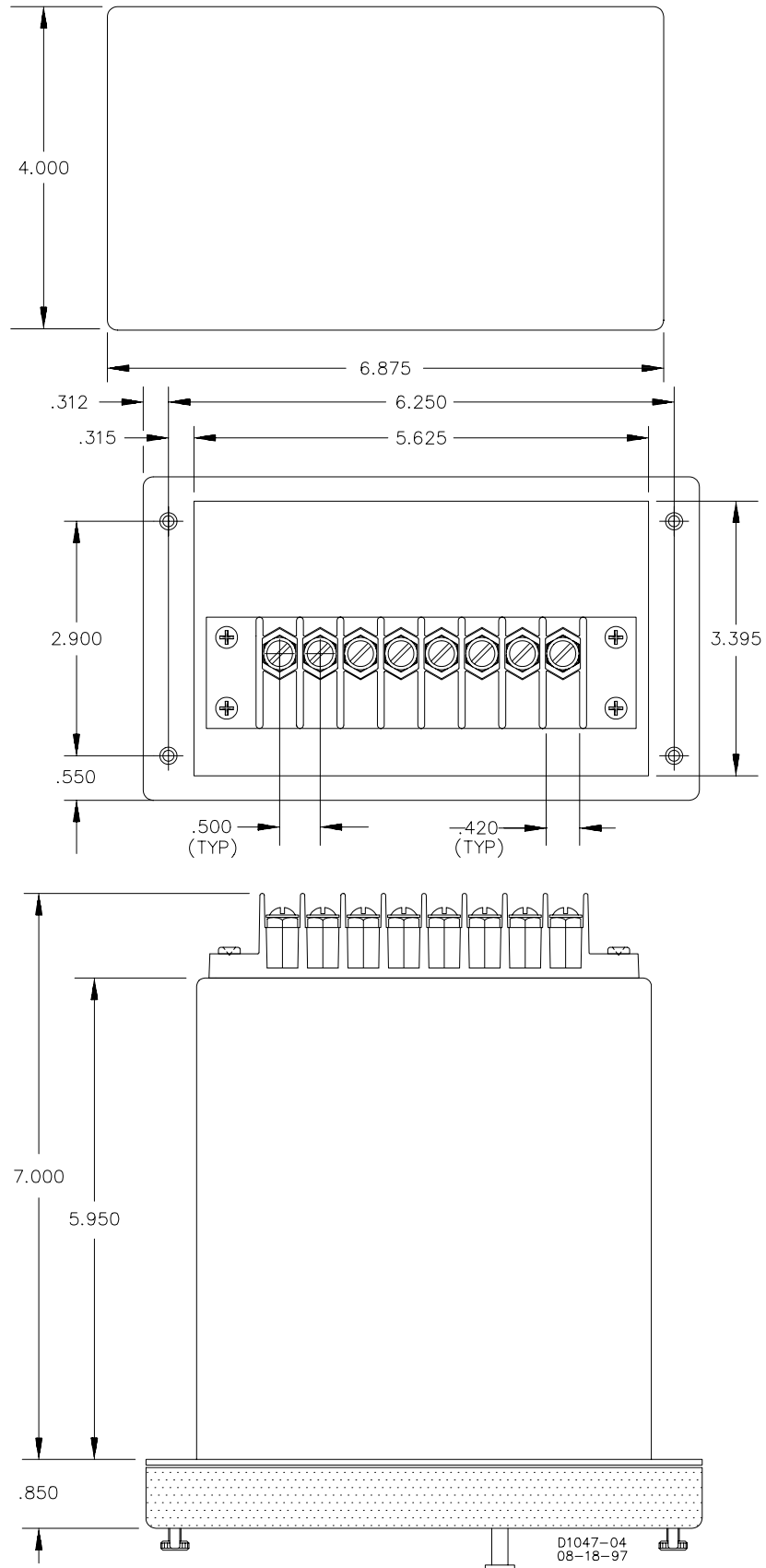
Figure 4-1. Outline Dimensions, C1 Case
