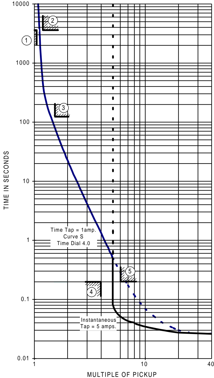
Figure 1-2. Load Demand Characteristic Curve
