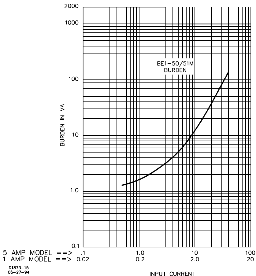
Figure 1-3. Device Burden Characteristics
