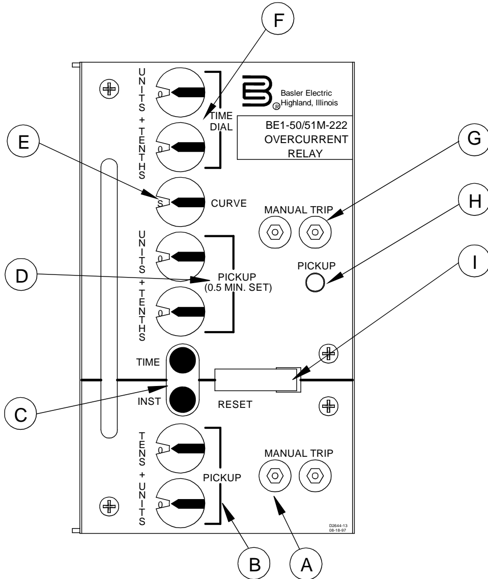
Figure 2-1. BE1-50/51M-222, Location of Controls and Indicators
