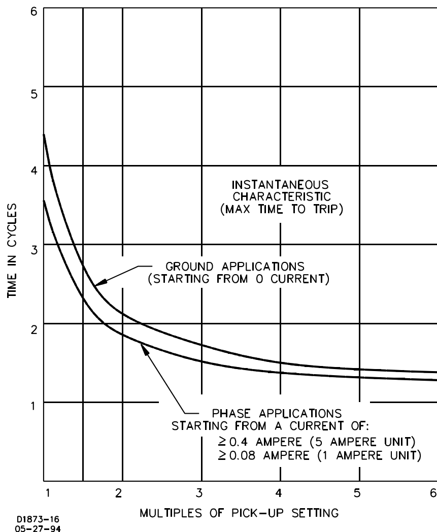
Figure 1-5. Instantaneous Characteristic Curves
