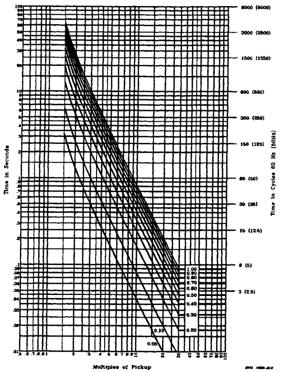
Time Curve C3
