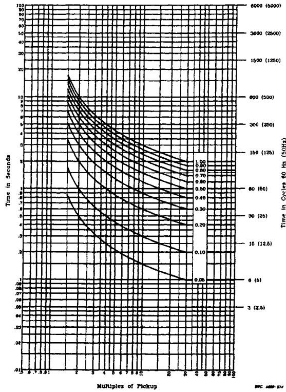
Time Curve C1
