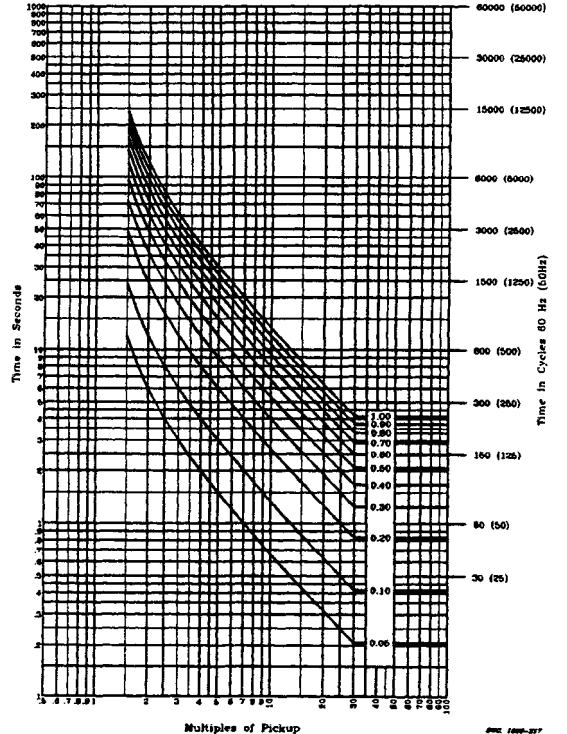
Time Curve C4
