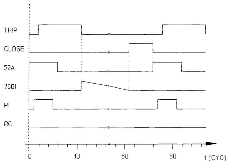
Figure 5.7: Single Shot Unsupervised Reclose Sequence
