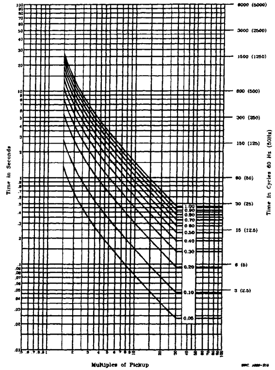
Time Curve C2
