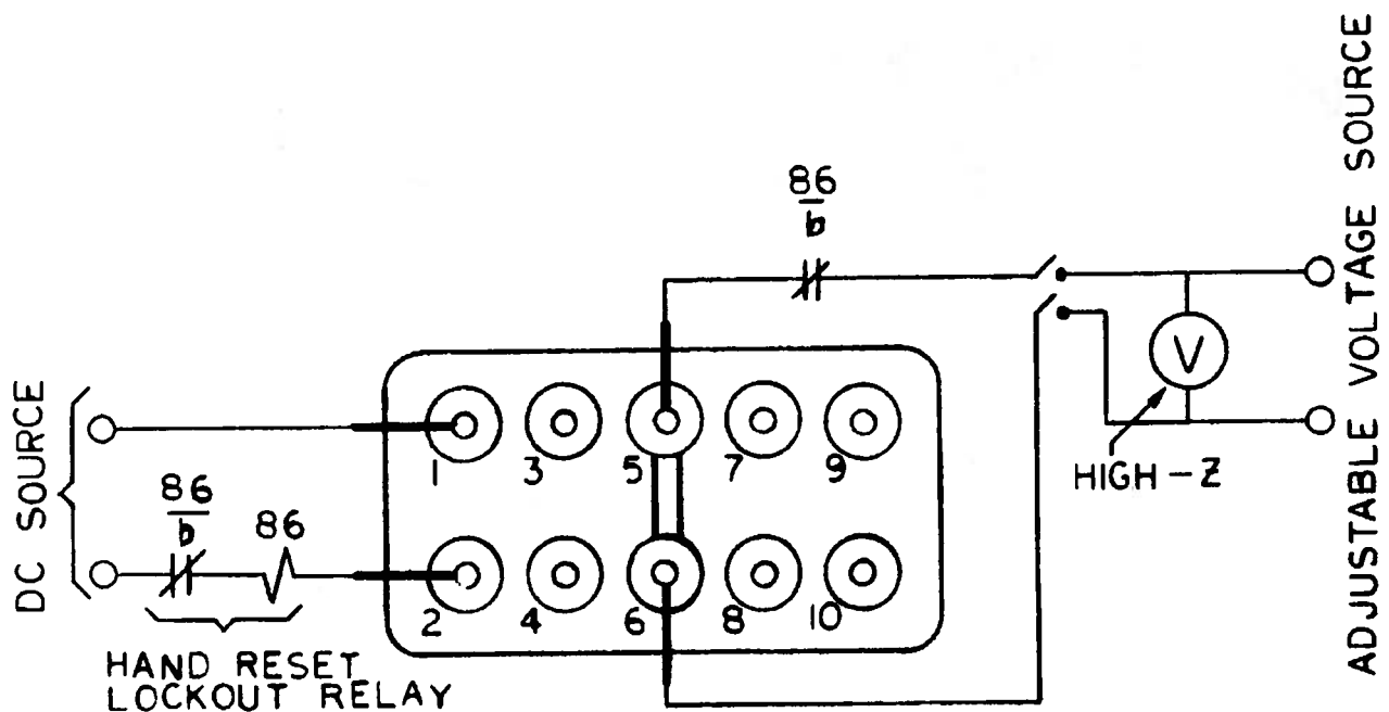
TEST CIRCUIT FOR SETTING 87L
